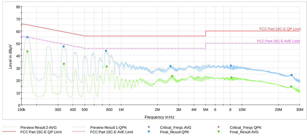
Plot 7-39. AC Line-Conducted Test Plot (L1, GFSK ePA – Ch.39, with AC/DC Adapter + Magnetic Charger)
