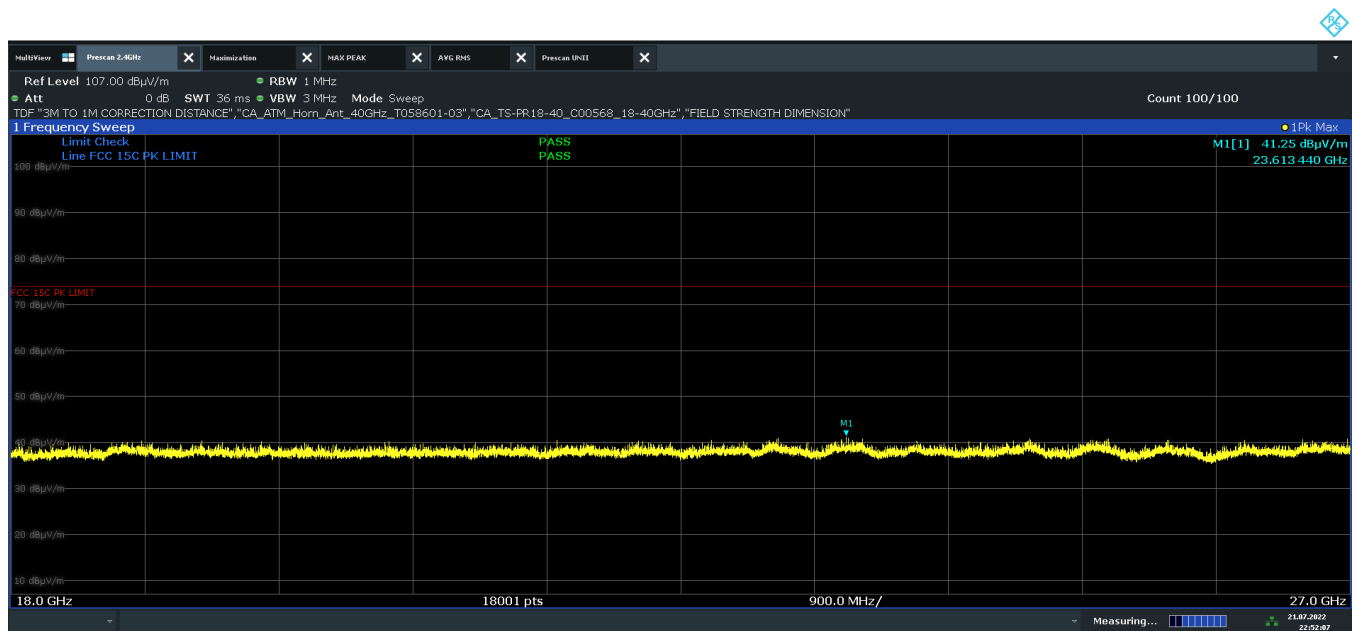
Plot 7-33. Radiated Spurious Emissions above 18GHz (BT GFSK ePA – Ch.39, Pol V)
