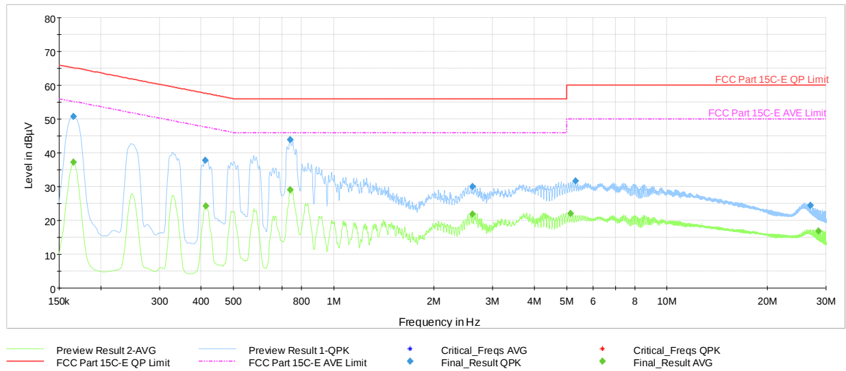
Plot 7-40. AC Line-Conducted Test Plot (N, GFSK ePA – Ch.39, with AC/DC Adapter + Magnetic Charger)
