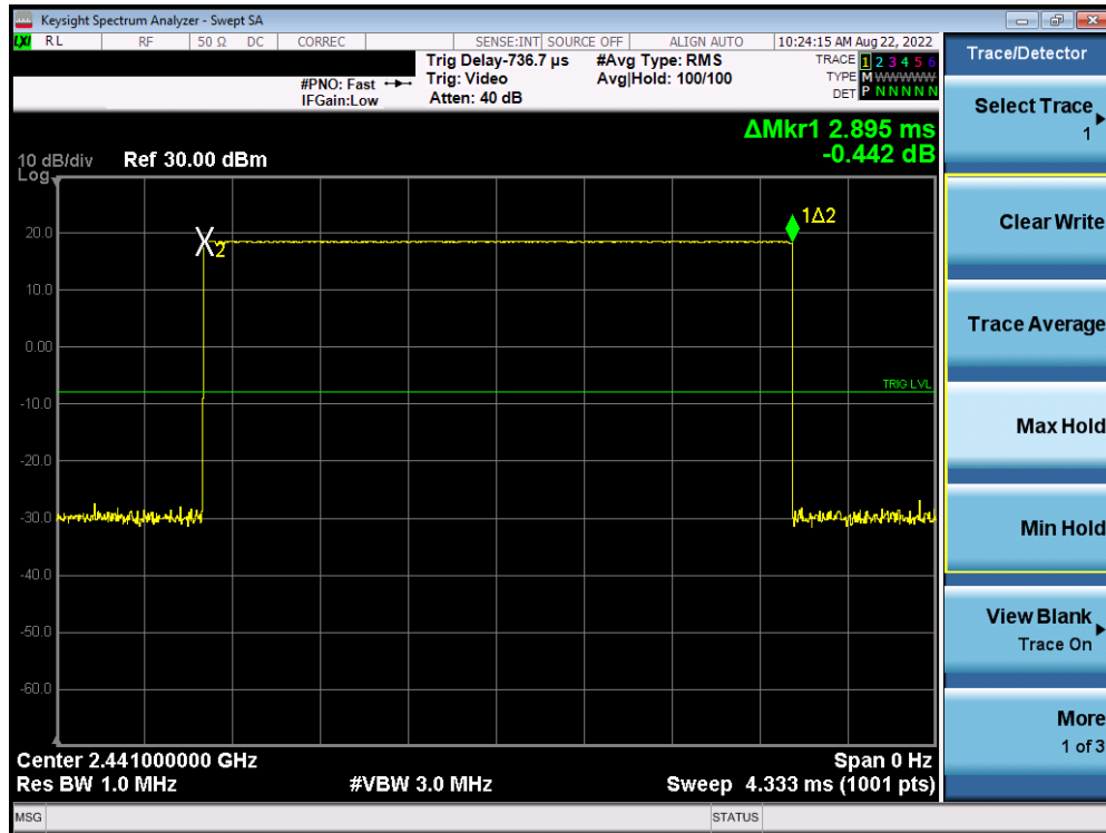
Plot 7-17. Time of Occupancy (Bluetooth, GFSK, ePA)
