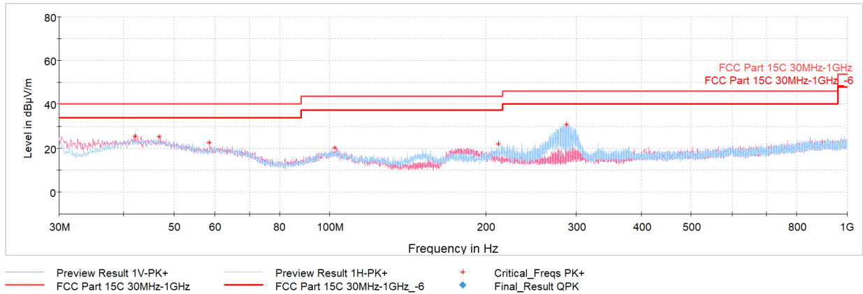
Plot 7-38. Radiated Spurious Emissions Below 1GHz (GFSK ePA – Ch.39, with AC/DC Adapter + Magnetic Charger)
