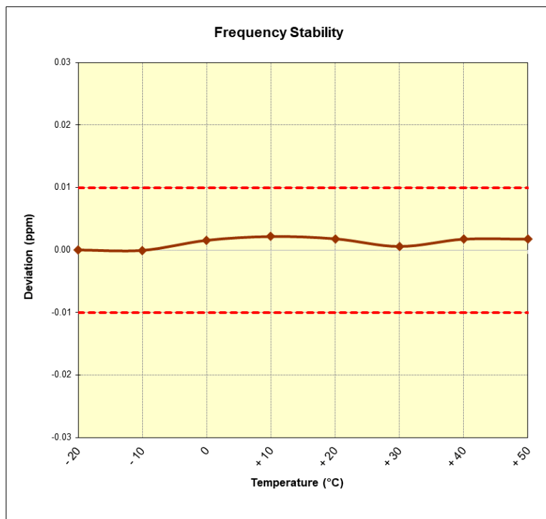
Figure 7-4. Frequency Stability Plot (Reader 100% ASK 1 out of 4)
