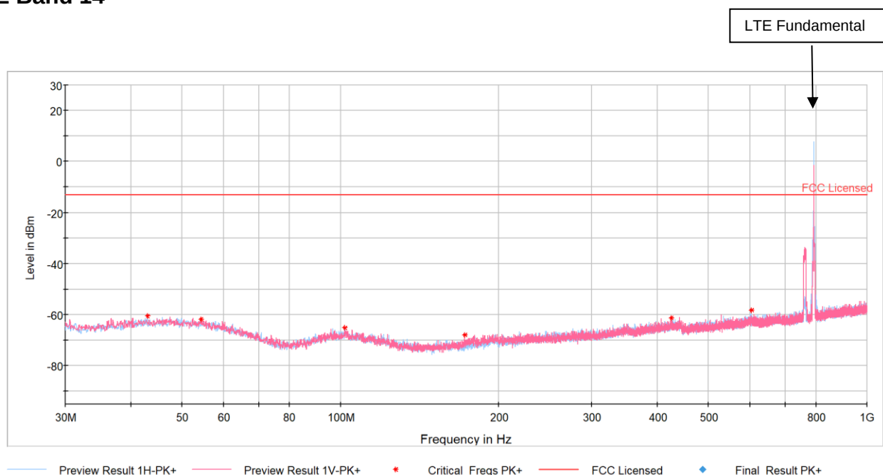
Plot 7-48. Antenna BCM Radiated Spurious Plot below 1GHz (LTE Band 14)
