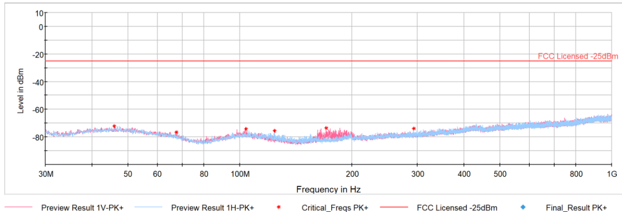
Plot 7-65. Antenna FCM Radiated Spurious Emissions -Simultaneous Transmission 30MHz – 1GHz
