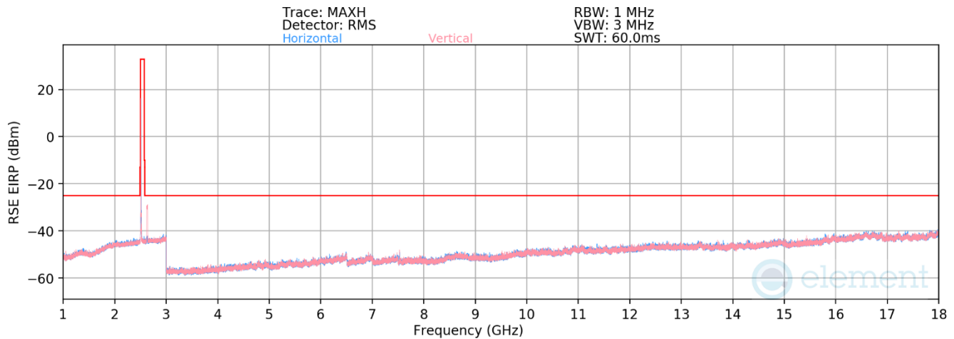
Plot 6-1. Radiated Spurious Emission Above 1GHz (LTE-Band 7)
