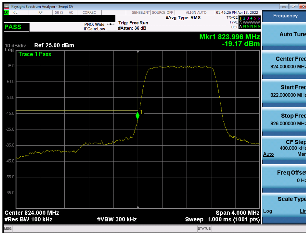
Plot 7-28. Lower BE Plot (LTE Band 5 – 1.4MHz QPSK – Full RB Configuration)
