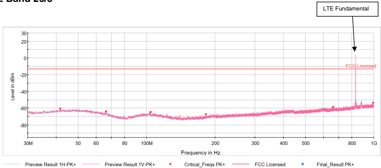
Plot 7-46. Antenna BCM Radiated Spurious Plot below 1GHz (LTE Band 26/5)
