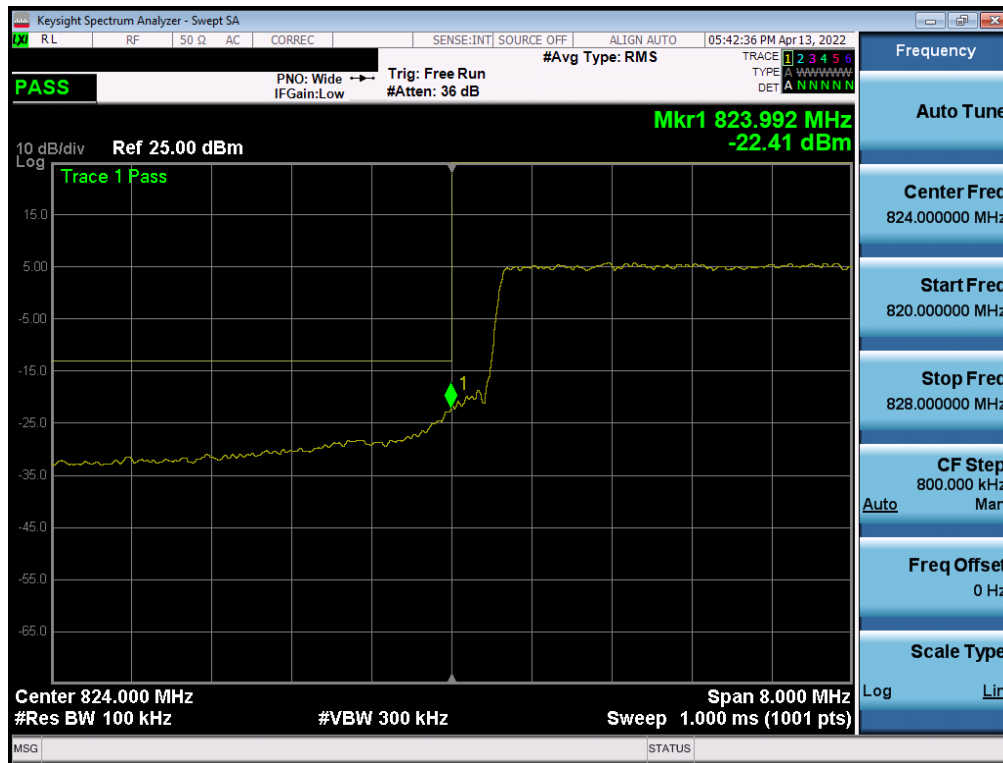
Plot 7-42. Lower BE Plot (LTE Band 26 - 10MHz QPSK - Full RB Configuration)
