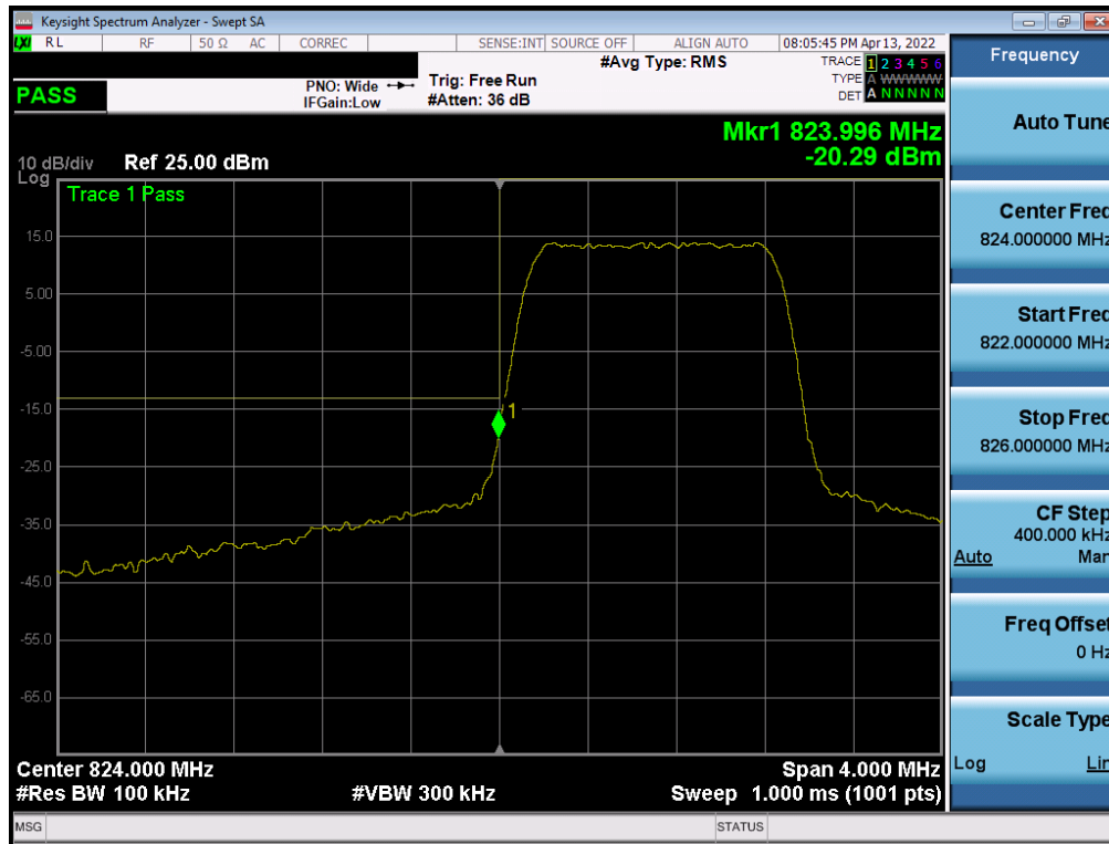
Plot 7-36. Lower BE Plot (LTE Band 26 – 1.4MHz QPSK – Full RB Configuration)
