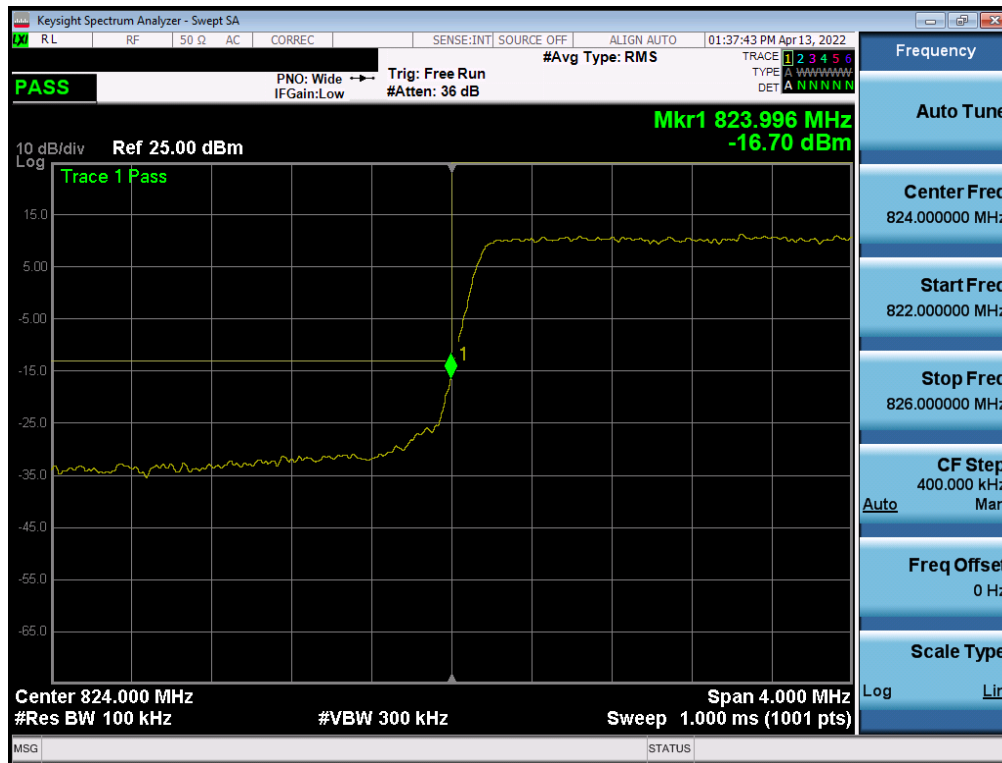
Plot 7-30. Lower BE Plot (LTE Band 5 - 3MHz QPSK - Full RB Configuration)
