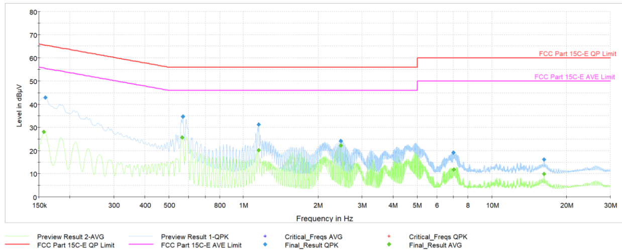
Plot 7-39. AC Line Conducted Plot with Bluetooth LE (L1, 1Mbps ePA – Ch.19 with Laptop Charger + Magnetic Charger)
