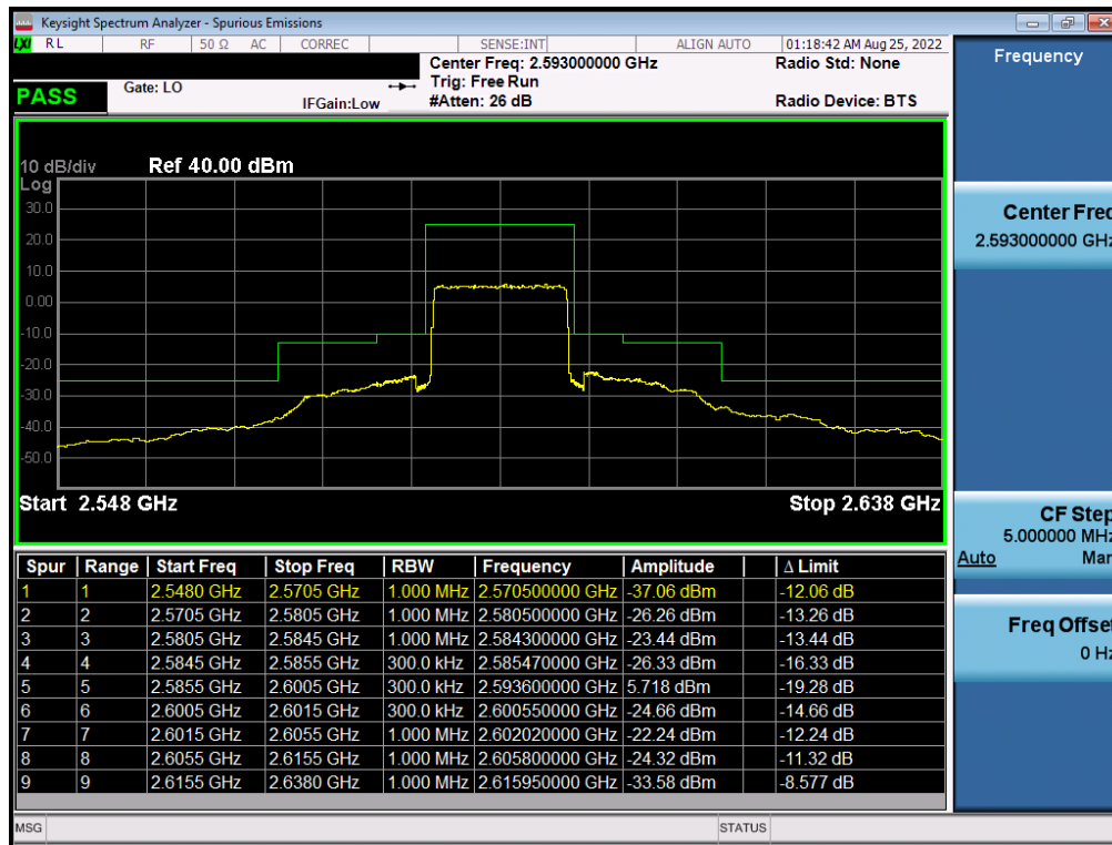
Plot 7-54. Middle ACP Plot (LTE Band 41 - 15MHz QPSK – Full RB)
