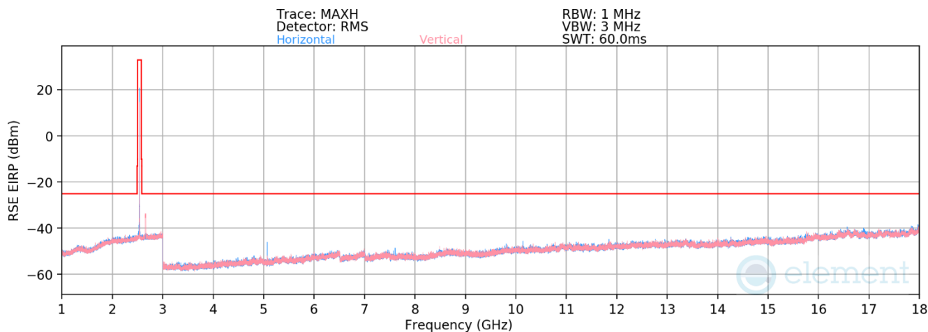
Plot 6-1. Radiated Spurious Emission Above 1GHz (LTE Band 7)
