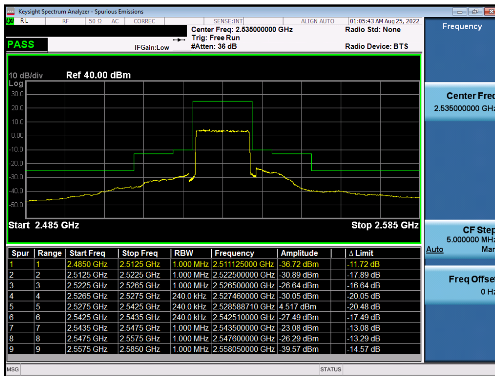
Plot 7-42. Middle ACP Plot (LTE Band 7 - 15MHz QPSK – Full RB)
