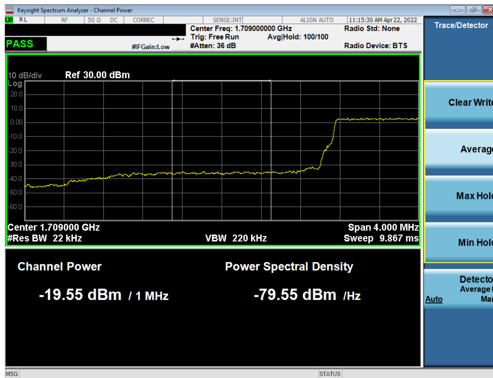
Plot 7-85. Lower Extended Band Edge Plot (LTE Band 4 - 3MHz QPSK – Full RB)
