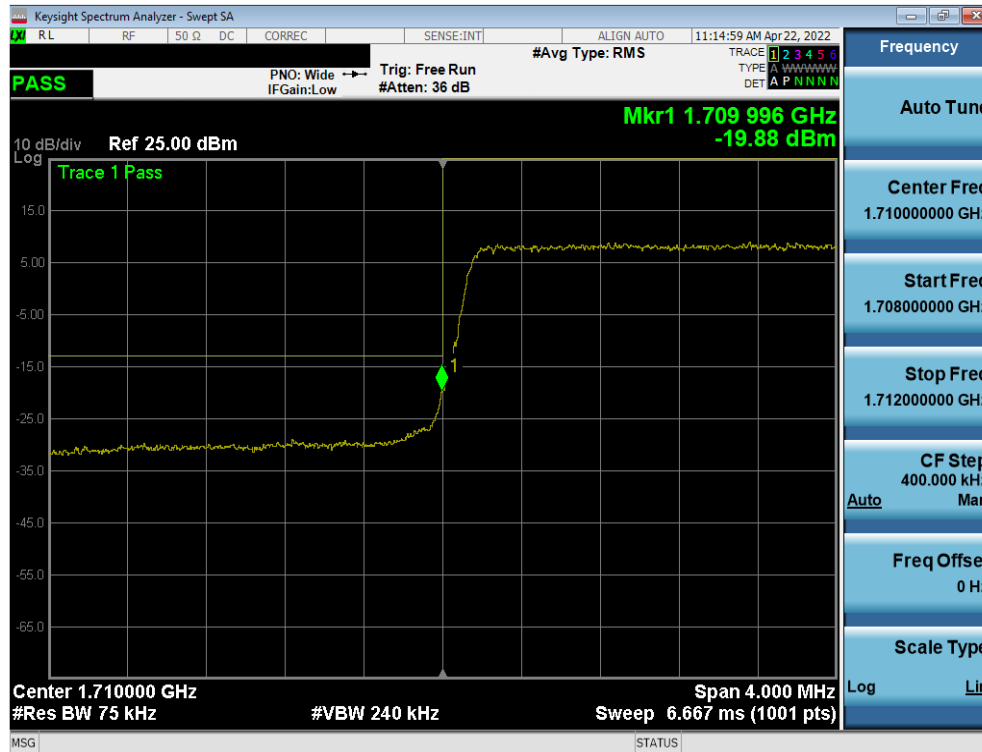
Plot 7-84. Lower Band Edge Plot (LTE Band 4 - 3MHz QPSK – Full RB)
