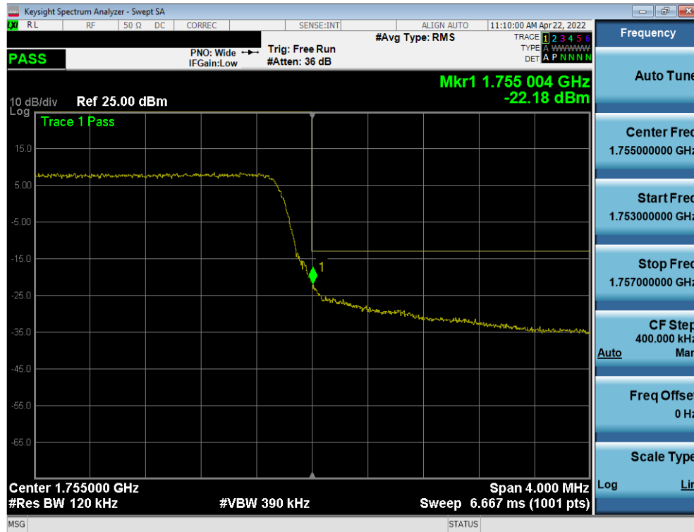
Plot 7-90. Upper Band Edge Plot (LTE Band 4 - 5MHz QPSK – Full RB)
