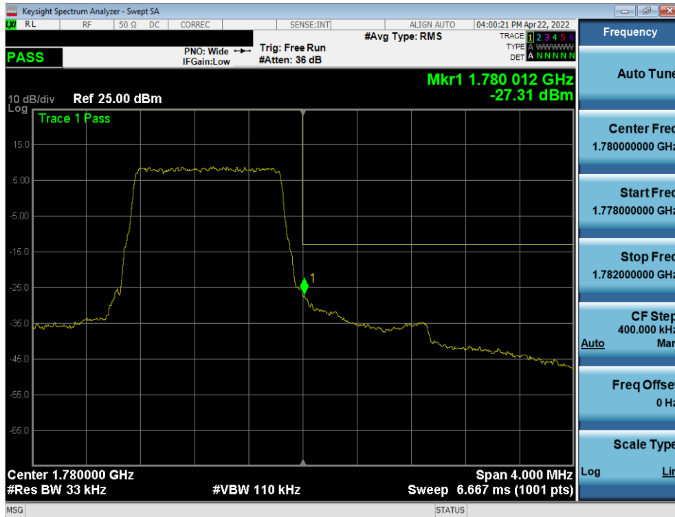
Plot 7-58. Upper Band Edge Plot (LTE Band 66 – 1.4MHz QPSK – Full RB)
