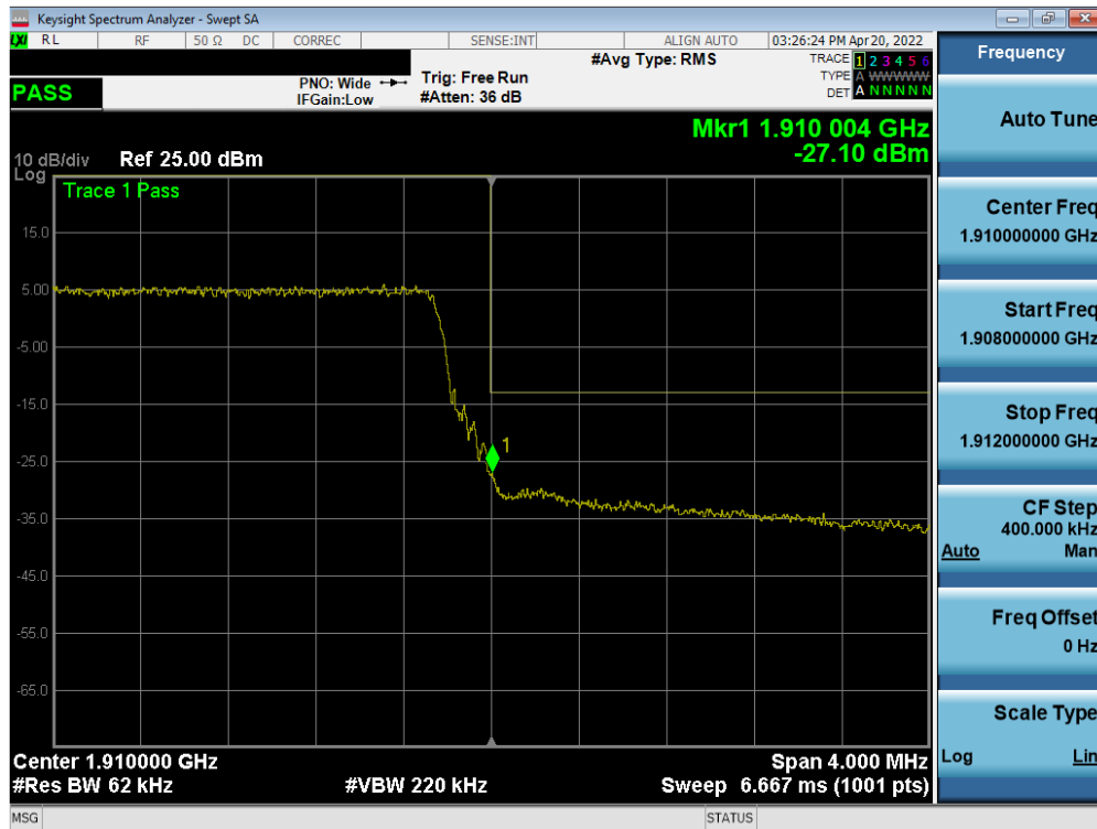
Plot 7-66. Upper Band Edge Plot (LTE Band 2 – 5MHz QPSK – Full RB Configuration)
