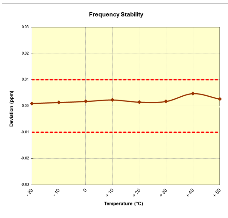
Figure 7-4. Frequency Stability Plot (Reader 100% ASK 1 out of 256)
