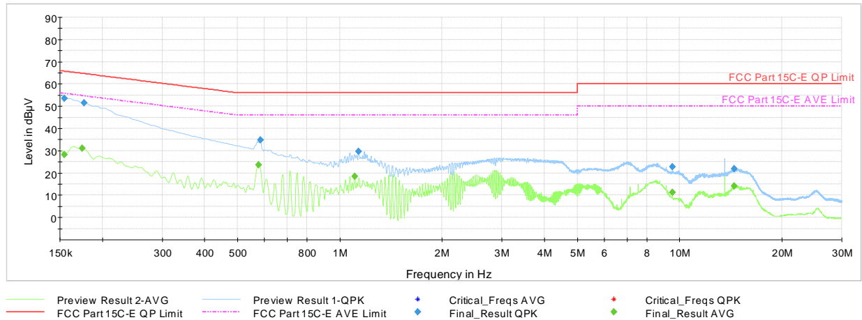
Plot 7-14. AC Line-Conducted Plot (L1, Reader A 848kbps, with AC/DC Adapter and Magnetic Charger)
