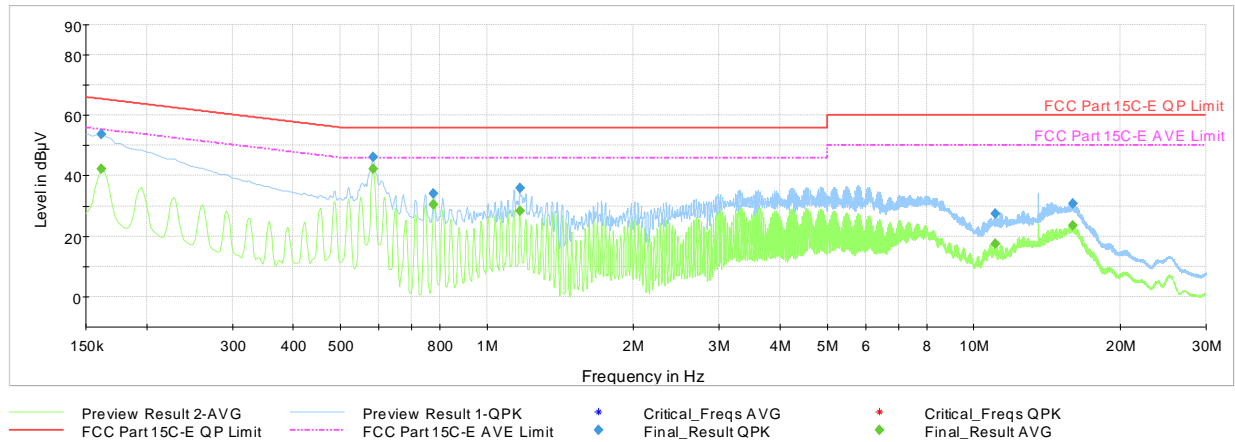
Plot 7-12. AC Line-Conducted Plot (L1, CE F 424kbps, with Laptop and Magnetic Charger)
