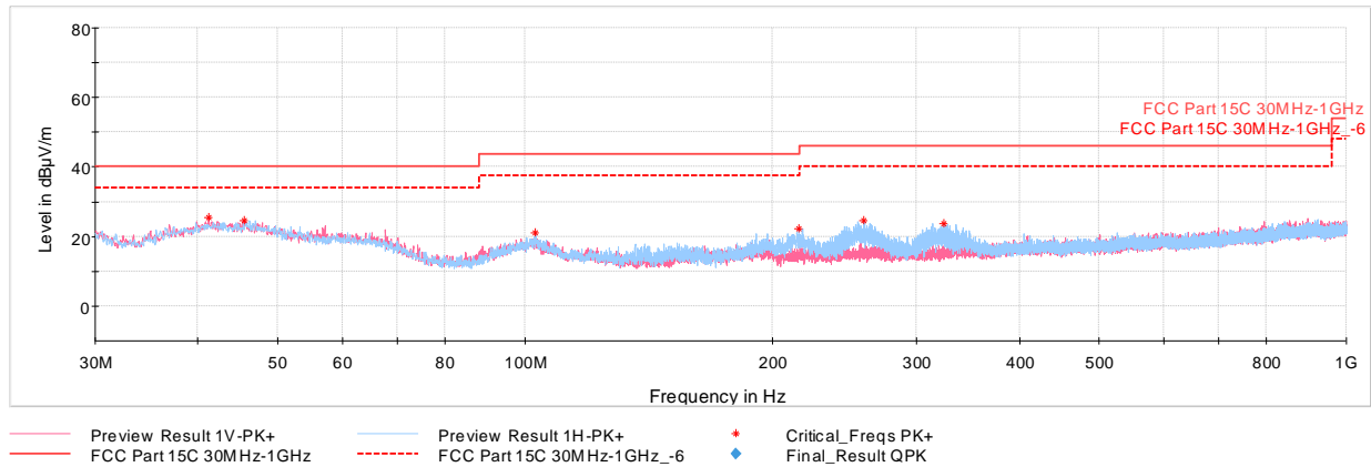
Plot 7-11. Radiated Spurious Emissions 30MHz – 1GHz (Reader A 848kbps, with Laptop and Magnetic Charger)
