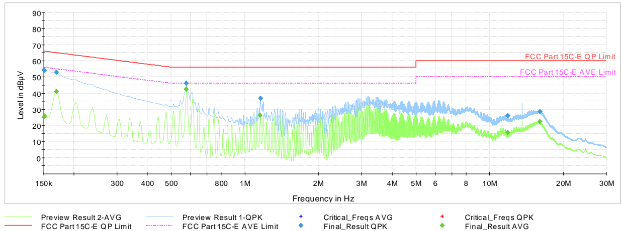
Plot 7-13. AC Line-Conducted Plot (N, CE F 424kbps, with Laptop and Magnetic Charger)
