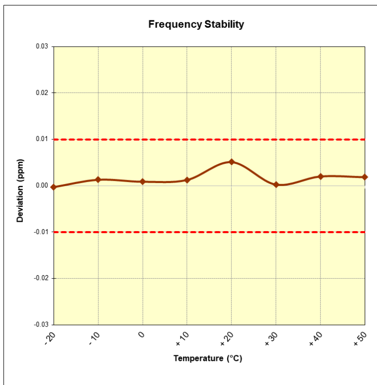
Figure 7-3. Frequency Stability Plot (CE F 424kbps)
