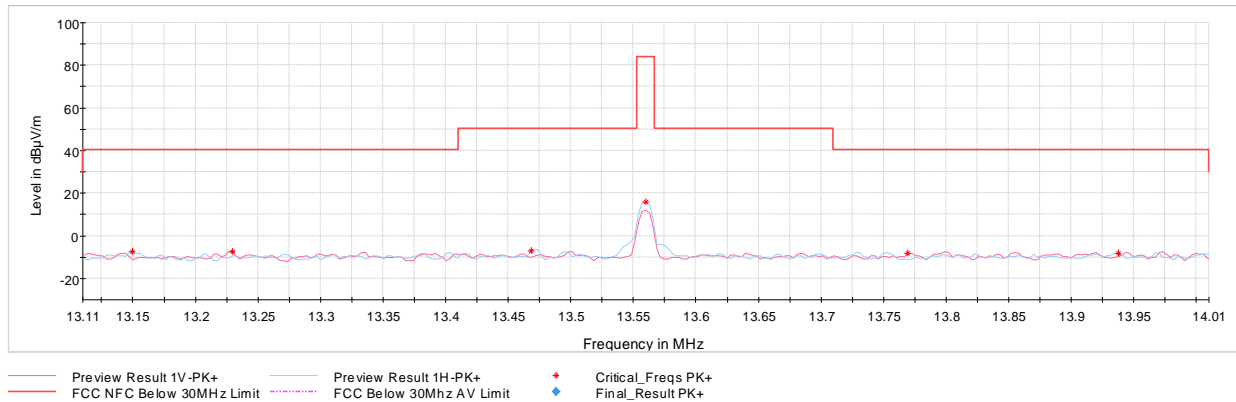
Plot 7-6. In Band Radiated Spurious Emissions (CE F 424kbps, with AC/DC Adapter and Magnetic Charger)
