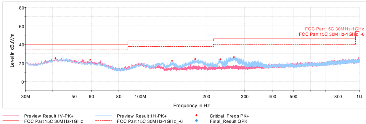
Plot 7-10. Radiated Spurious Emissions 30MHz – 1GHz (CE F 424kbps, with Laptop and Magnetic Charger)
