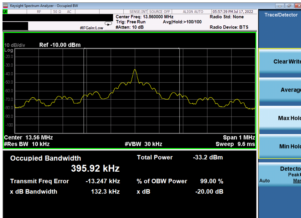
Plot 7-5. 20dB and 99% Bandwidth Plot (Reader 100% ASK 1 out of 256)
