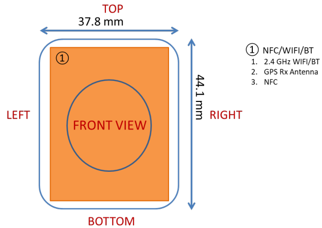
Figure E-1 DUT Antenna Locations
