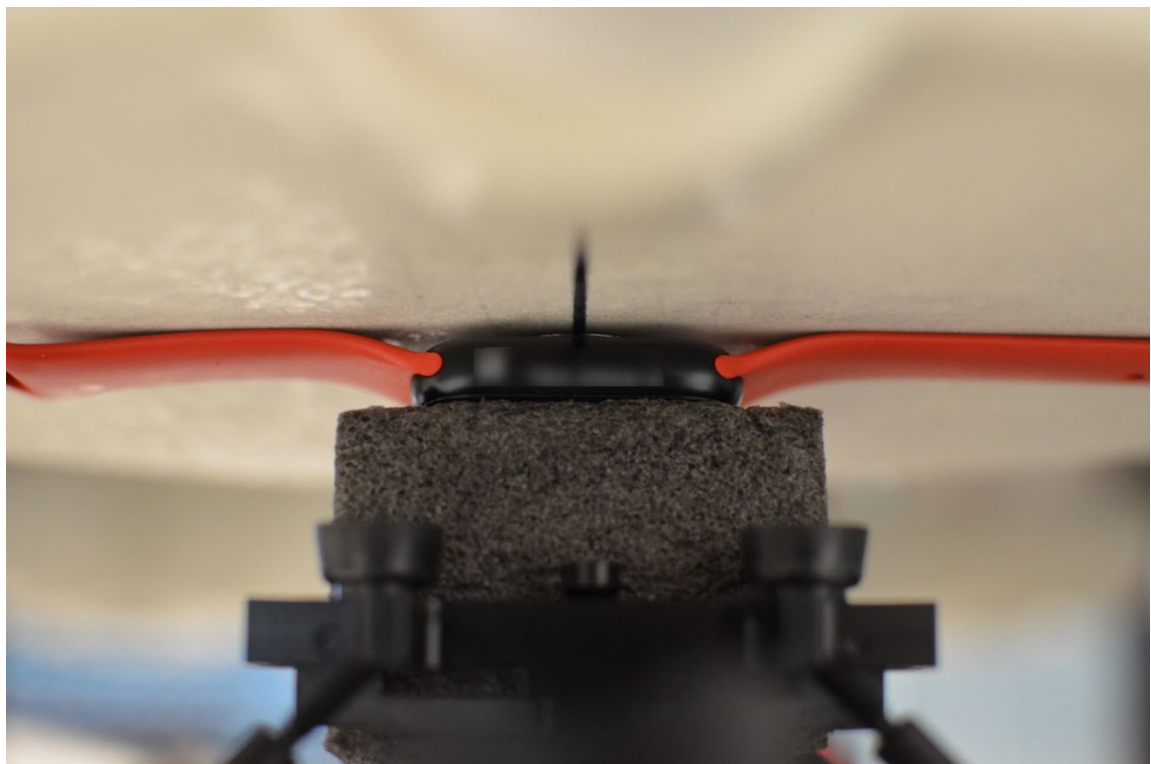
SAR Test Setup Photo 4: Aluminum with Sport Wristband, Extremity, Back Side at 0.0 mm
