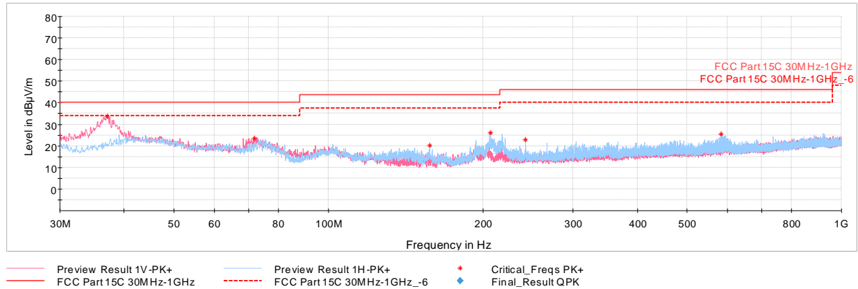
Plot 7-38. Radiated Spurious Emissions Below 1GHz (GFSK ePA – Ch.78, with AC/DC Adapter via USB cable with Magnetic Charger)
