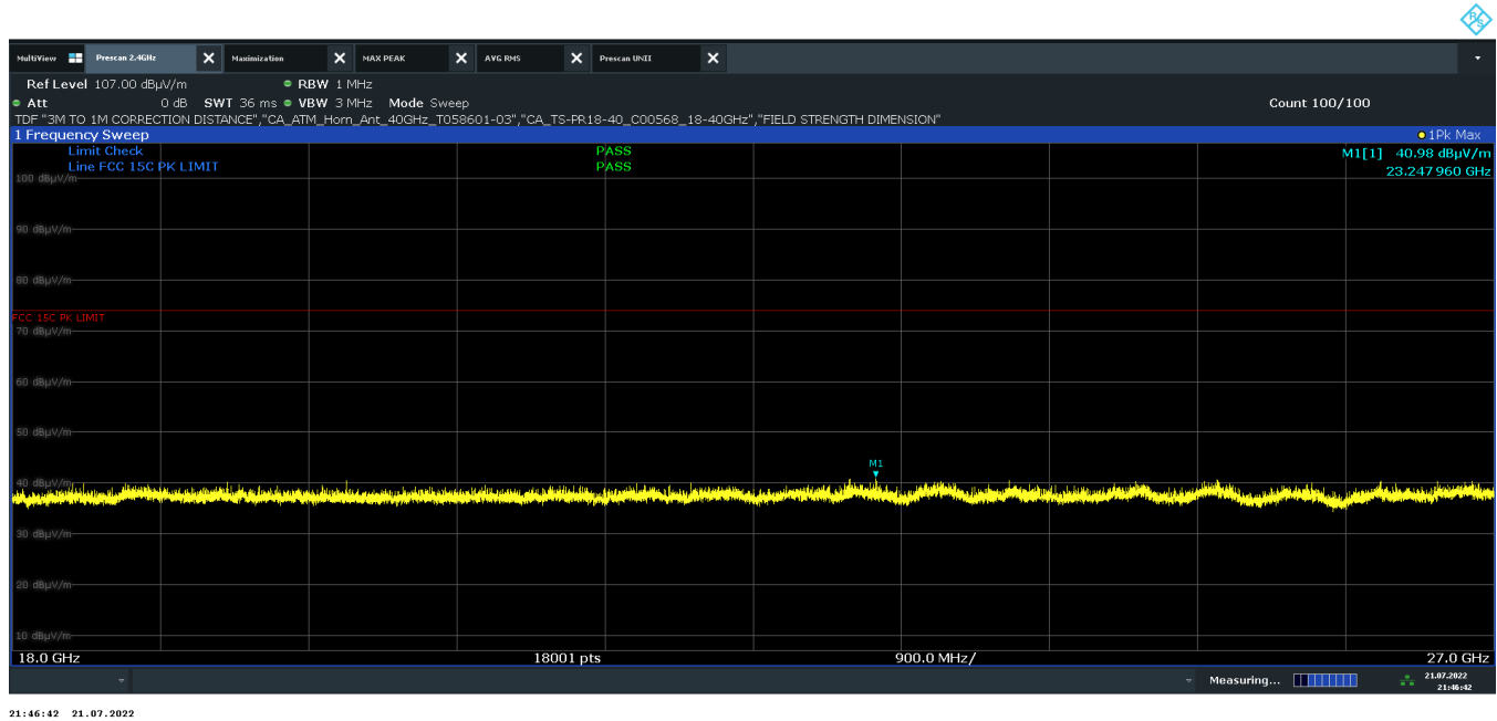
Plot 7-32. Radiated Spurious Emissions above 18GHz (BT GFSK – Ch.78, Pol. H)
