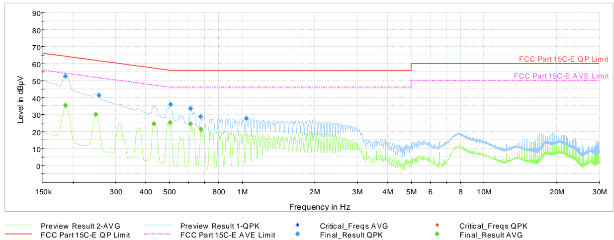
Plot 7-40. AC Line-Conducted Test Plot (N, GFSK ePA – Ch.78, with Laptop via USB cable with Magnetic Charger)
