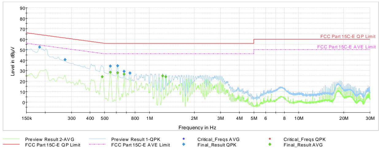
Plot 7-39. AC Line-Conducted Test Plot (L1, GFSK ePA – Ch.78, with Laptop via USB cable with Magnetic Charger)
