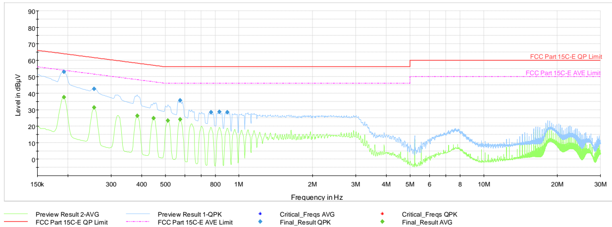
Plot 7-79. AC Line Conducted Plot 802.11b Ch.6 (L1, with Laptop + Magnetic Charger)
