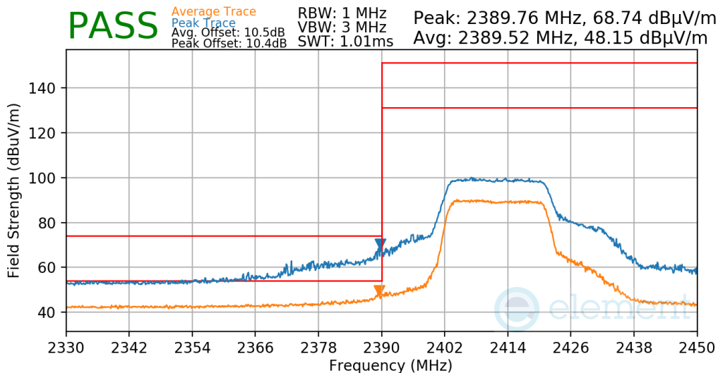
Plot 7-72. Radiated Restricted Lower Band Edge Measurement
