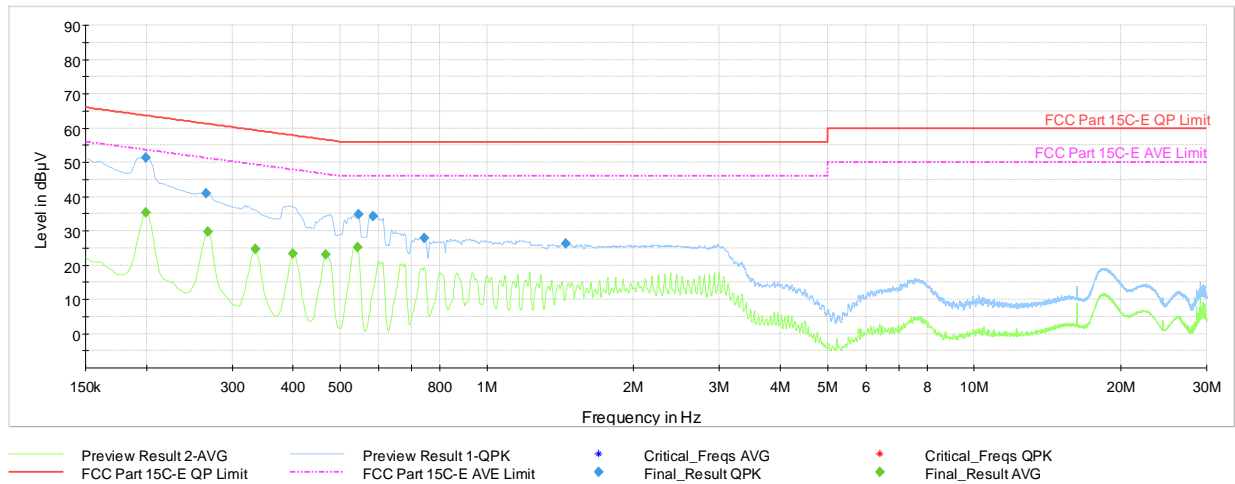
Plot 7-80. AC Line Conducted Plot 802.11b Ch.6 (N, with Laptop + Magnetic Charger)
