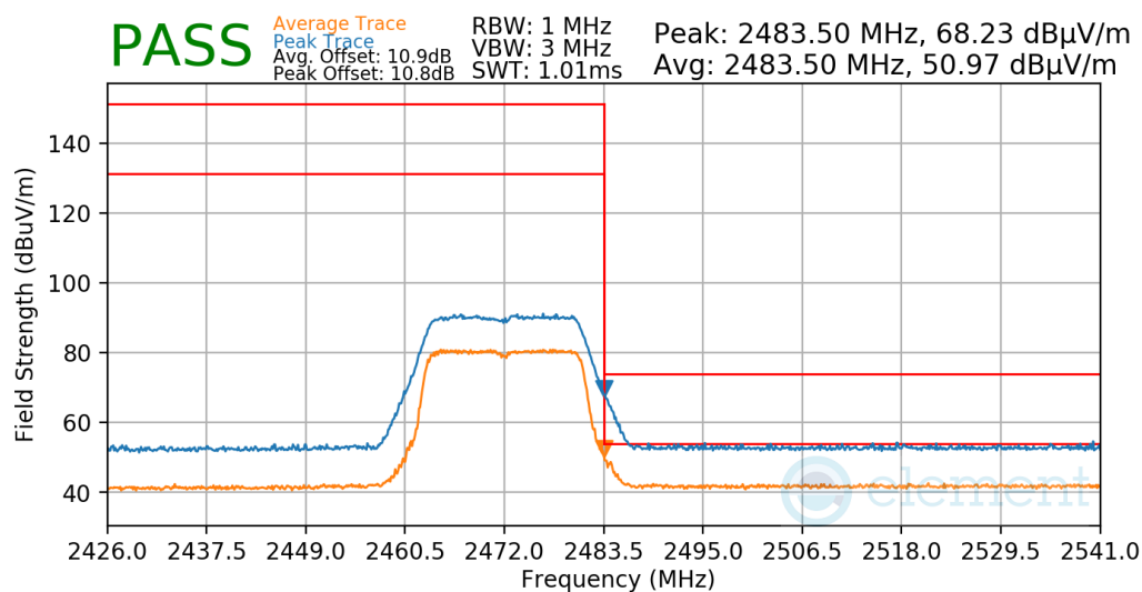
Plot 7-77. Radiated Restricted Upper Band Edge Measurement
