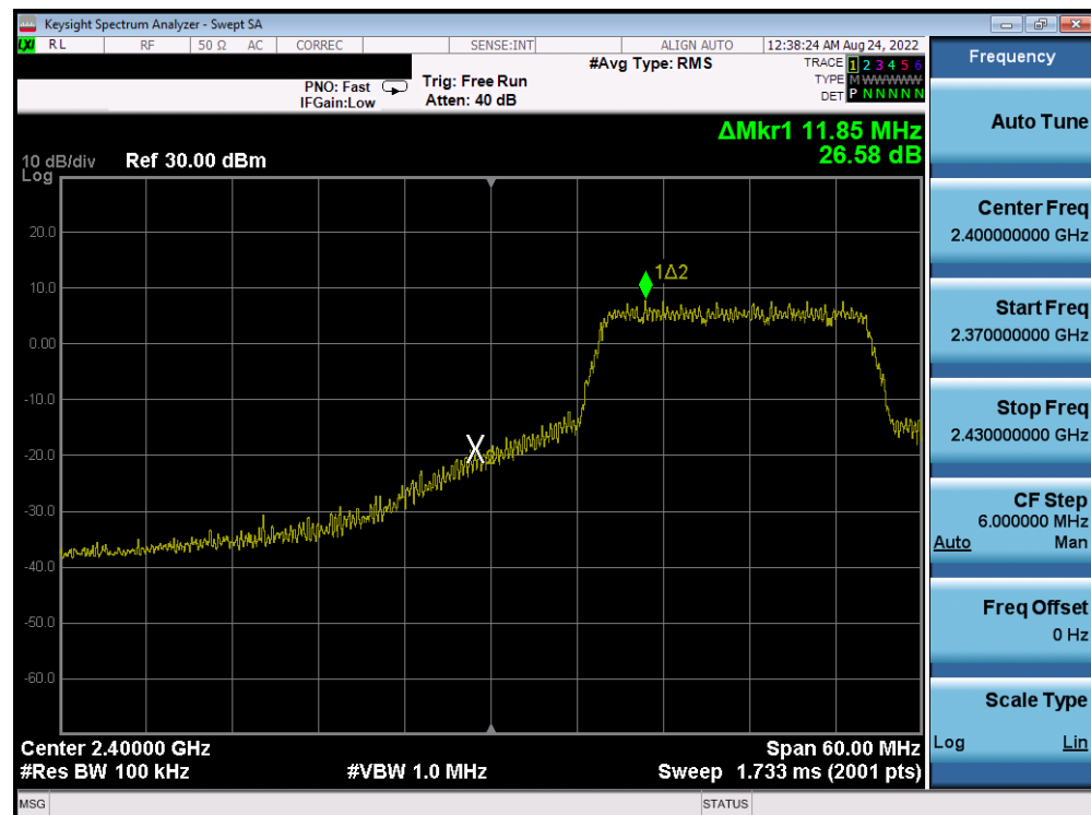
Plot 7-44. Band Edge Plot (802.11n (2.4GHz) – Ch. 2) – MCS7
