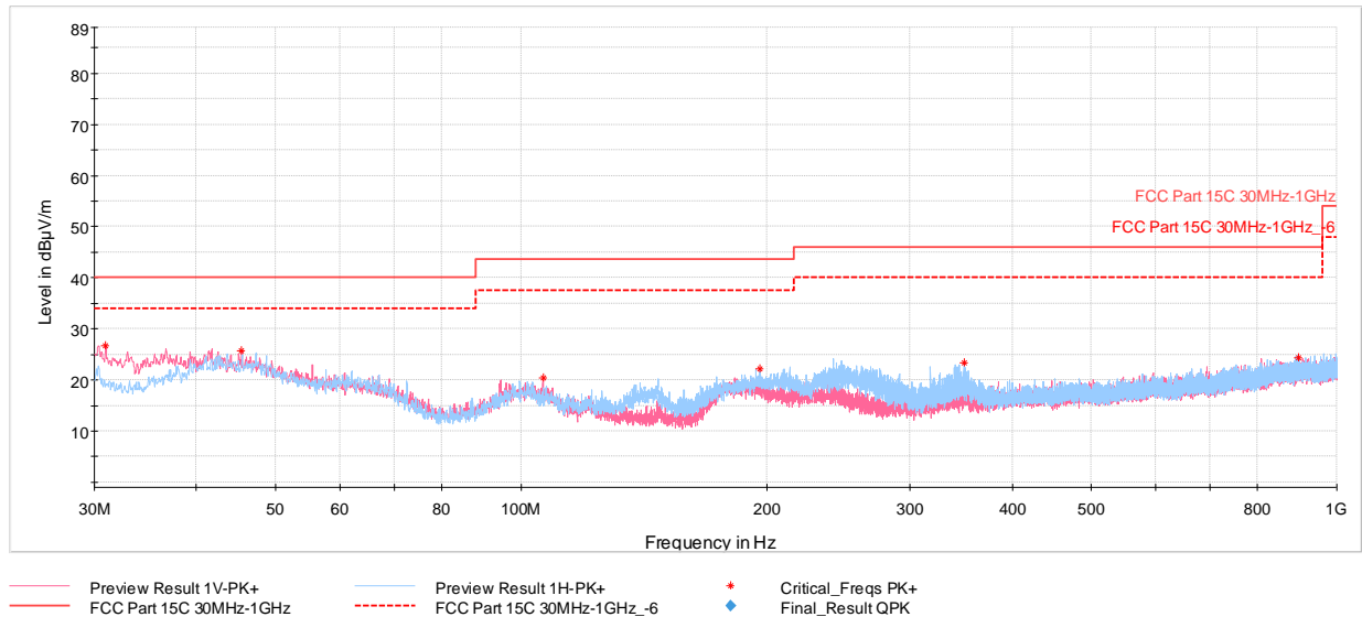
Plot 7-78. Radiated Spurious Emissions 30MHz - 1GHz (802.11b - Ch.6), with AC/DC Adapter + Magnetic Charger
