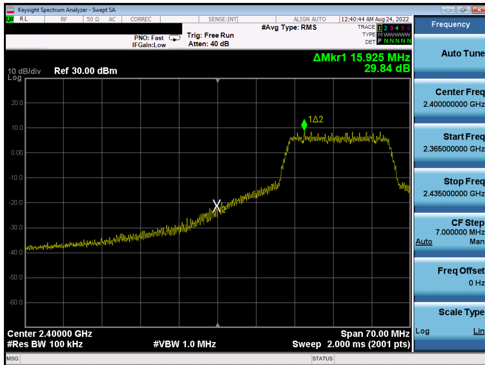
Plot 7-45. Band Edge Plot (802.11n (2.4GHz) – Ch. 3) – MCS7
