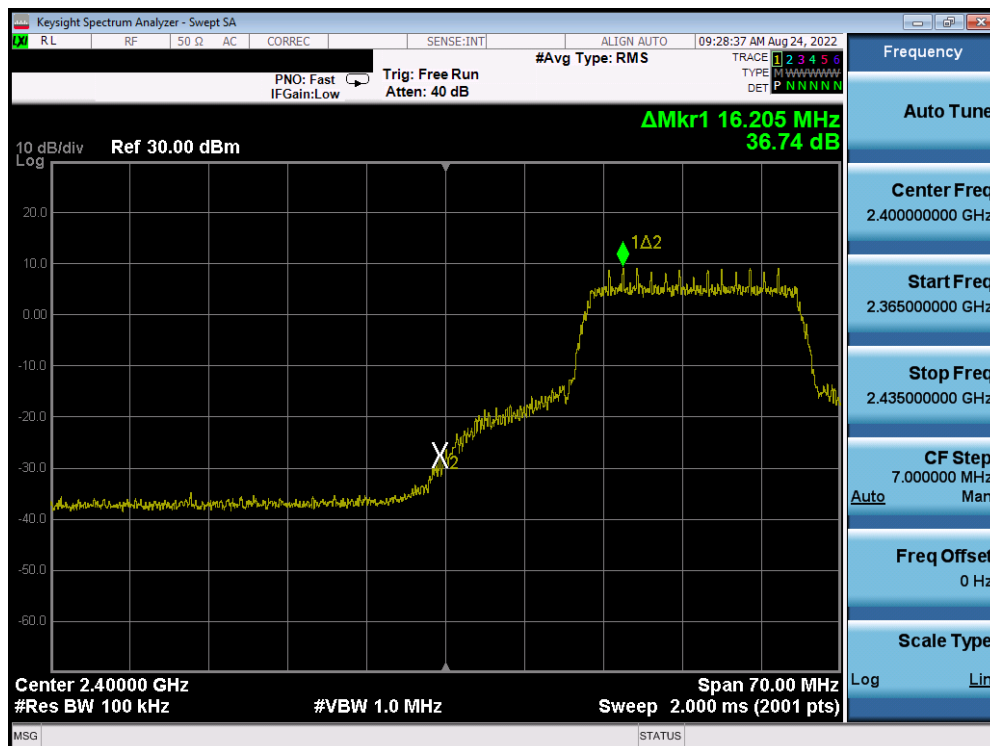
Plot 7-38. Band Edge Plot (802.11n (2.4GHz) – Ch. 3) – MCS0
