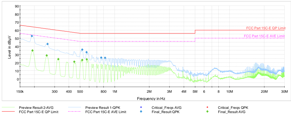
Plot 7-40. AC Line Conducted Plot with Bluetooth LE (N, 1Mbps ePA – Ch.19, with Laptop via USB cable with Magnetic Charger)
