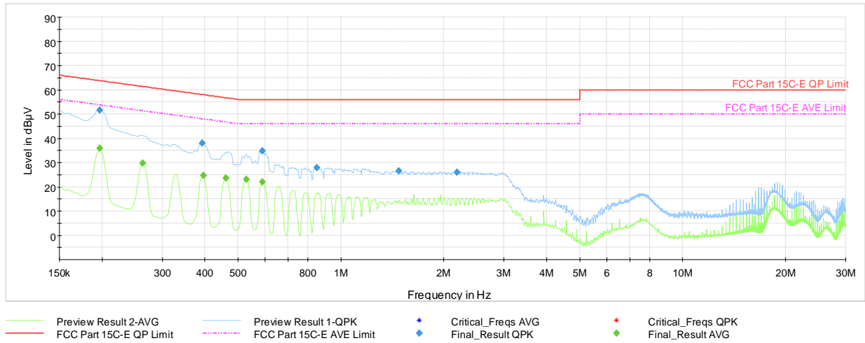
Plot 7-39. AC Line Conducted Plot with Bluetooth LE (L1, 1Mbps ePA – Ch.19 with Laptop via USB cable with Magnetic Charger)
