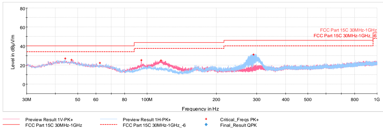
Plot 7-38. Radiated Spurious Emissions Below 1GHz (1Mbps, ePA – Ch. 19, Pol. H & V, with Laptop via USB cable with Magnetic Charger)
