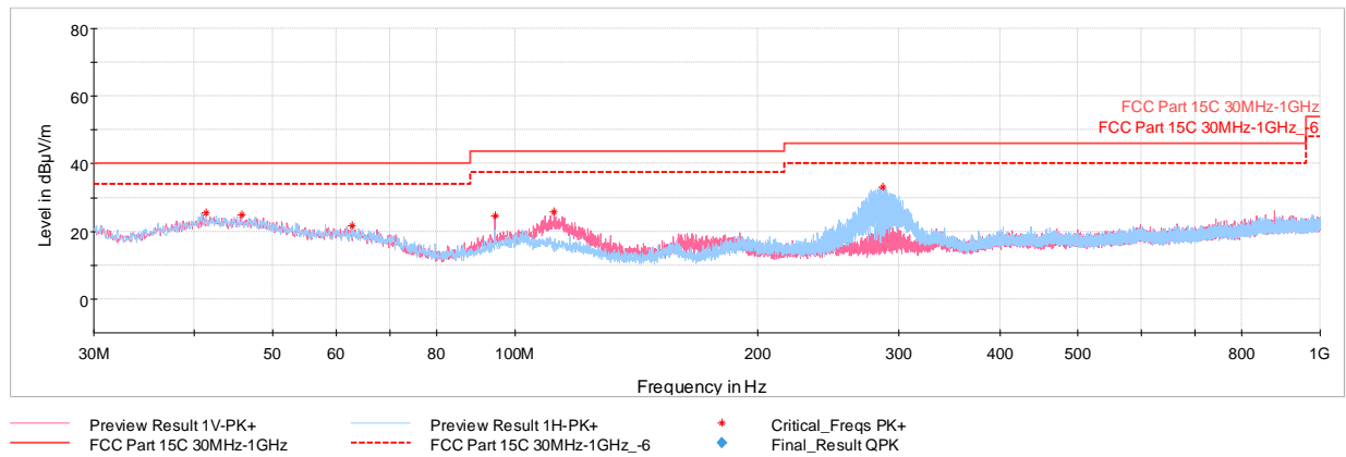
Plot 7-38. Radiated Spurious Emissions Below 1GHz (4Mbps, ePA – Ch.38 with Laptop via USB cable with Magnetic Charger)
