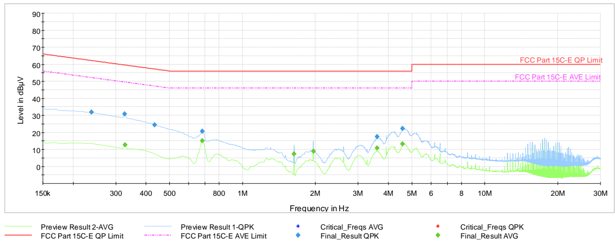
Plot 7-39. AC Line Conducted Plot with Bluetooth HDR (L1, 4Mbps ePA - Ch.38 with Laptop via USB cable with Magnetic Charger)
