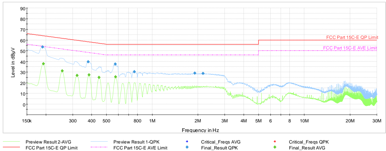
Plot 7-40. AC Line Conducted Plot with Bluetooth HDR (N, 4Mbps ePA - Ch.38 with Laptop via USB cable with Magnetic Charger)
