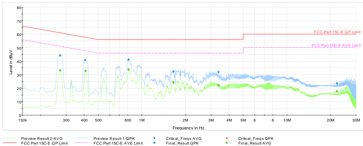
Plot 7-40. AC Line Conducted Plot with Bluetooth HDR (N, 4Mbps ePA - Ch.75 with AC/DC Adapter + Magnetic Charger)
