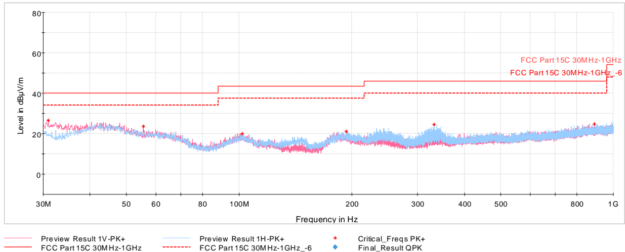
Plot 7-38. Radiated Spurious Emissions Below 1GHz (4Mbps, ePA – Ch.75 with AC/DC Adapter + Magnetic Charger)
