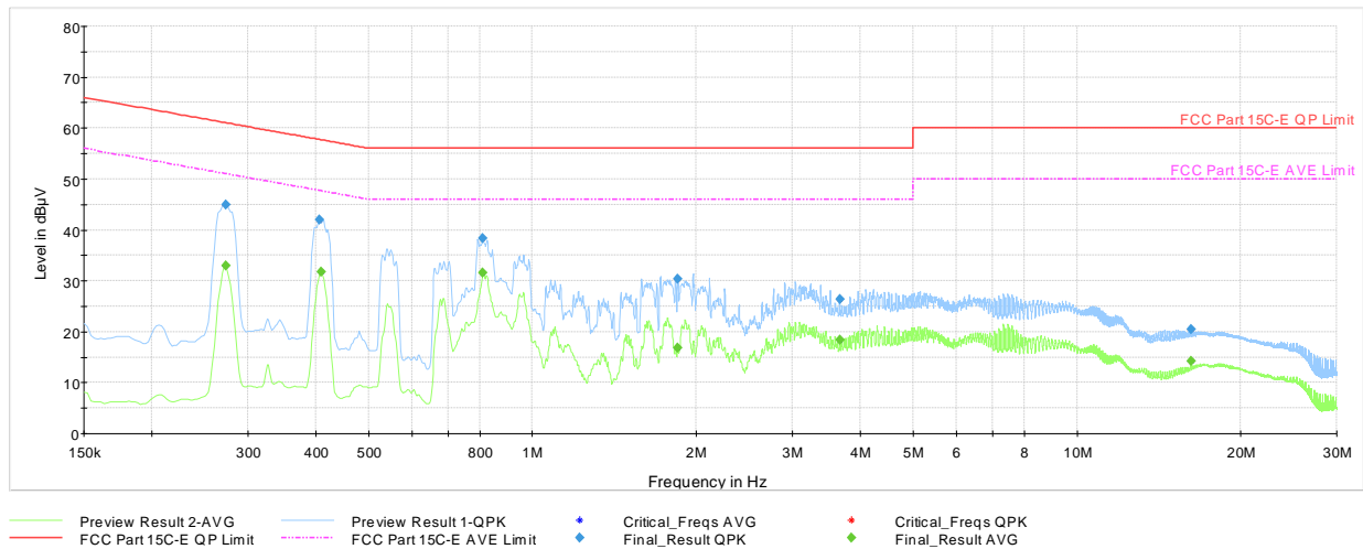
Plot 7-39. AC Line Conducted Plot with Bluetooth HDR (L1, 4Mbps ePA - Ch.75 with AC/DC Adapter + Magnetic Charger)
