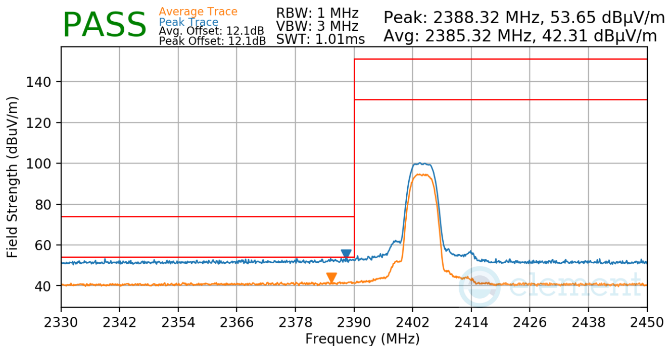
Plot 7-325. Radiated Restricted Lower Band Edge Measurement
