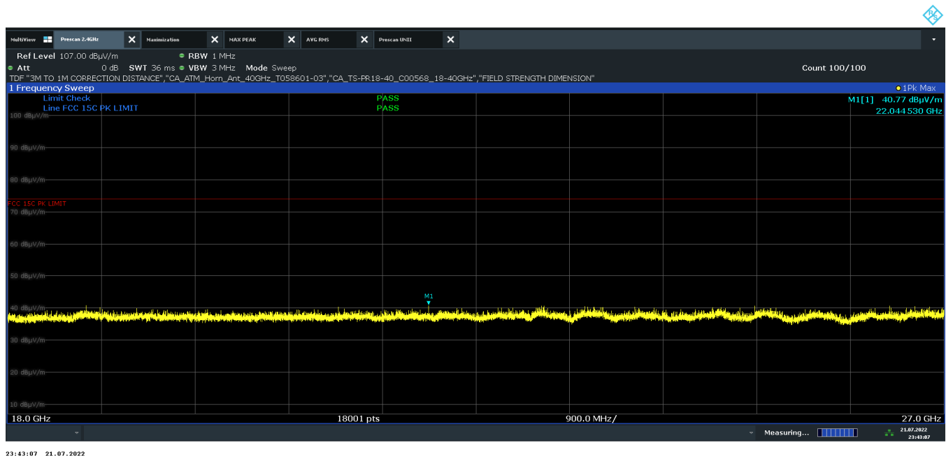
Plot 7-32. Radiated Spurious Plot Above 18GHz (4Mbps, HDR4, ePA – Ch.75, Ant. Pol.H)
