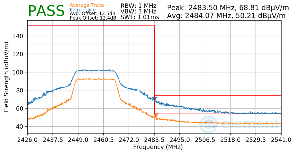
Plot 7-71. Radiated Restricted Upper Band Edge Measurement
