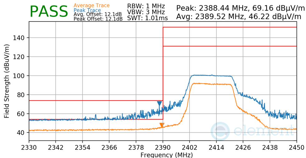
Plot 7-62. Radiated Restricted Lower Band Edge Measurement
