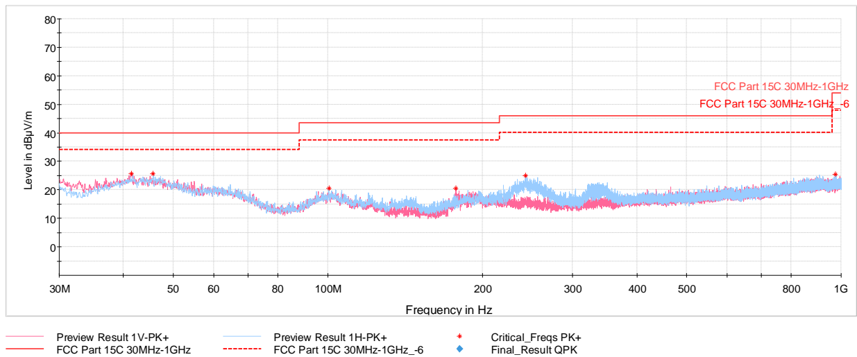
Plot 7-75. Radiated Spurious Emissions below 1GHz (802.11b - Ch.6, with AC/DC Adapter via USB-C cable with Magnetic Charger)
