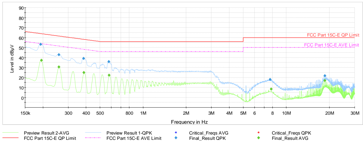
Plot 7-76. AC Line Conducted Plot 11b Ch.6 (L1, with Laptop via USB-C cable with Magnetic Charger)
