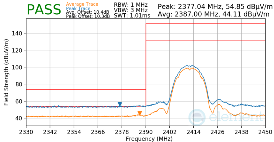
Plot 7-59. Radiated Restricted Lower Band Edge Measurement
