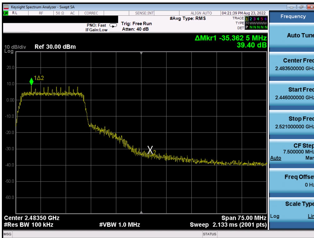
Plot 7-38. Band Edge Plot (802.11n MCS0 – Ch. 10)
