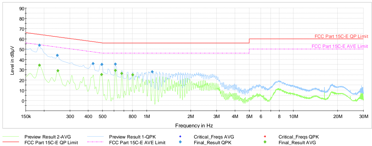
Plot 7-77. AC Line Conducted Plot 11b Ch.6 (N, with Laptop via USB-C cable with Magnetic Charger)
