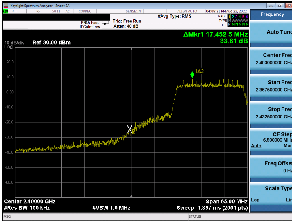
Plot 7-37. Band Edge Plot (802.11n MCS0 – Ch. 3)
