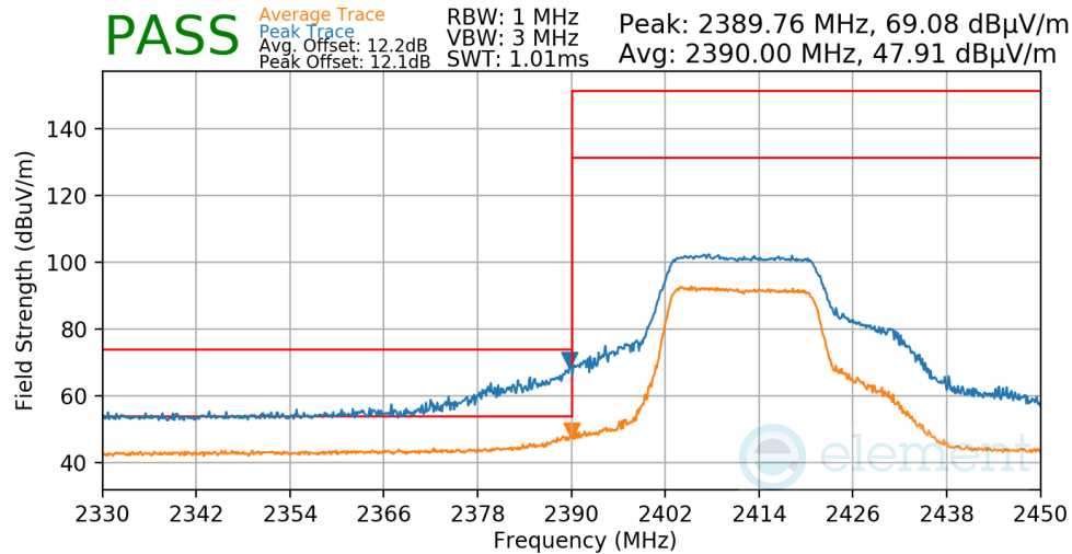
Plot 7-69. Radiated Restricted Lower Band Edge Measurement
