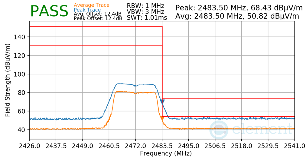
Plot 7-68. Radiated Restricted Upper Band Edge Measurement
