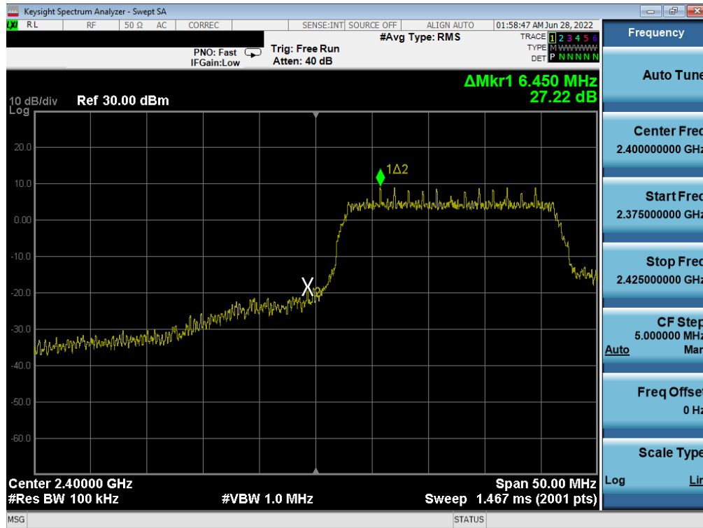
Plot 7-35. Band Edge Plot (802.11n MCS0 – Ch. 1)
