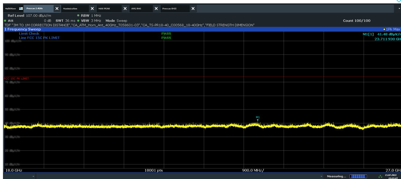
Plot 7-58. Radiated Spurious Emissions above 18GHz (802.11b – Ch16, Pol V)
