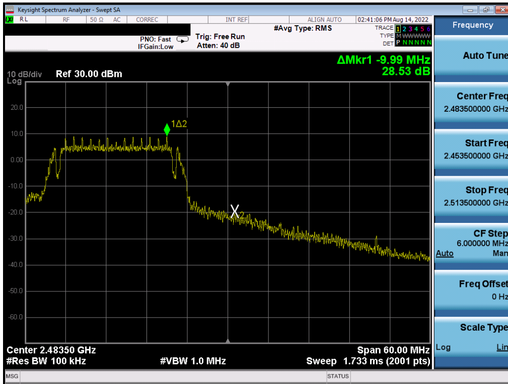
Plot 7-33. Band Edge Plot (802.11g – Ch. 12)
