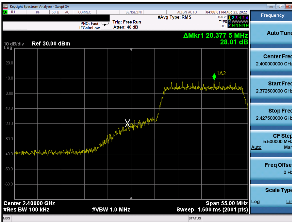
Plot 7-36. Band Edge Plot (802.11n MCS0 – Ch. 2)
