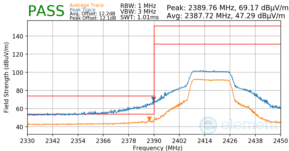
Plot 7-70. Radiated Restricted Lower Band Edge Measurement
