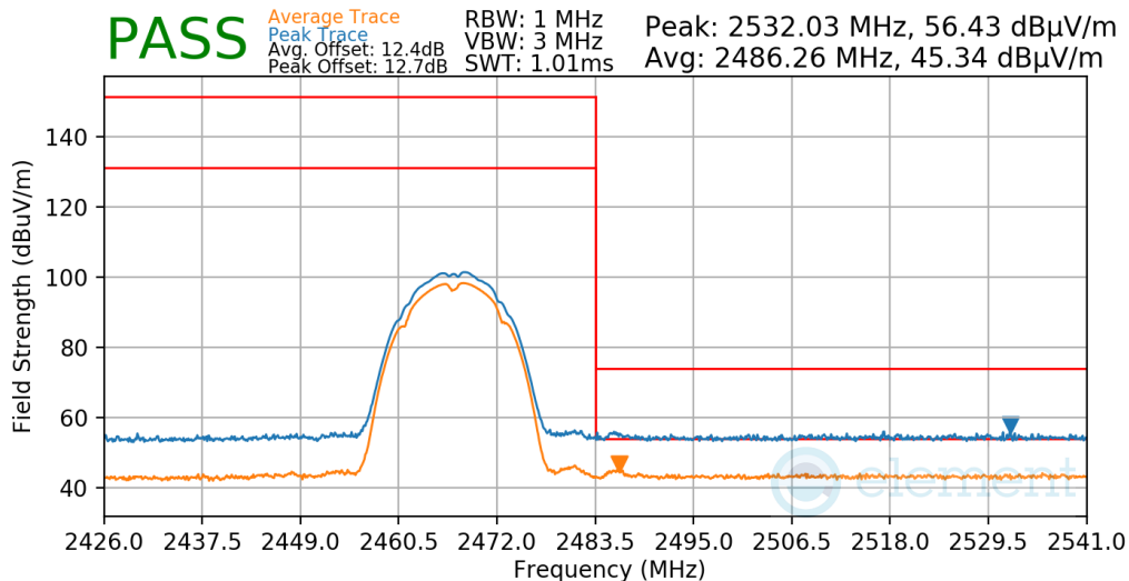
Plot 7-60. Radiated Restricted Upper Band Edge Measurement
