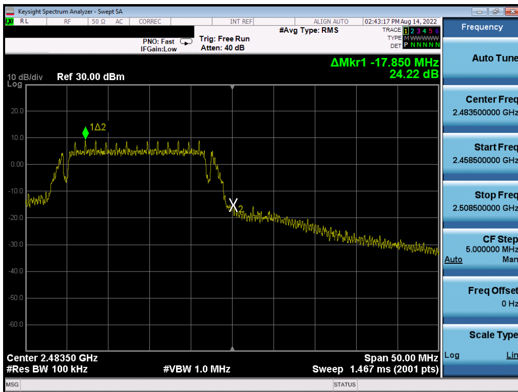
Plot 7-34. Band Edge Plot (802.11g – Ch. 13)
