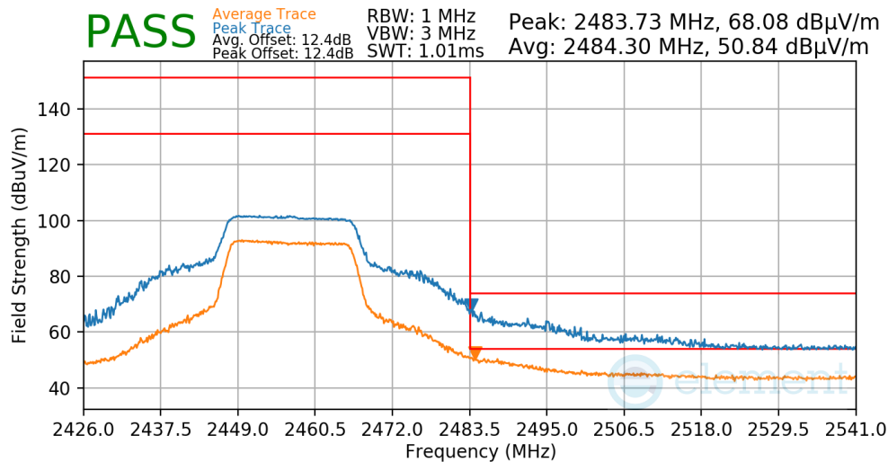
Plot 7-63. Radiated Restricted Upper Band Edge Measurement
