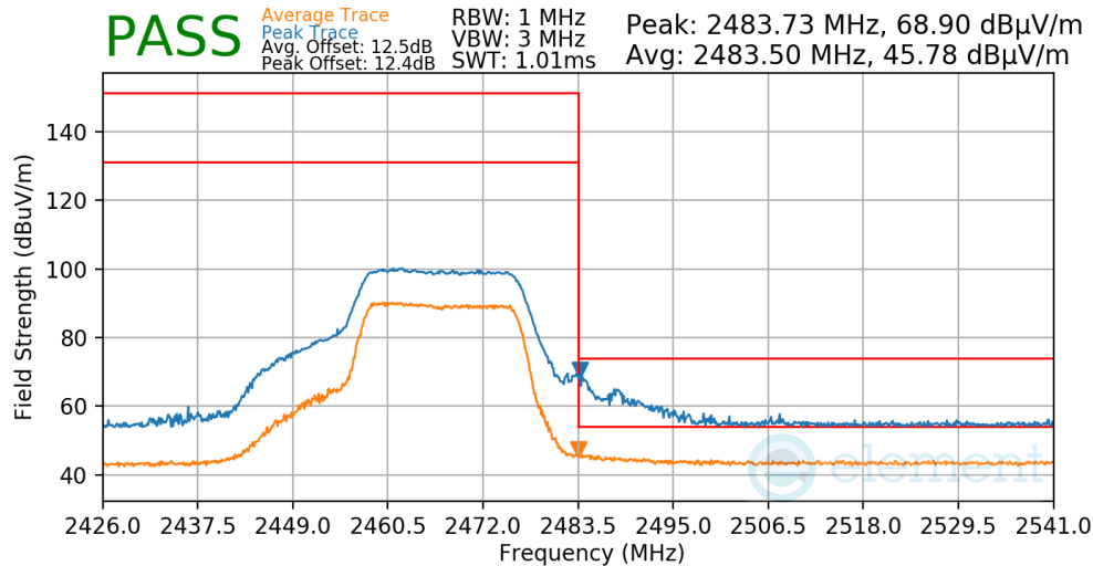
Plot 7-73. Radiated Restricted Upper Band Edge Measurement
