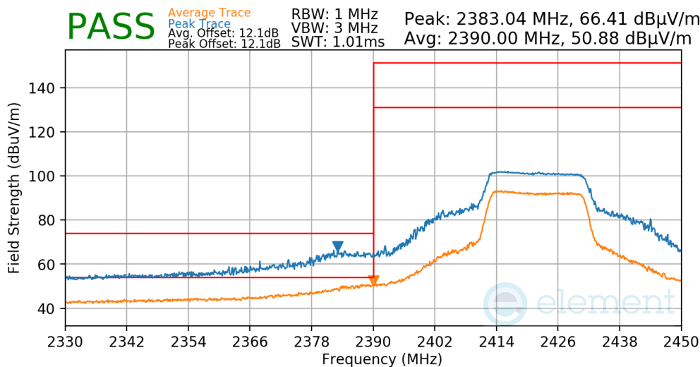
Plot 7-64. Radiated Restricted Lower Band Edge Measurement
