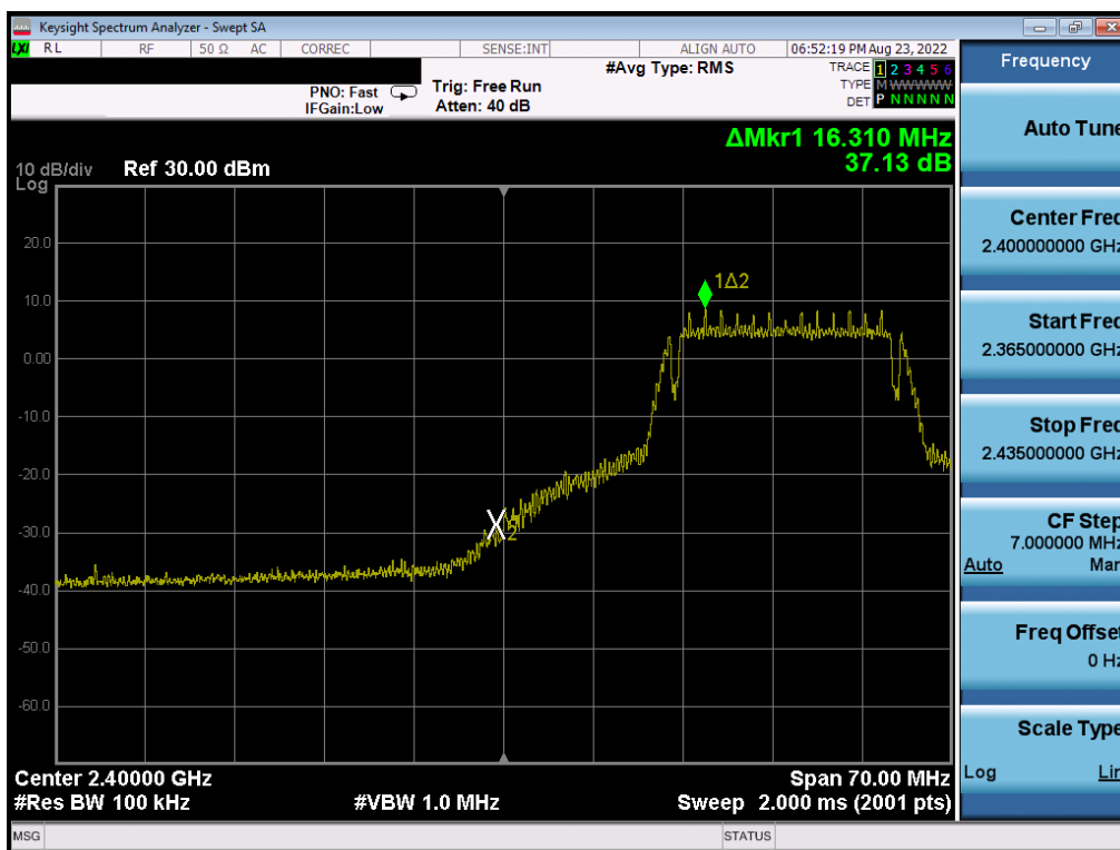
Plot 7-30. Band Edge Plot (802.11g – Ch. 3)
