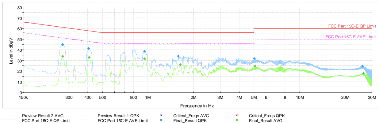
Plot 7-40. AC Line Conducted Plot with Bluetooth LE (N, 1Mbps ePA – Ch.39, with AC/DC Adapter + Magnetic Charger)
