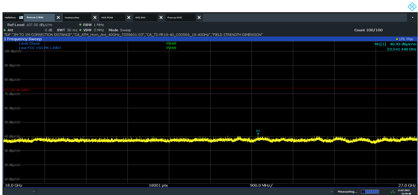
Plot 7-32. Radiated Spurious Plot Above 18GHz (1Mbps, ePA – Ch. 39, Pol.H)
