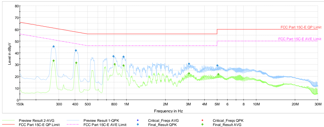
Plot 7-39. AC Line Conducted Plot with Bluetooth LE (L1, 1Mbps ePA – Ch.39 with AC/DC Adapter + Magnetic Charger)
