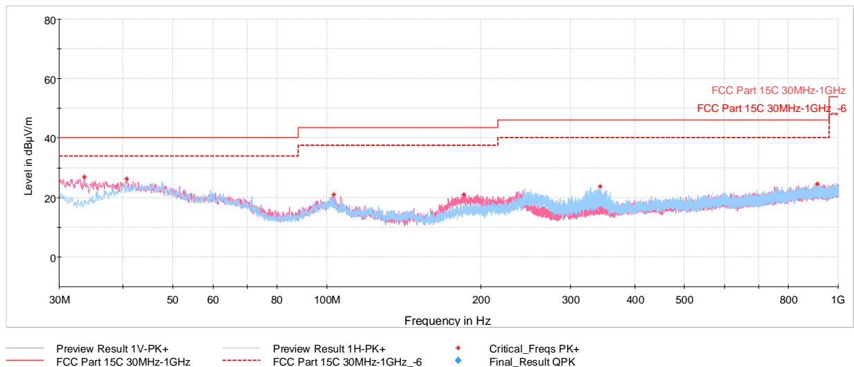
Plot 7-38. Radiated Spurious Plot Below 1GHz (1Mbps, ePA – Ch.39, Pol. H & V, with AC/DC Adapter + Magnetic Charger)
