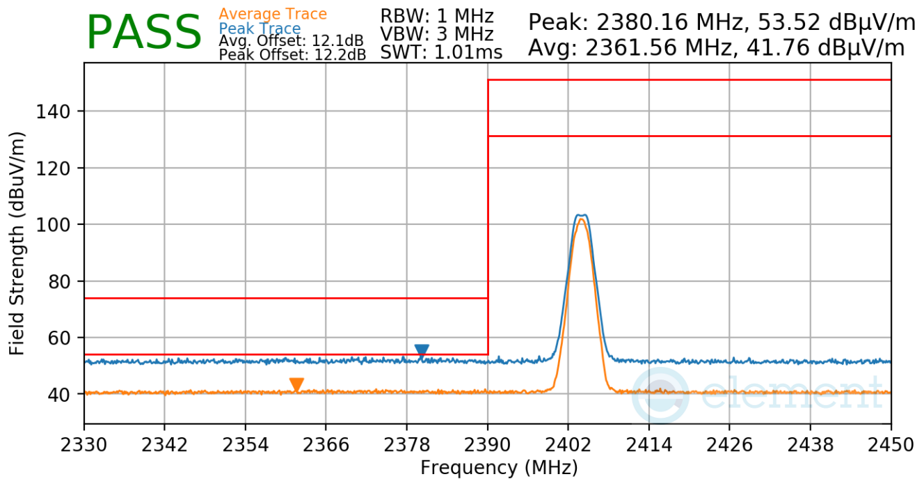
Plot 7-36. Radiated Restricted Lower Band Edge Measurement
