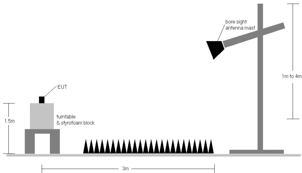
Figure 7-1. Test Setup
