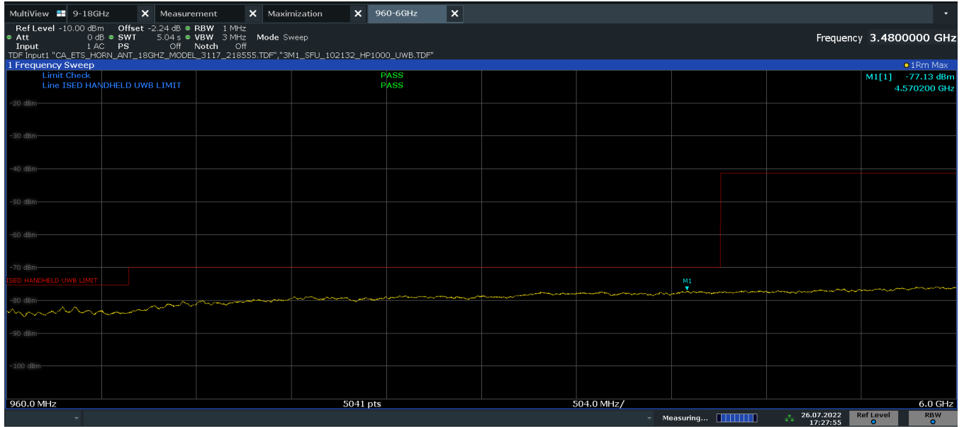
Plot 7-9. ISED Radiated Spurious Emission 960-6000MHz (Ch. 9, Config 0, Payload 125 Ant. Pol. H)
