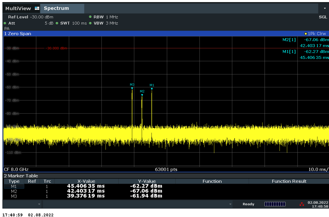
Plot 7-6. Zoom in Cessation Time – Mode1 (Ch.9, 8GHz)
