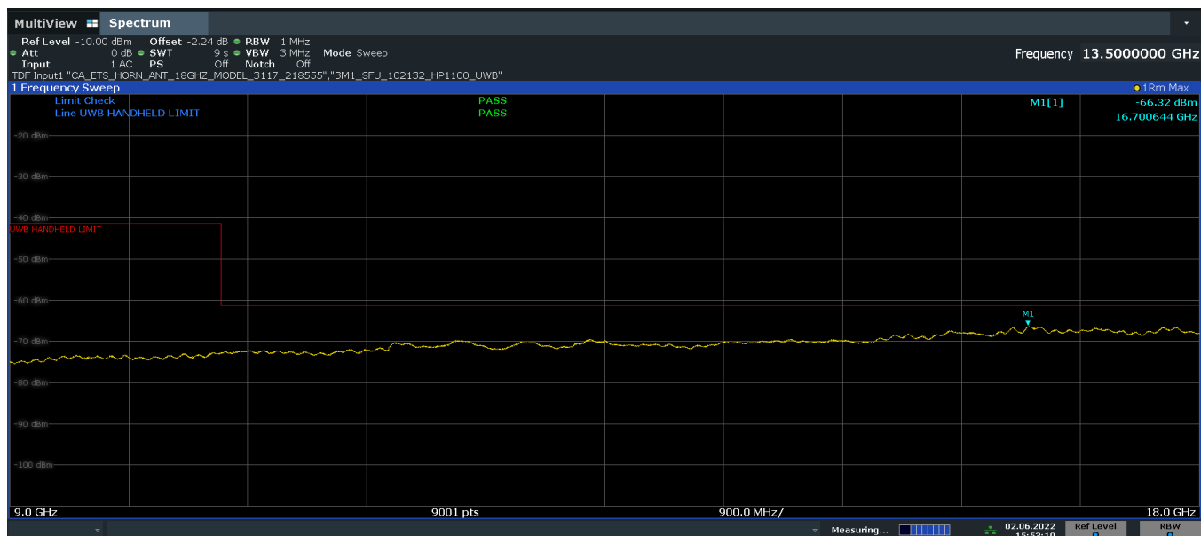
Plot 7-16. Radiated Spurious Emission 9-18GHz (Ch. 9, Config 0, Payload 125 Ant. Pol. V)
