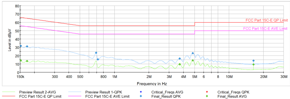
Plot 7-23. AC Line Conducted (Ch.9, Config 0, Payload 125, L1, with AC/DC Adapter)
