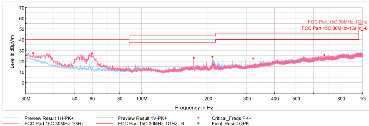
Plot 7-22. Radiated Spurious Emission – Simultaneous Transmission below 960MHz with AC/DC Adapter
