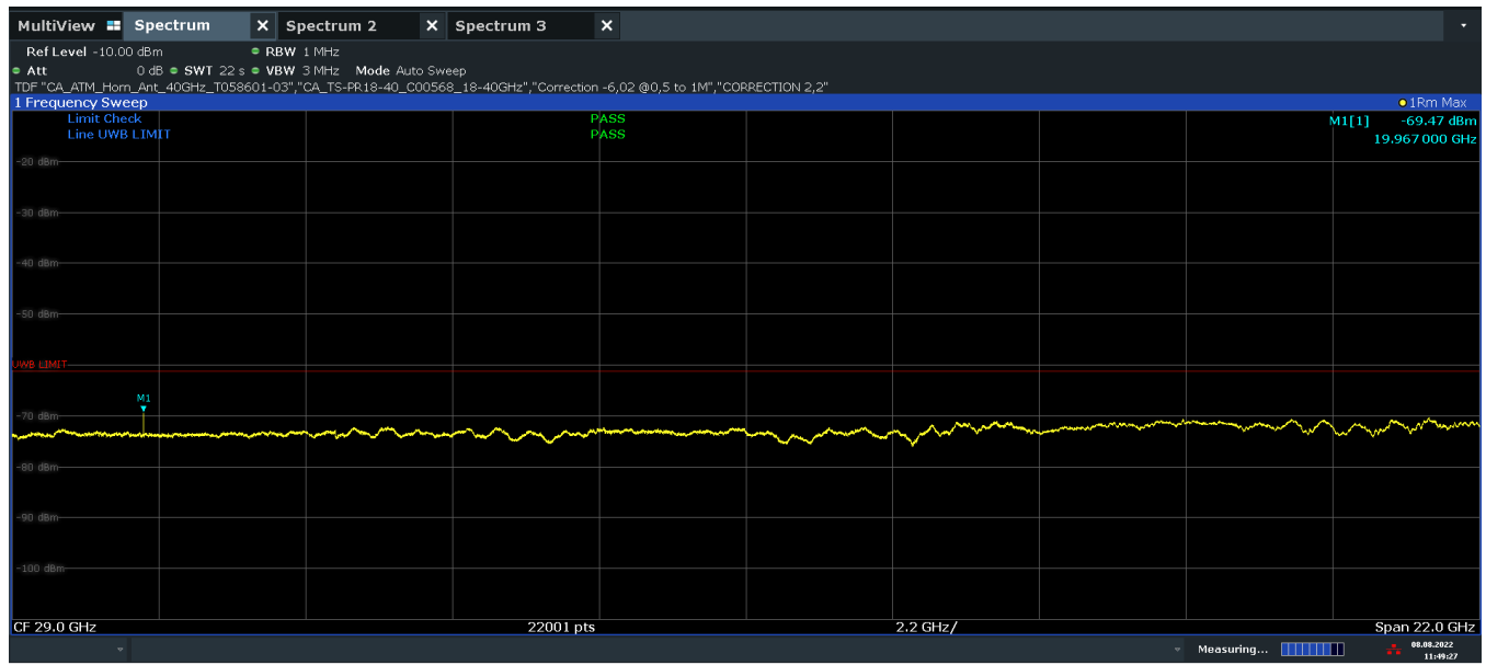
Plot 7-20. Radiated Spurious Simultaneous Transmission 18-40GHz (Ch.9, Config 3, Payload 125)
