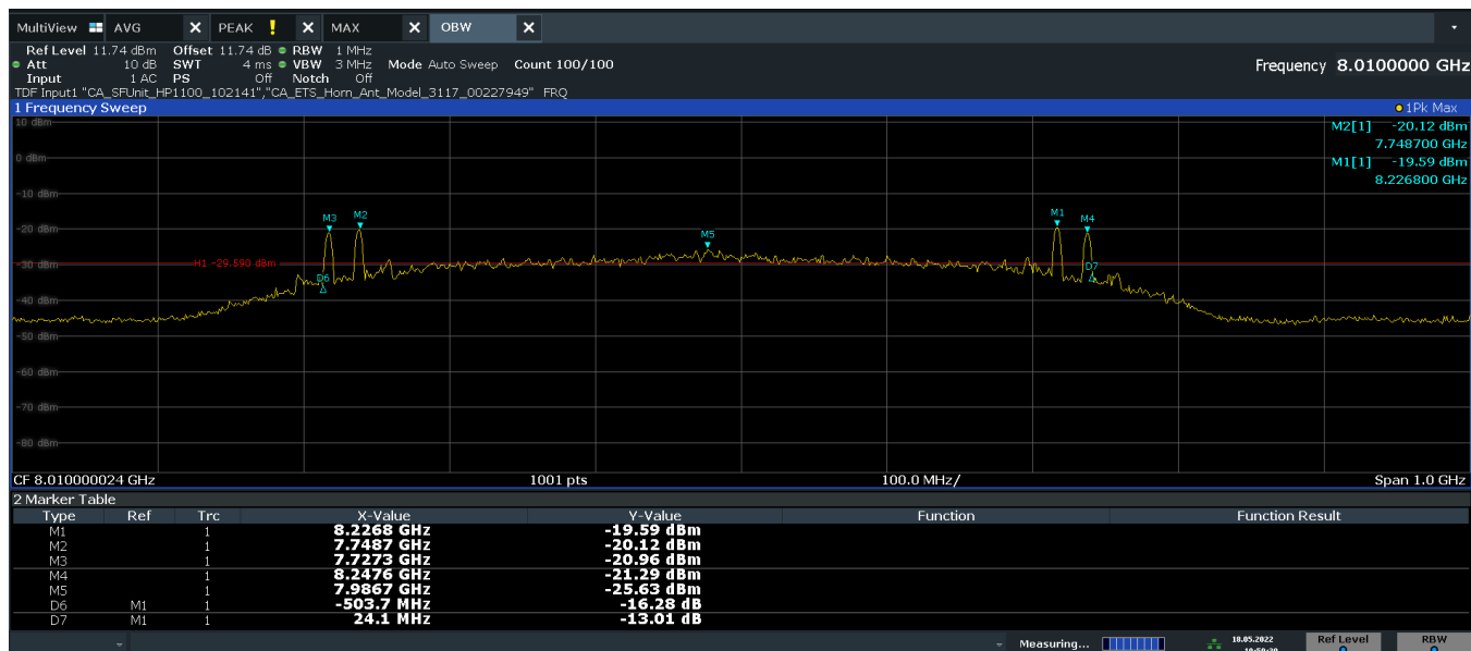
Plot 7-1. 10dBc Bandwidth Plot (UWB, Ch. 9, Config 0/Payload 125)
