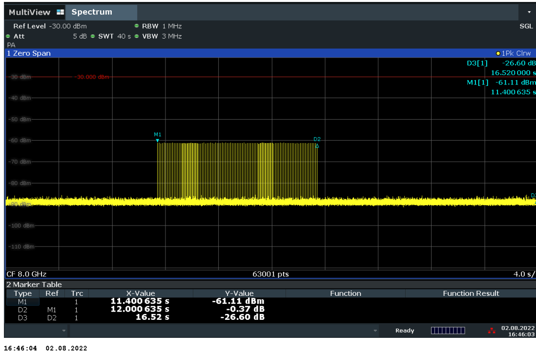
Plot 7-5. Cessation Time – Mode1 (Ch.9, 8GHz)
