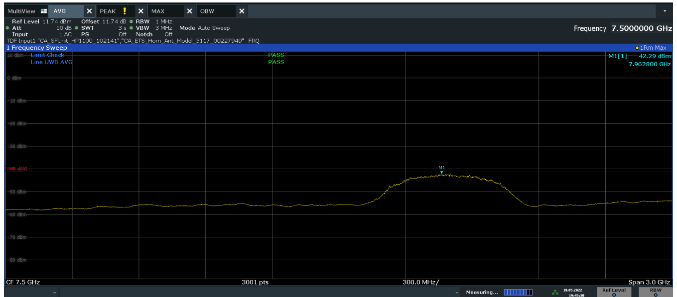
Plot 7-4. Average Radiated Power (UWB, Ch. 9, Config 0/Payload 125)
