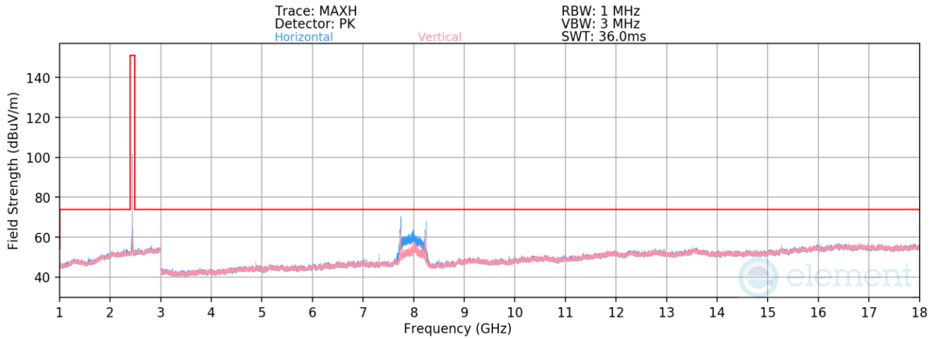
Plot 7-19. Radiated Spurious Simultaneous Transmission 1-18GHz (Ch.9, Config 3, Payload 125)
