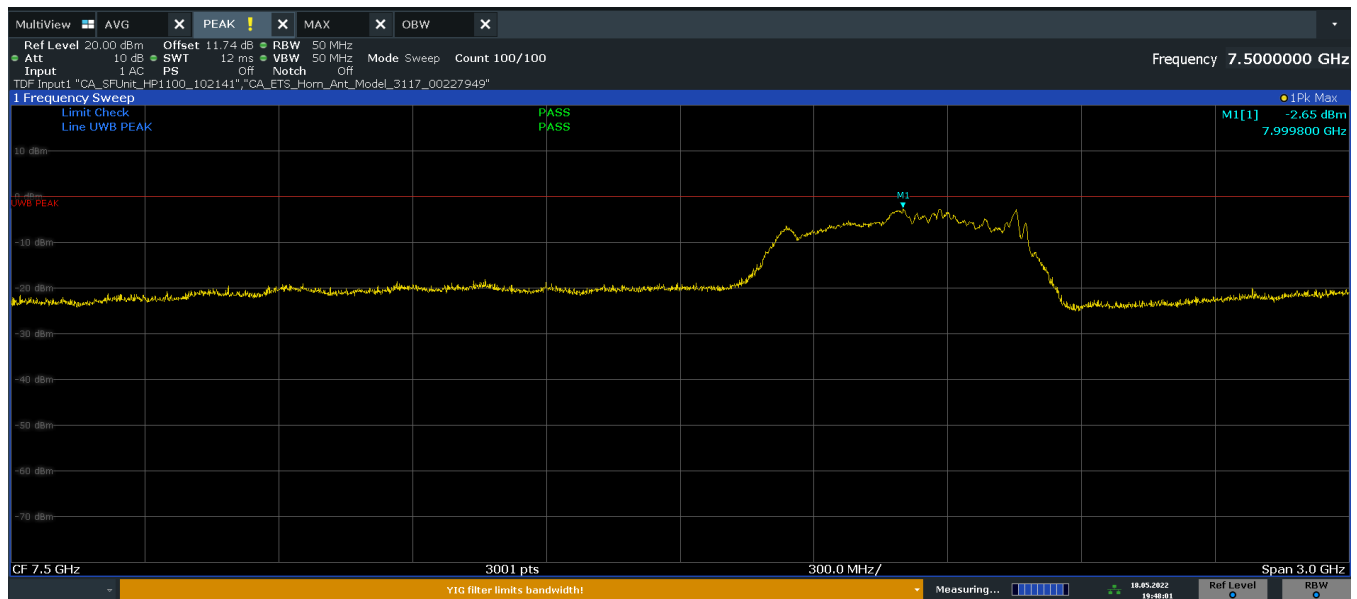
Plot 7-3. Peak Radiated Power (UWB, Ch. 9, Config 0/Payload 125)
