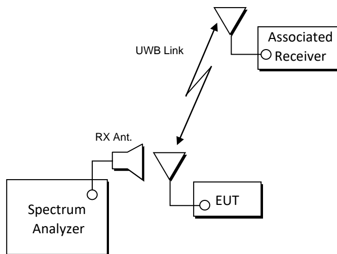
Figure 7-4. Test Setup
