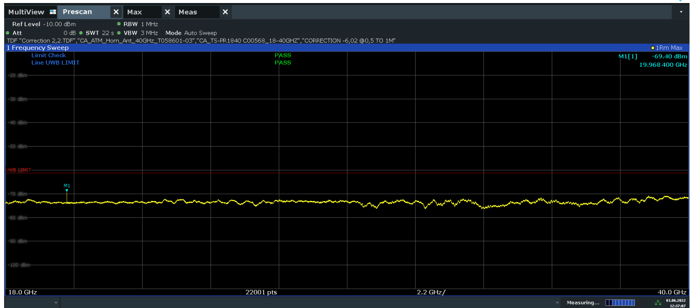
Plot 7-17. Radiated Spurious Emission 18-40GHz (Ch.9, Config 3, Payload 125 Ant. Pol. H)
