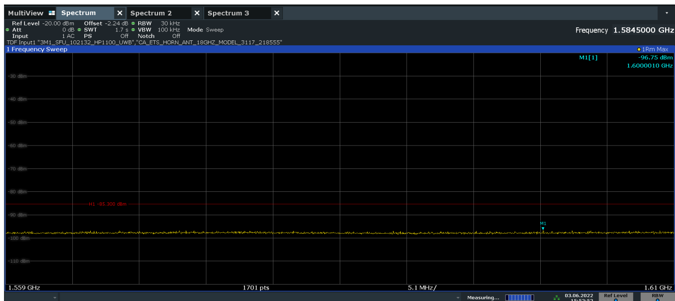
Plot 7-14. Radiated Spurious Emission 1559-1610MHz (Ch. 9, Config 0, Payload 0 Ant. Pol V)
