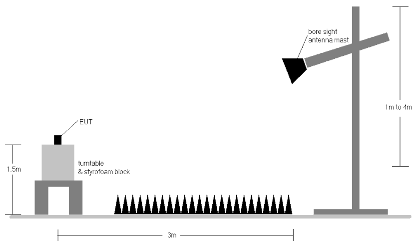
Figure 7-2. Test Instrument & Measurement Setup
