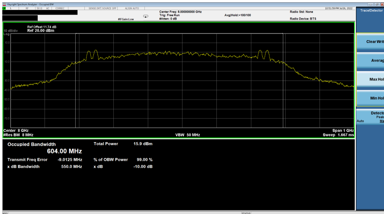
Plot 7-2. ISED 10dBc Bandwidth & 99% OBW (UWB, Ch. 9, Config 0/Payload 125)
