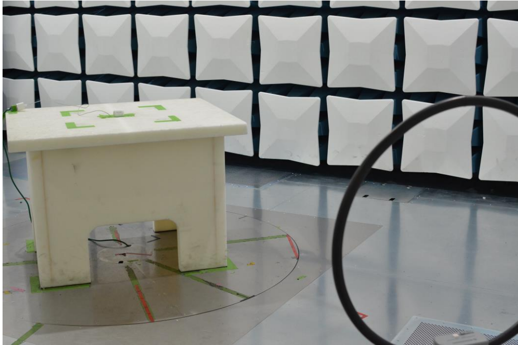
Figure 25: 9kHz-30MHz Test Setup (Front View)
