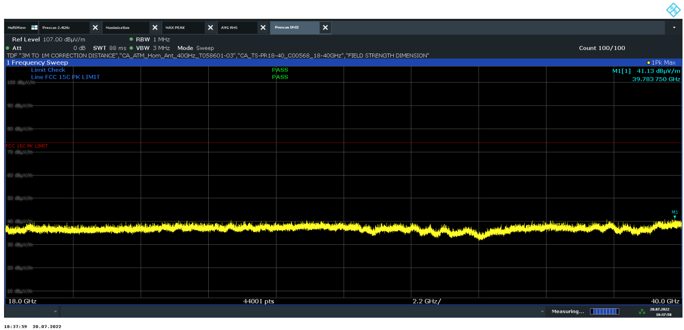
Plot 7-16. Radiated Spurious Emissions Above 18GHz (LE2M – 5245MHz Pol. H)
