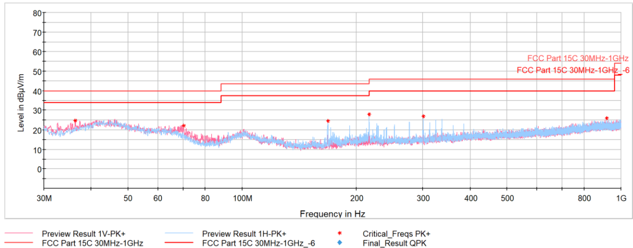
Plot 7-24. RSE 30MHz - 1GHz (LE2M - 5245MHz), with AC/DC Adapter and lightning cable
