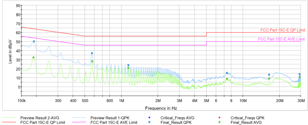
Plot 7-26. AC Line Conducted Plot (LE2M – 5245MHz) (N) with host PC and lightning charger
