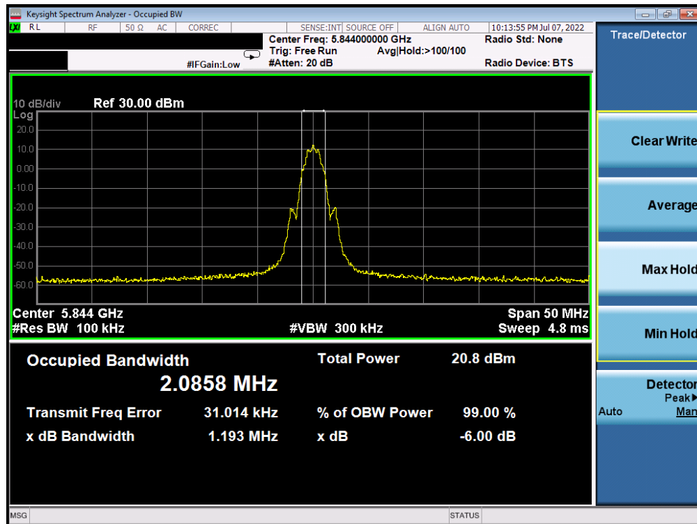
Plot 7-6. 6dB BW & 99% OBW (LE2M, 5844MHz)
