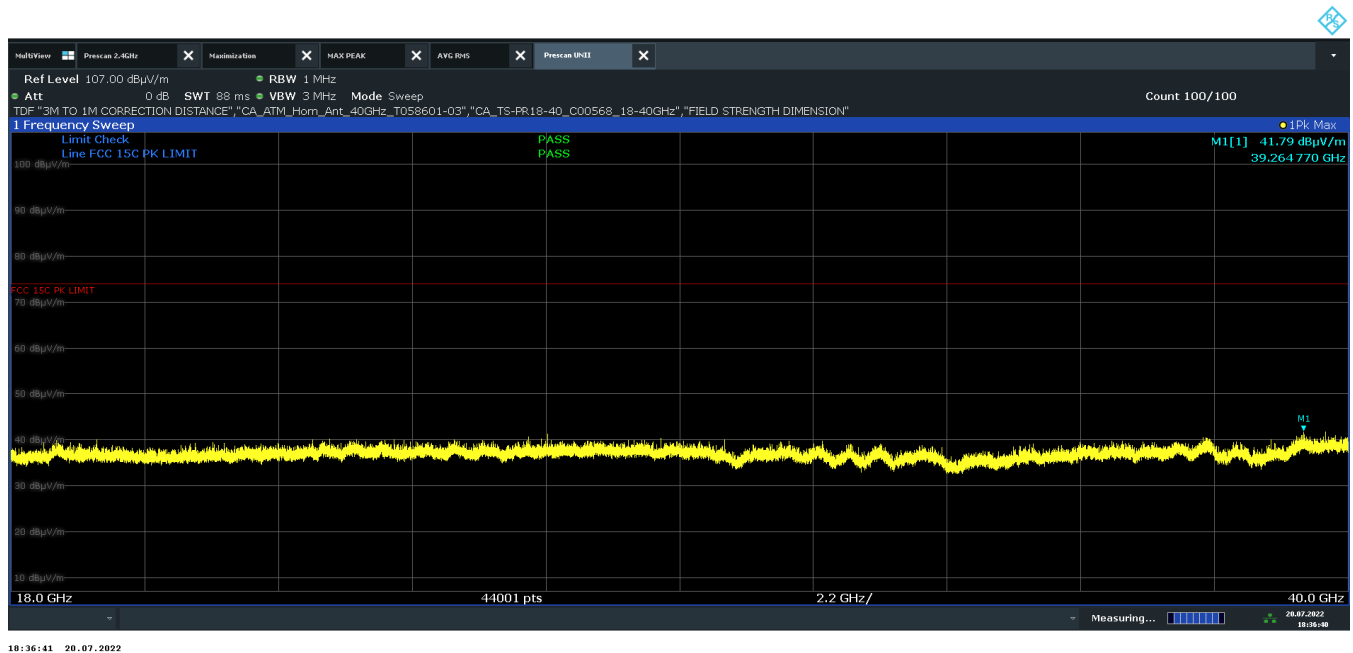
Plot 7-17. Radiated Spurious Emissions Above 18GHz (LE2M – 5245MHz Pol. V)
