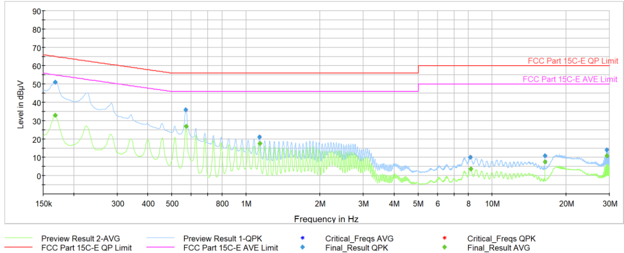
Plot 7-25. AC Line Conducted Plot (LE2M – 5245MHz) (L1) with host PC and lightning charger
