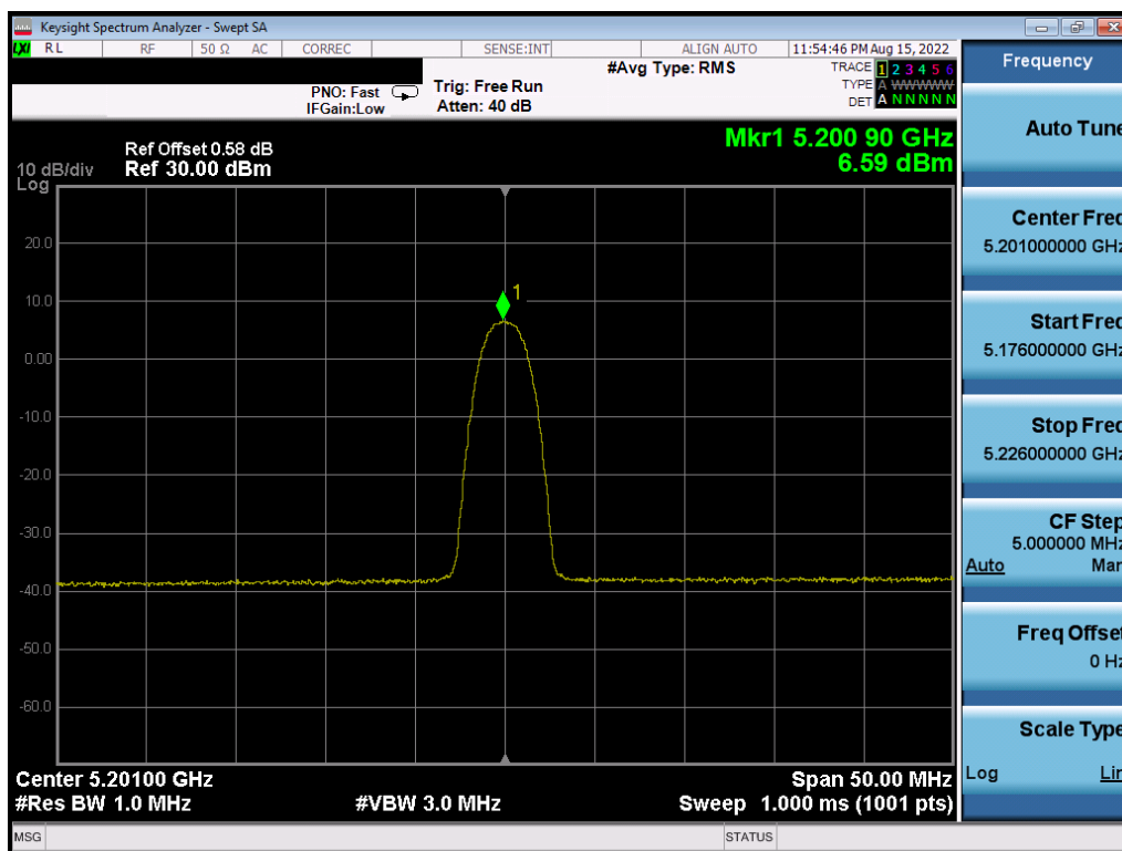
Plot 7-32. PSD (HDRp4, 5201MHz)
