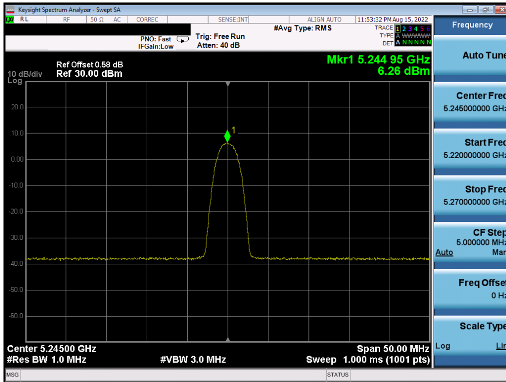
Plot 7-33. PSD (HDRp4, 5245MHz)
