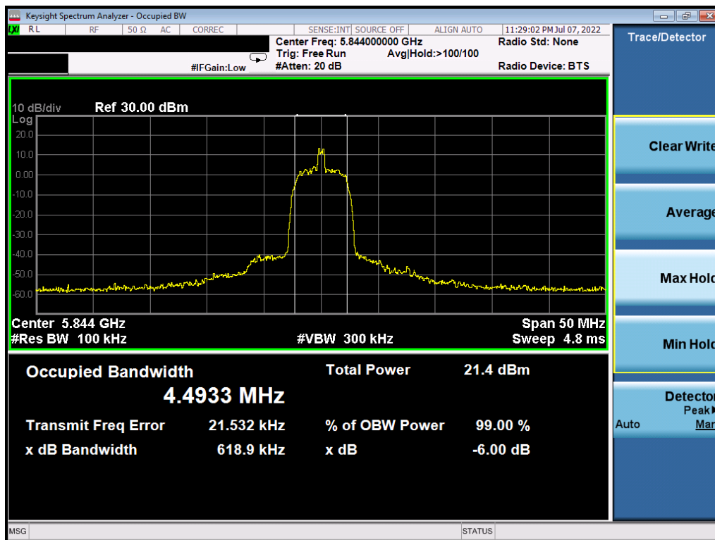
Plot 7-18. 6dB BW & 99% OBW (HDR8, 5844MHz)
