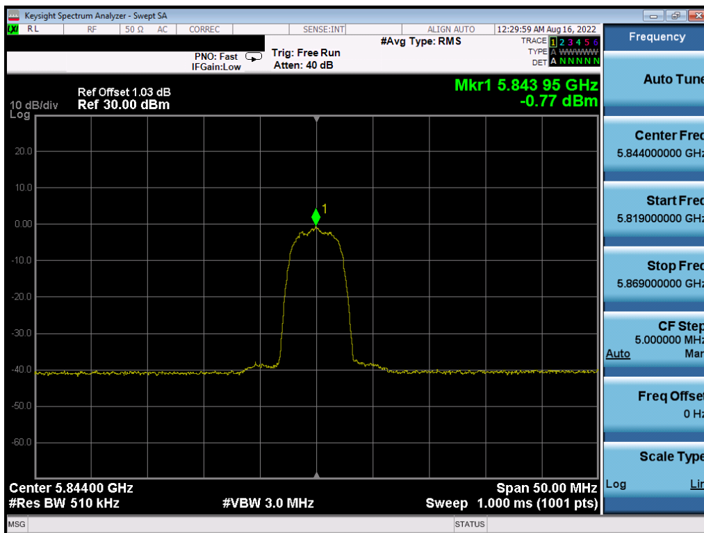
Plot 7-42. PSD (HDR8, 5844MHz)
