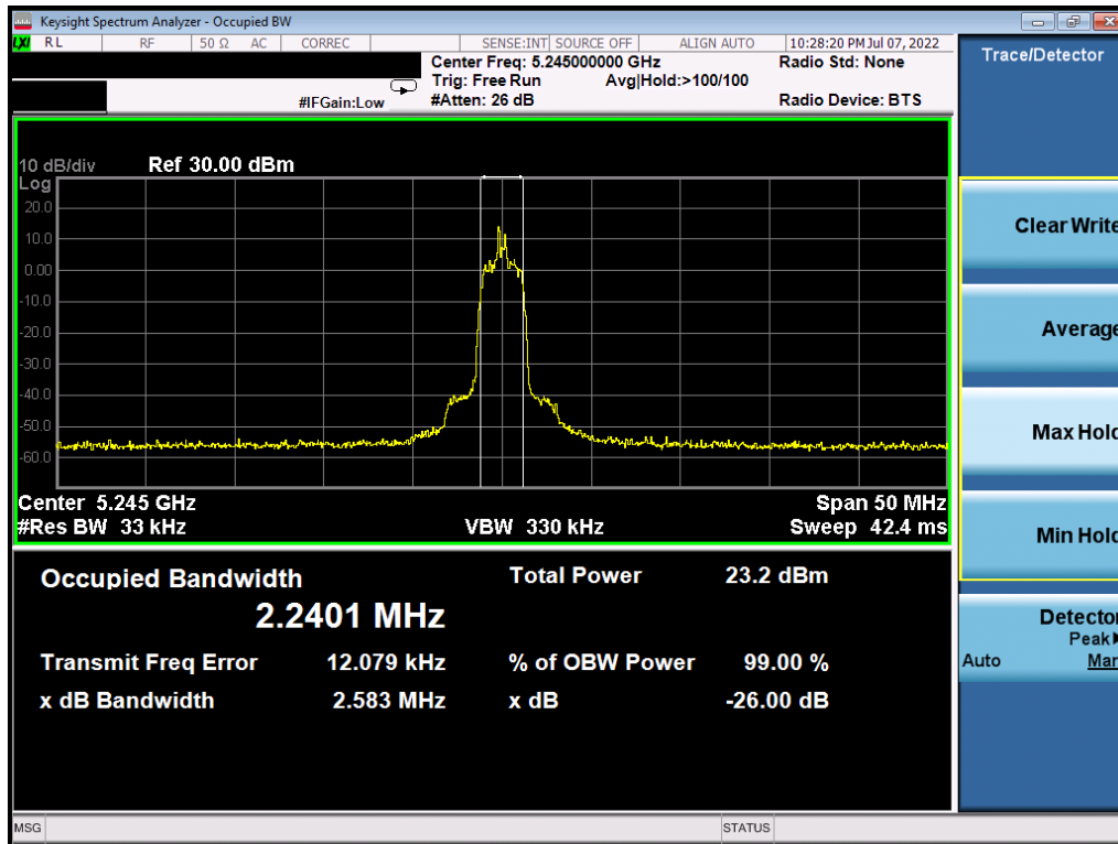
Plot 7-3. 26dB BW & 99% OBW (HDR4, 5245MHz)
