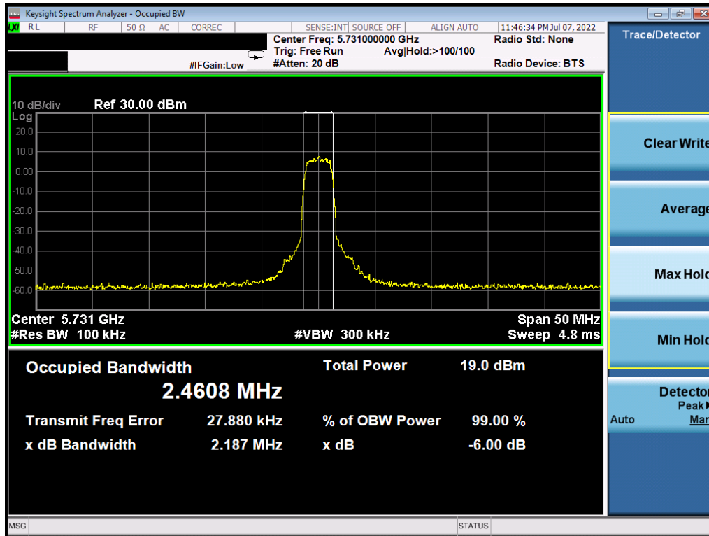
Plot 7-19. 6dB BW & 99% OBW (HDRp4, 5731MHz)
