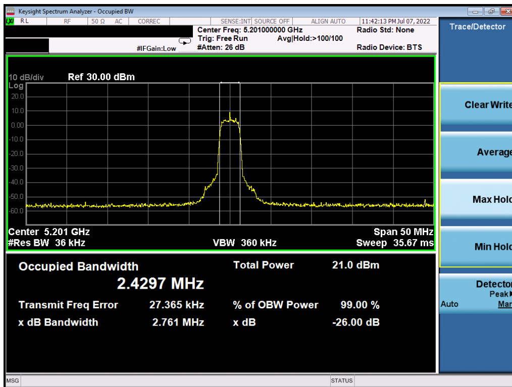
Plot 7-8. 26dB BW & 99% OBW (HDRp4, 5201MHz)
