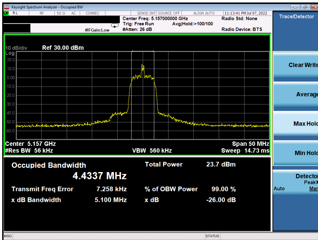
Plot 7-4. 26dB BW & 99% OBW (HDR8, 5157MHz)
