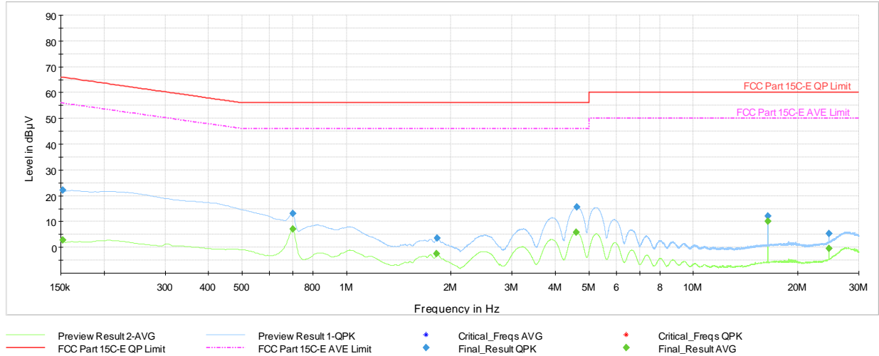
Plot 7-72. AC Line Conducted Plot (HDR4 – 5201MHz) (L1) with AC/DC Adapter
