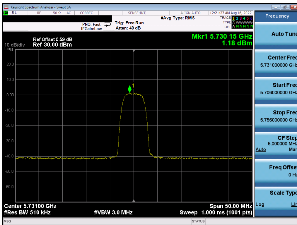
Plot 7-46. PSD (HDRp8, 5731MHz)
