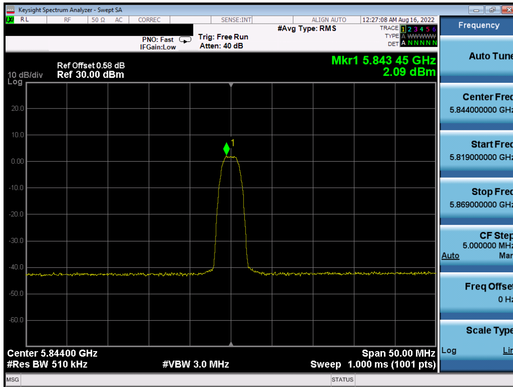
Plot 7-45. PSD (HDRp4, 5844MHz)
