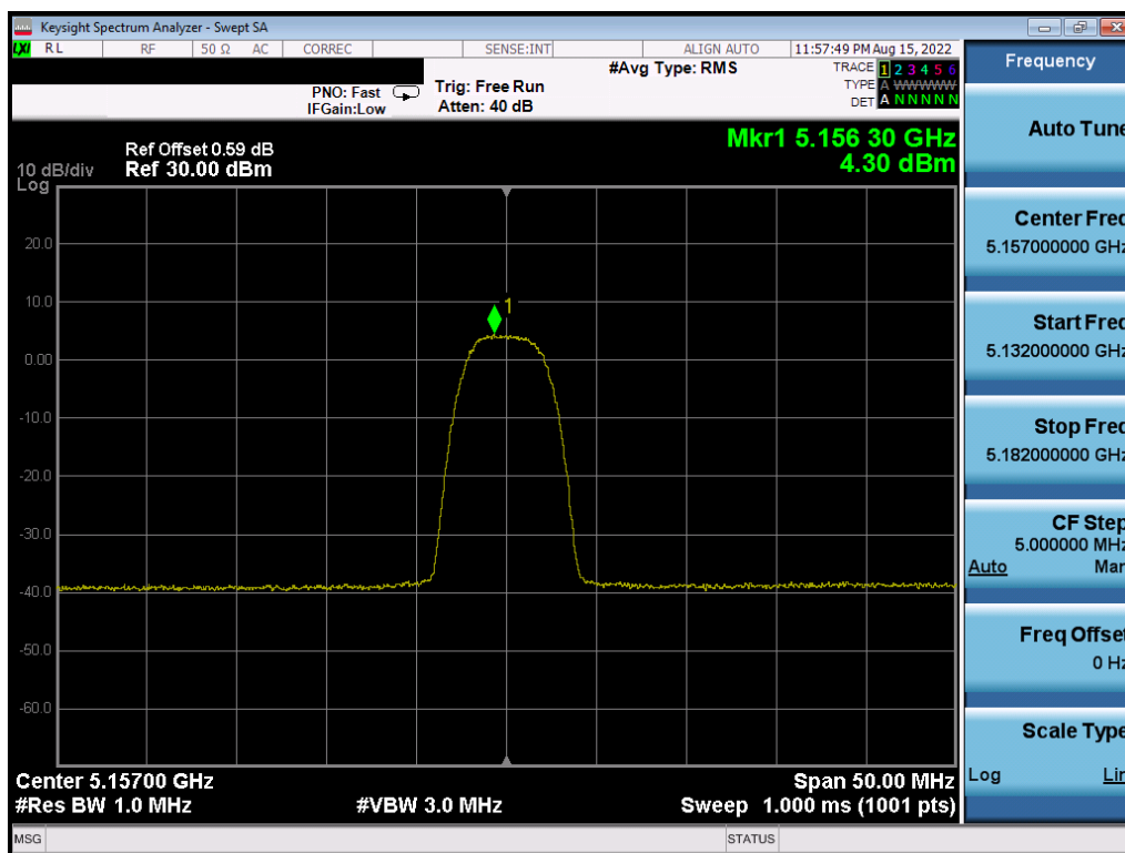
Plot 7-34. PSD (HDRp8, 5157MHz)
