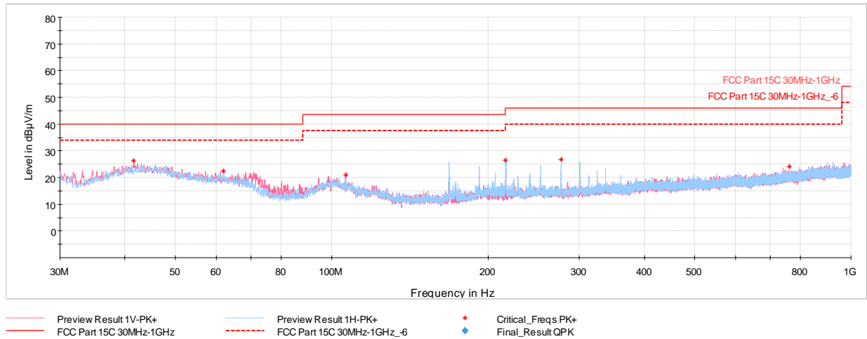
Plot 7-71. RSE 30MHz - 1GHz (HDR4 - 5201MHz), with AC/DC Adapter
