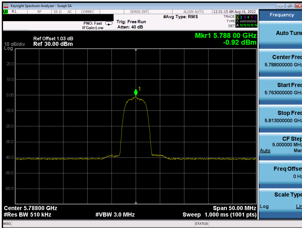
Plot 7-41. PSD (HDR8, 5788MHz)
