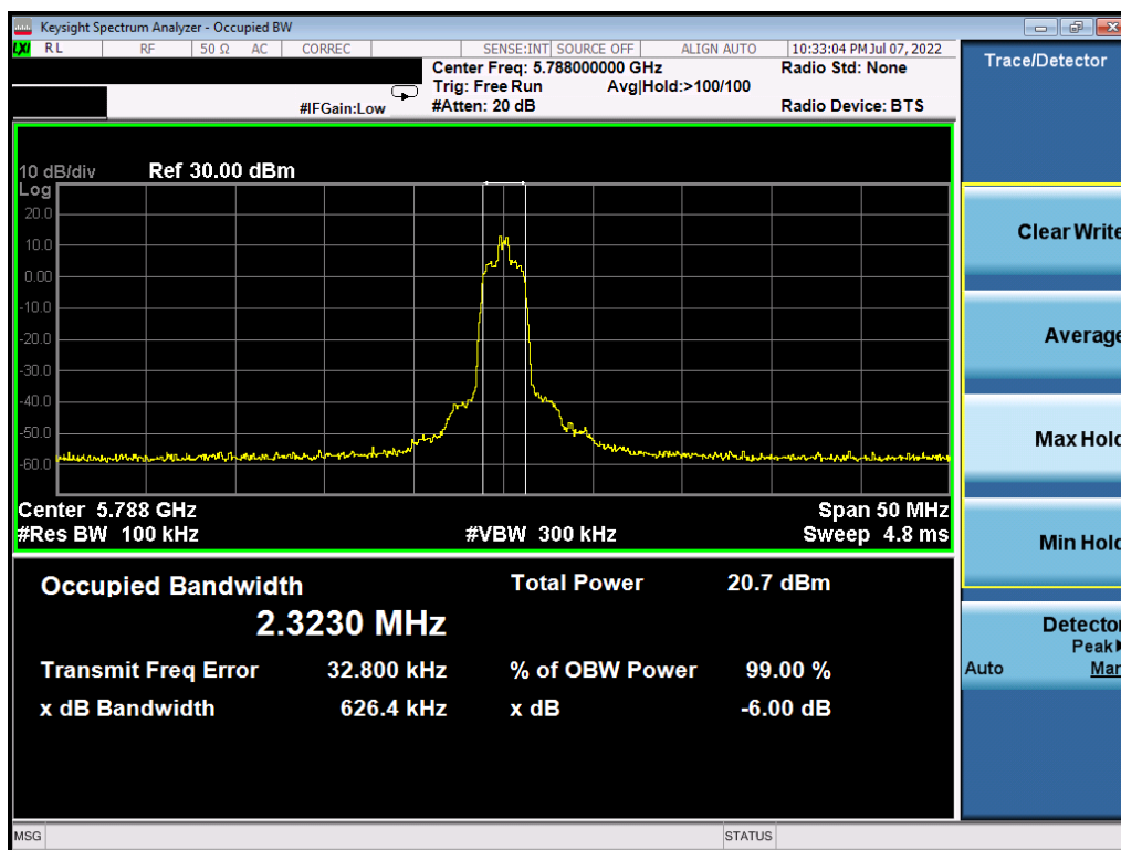
Plot 7-14. 6dB BW & 99% OBW (HDR4, 5788MHz)
