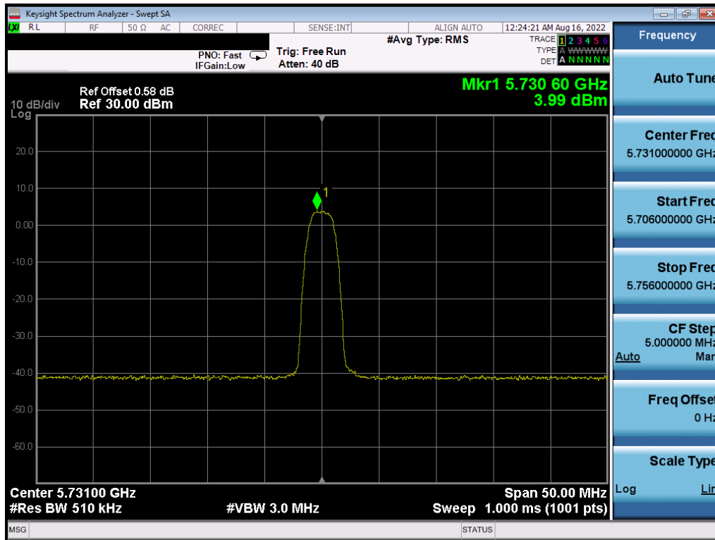
Plot 7-43. PSD (HDRp4, 5731MHz)
