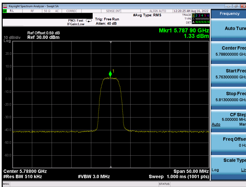
Plot 7-47. PSD (HDRp8, 5788MHz)
