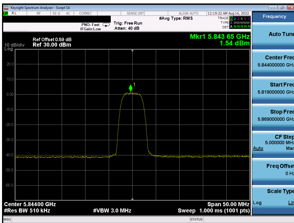
Plot 7-48. PSD (HDRp8, 5844MHz)
