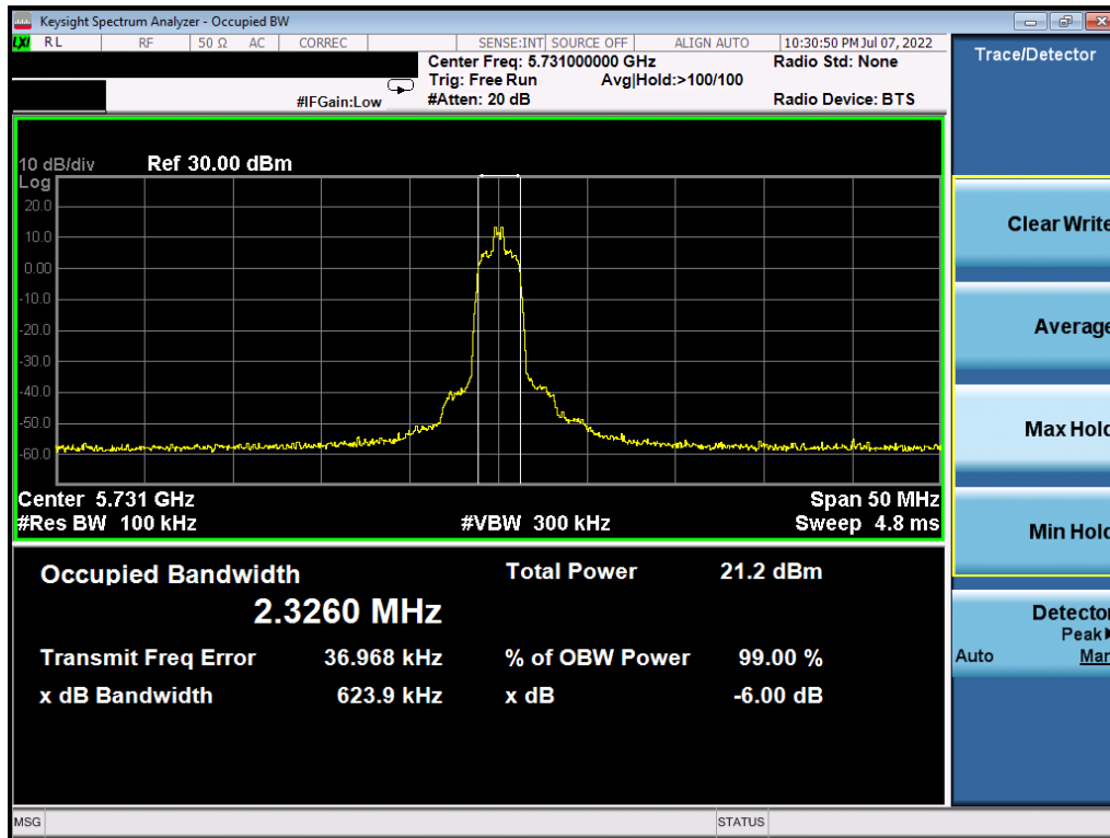
Plot 7-13. 6dB BW & 99% OBW (HDR4, 5731MHz)
