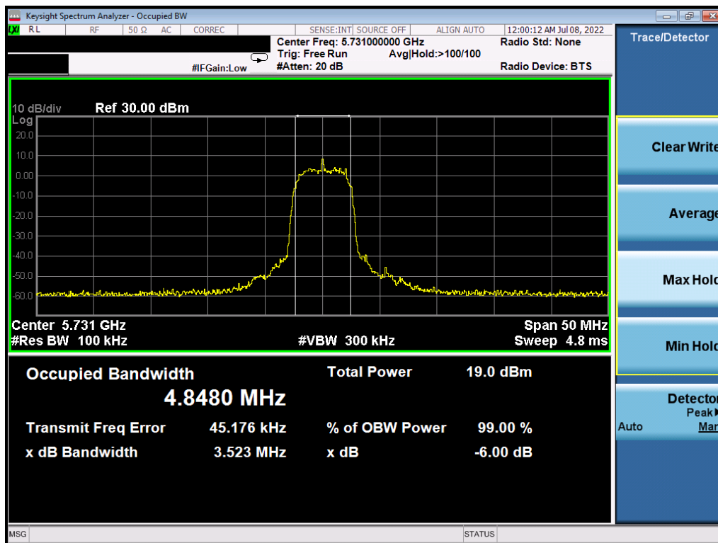
Plot 7-22. 6dB BW & 99% OBW (HDRp8, 5731MHz)
