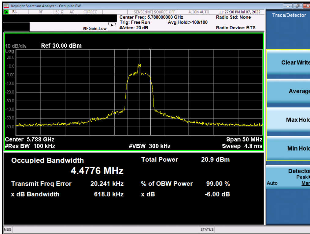
Plot 7-17. 6dB BW & 99% OBW (HDR8, 5788MHz)
