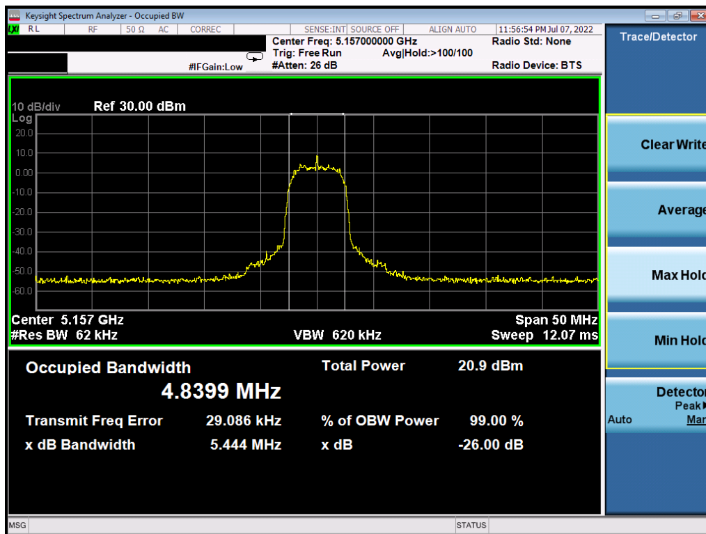
Plot 7-10. 26dB BW & 99% OBW (HDRp8, 5157MHz)
