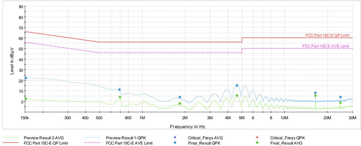
Plot 7-73. AC Line Conducted Plot (HDR4 – 5201MHz) (N) with AC/DC Adapter
