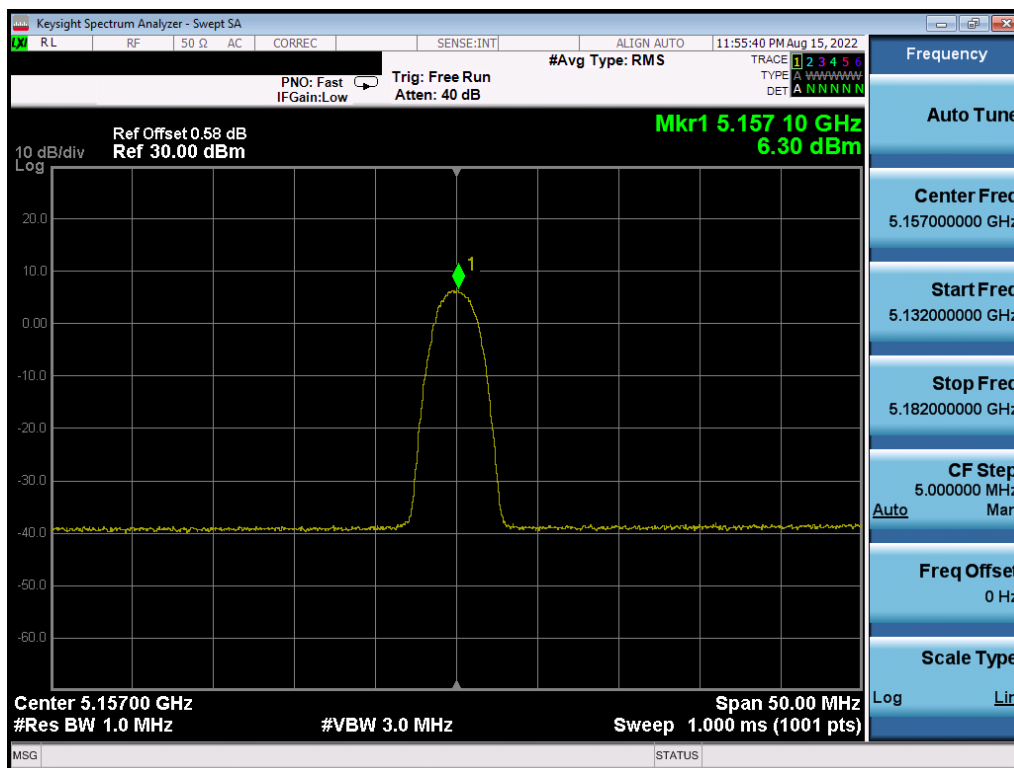
Plot 7-31. PSD (HDRp4, 5157MHz)
