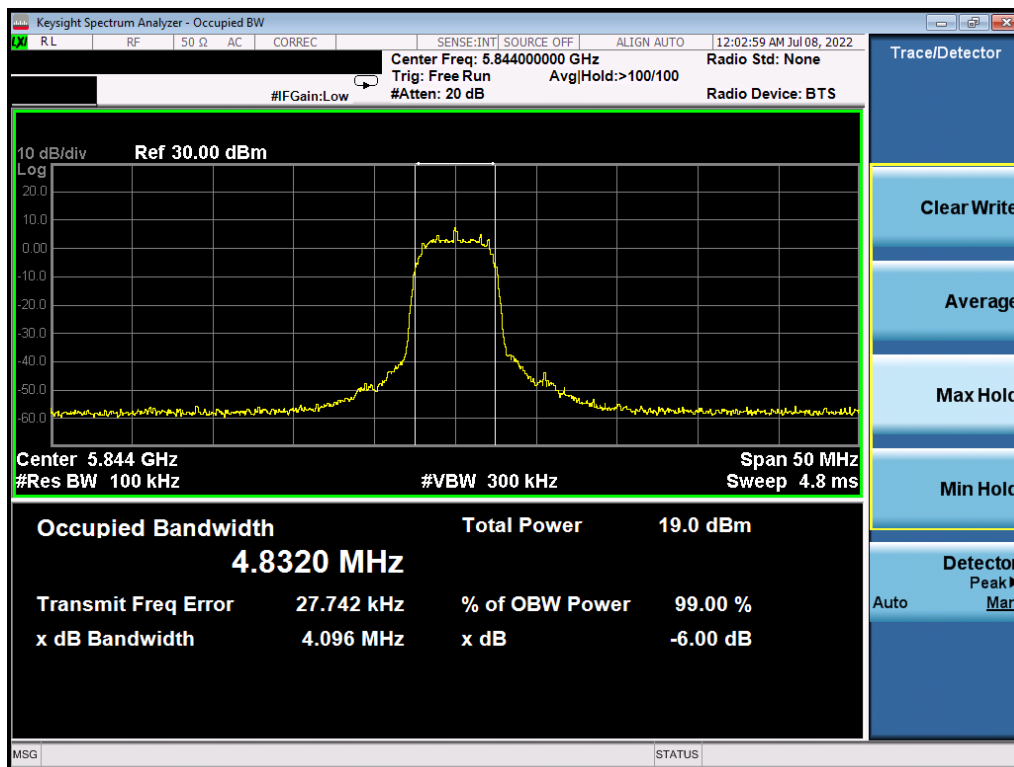
Plot 7-24. 6dB BW & 99% OBW (HDRp8, 5844MHz)
