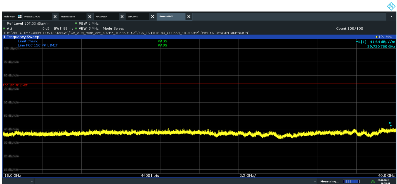
Plot 7-58. Radiated Spurious Emissions Above 18GHz (HDR4 – 5731MHz Pol. V)
