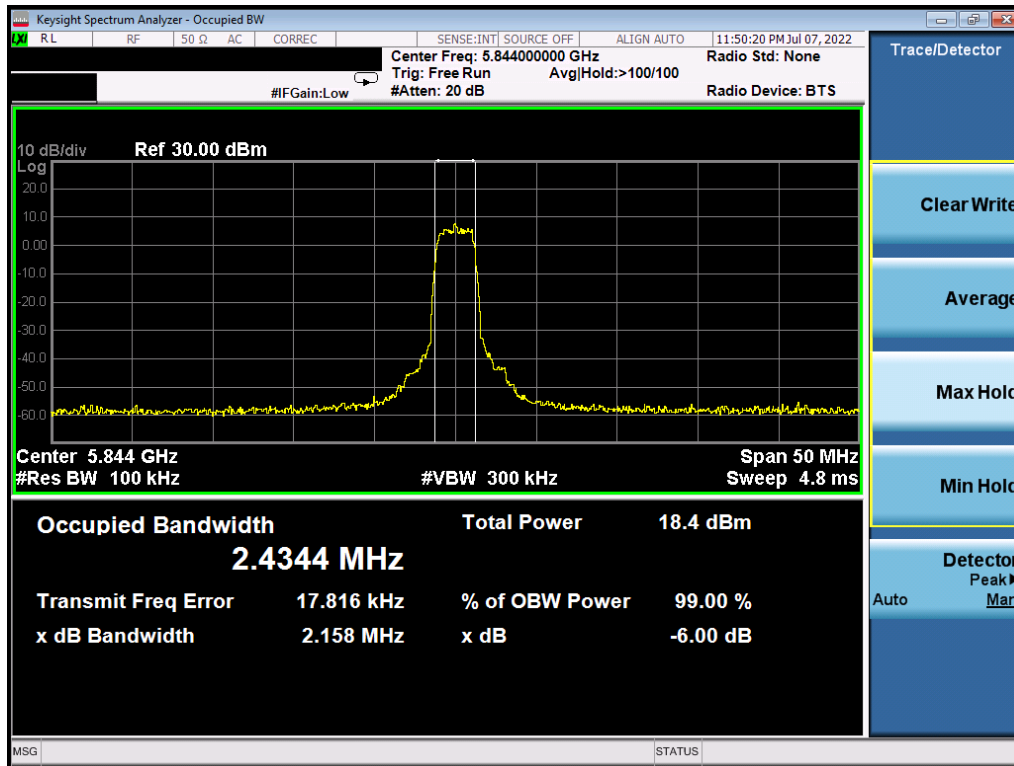
Plot 7-21. 6dB BW & 99% OBW (HDRp4, 5844MHz)
