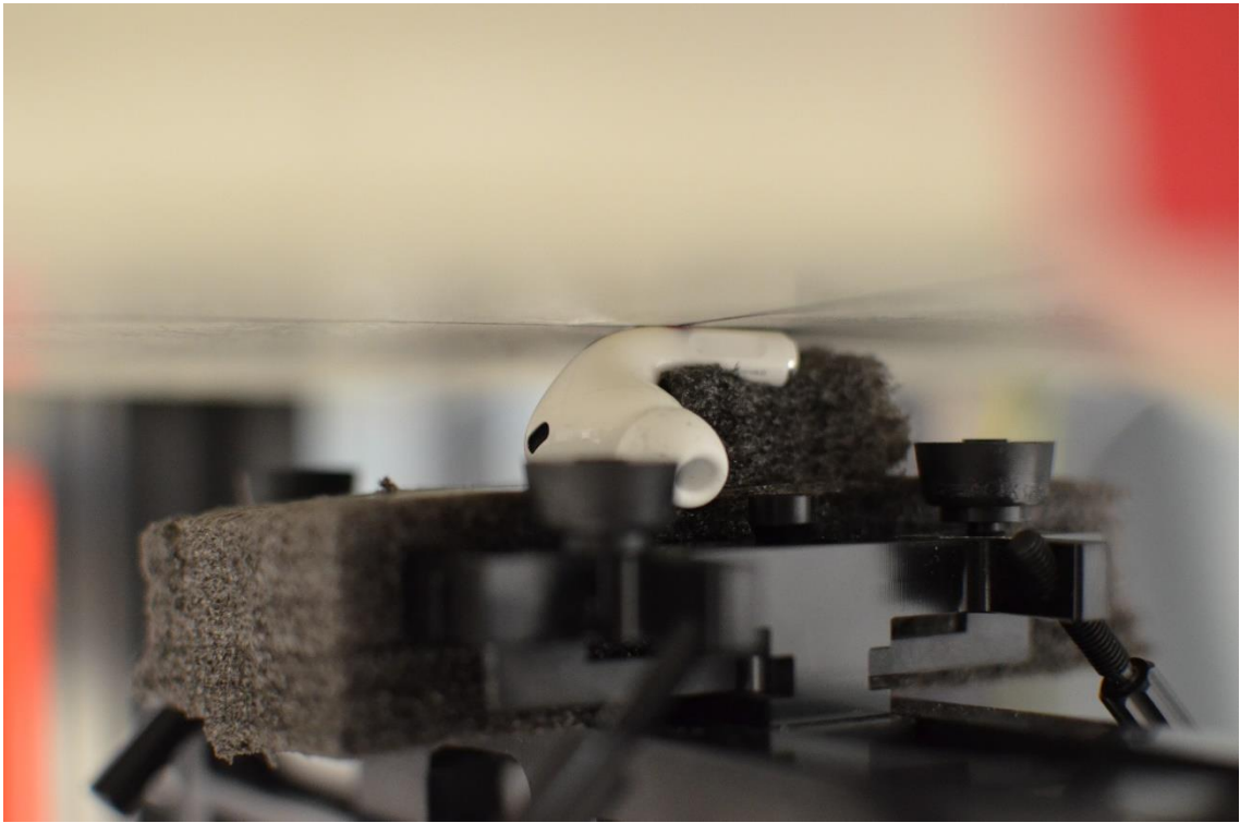
SAR Test Setup Photo 2: Body-Worn, Back Side, 0 mm
