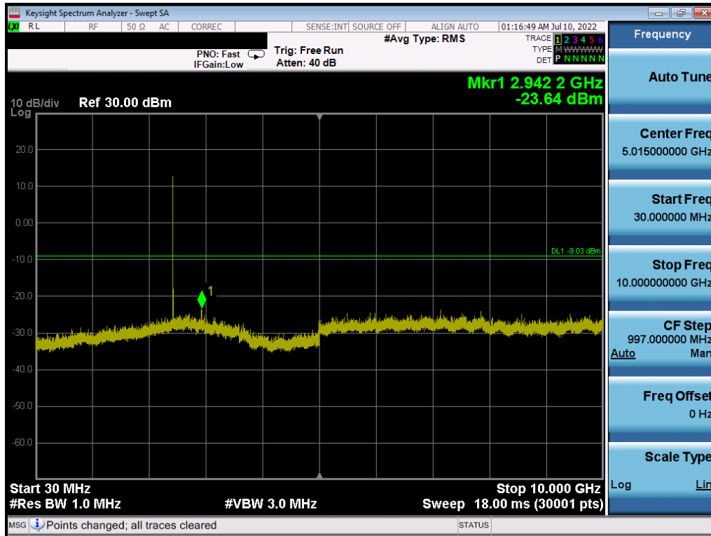
Plot 7-35. Conducted Spurious Plot (Bluetooth (HDRp8), 8 Mbps – Ch. 38)
