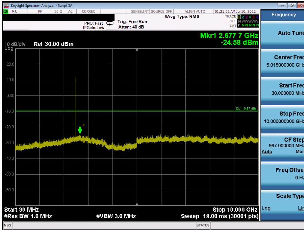
Plot 7-37. Conducted Spurious Plot (Bluetooth (HDRp8), 8 Mbps – Ch. 75)
