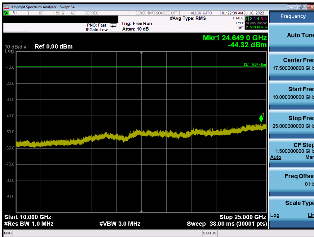
Plot 7-38. Conducted Spurious Plot (Bluetooth (HDRp8), 8 Mbps – Ch. 75)
