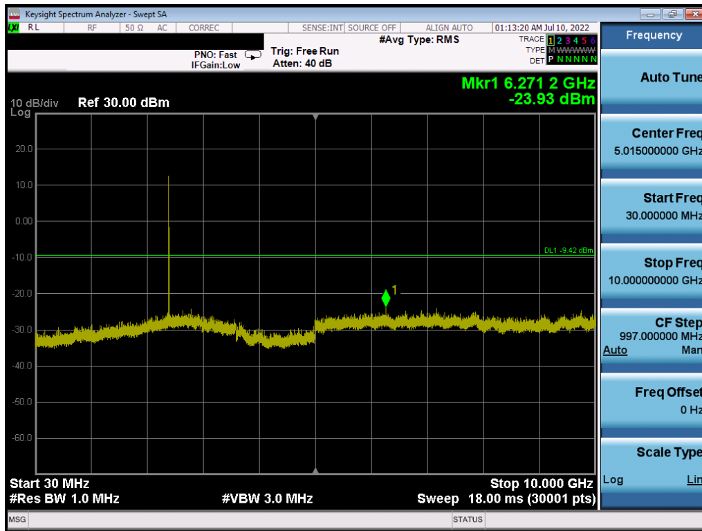
Plot 7-33. Conducted Spurious Plot (Bluetooth (HDP8), 8 Mbps – Ch. 1)
