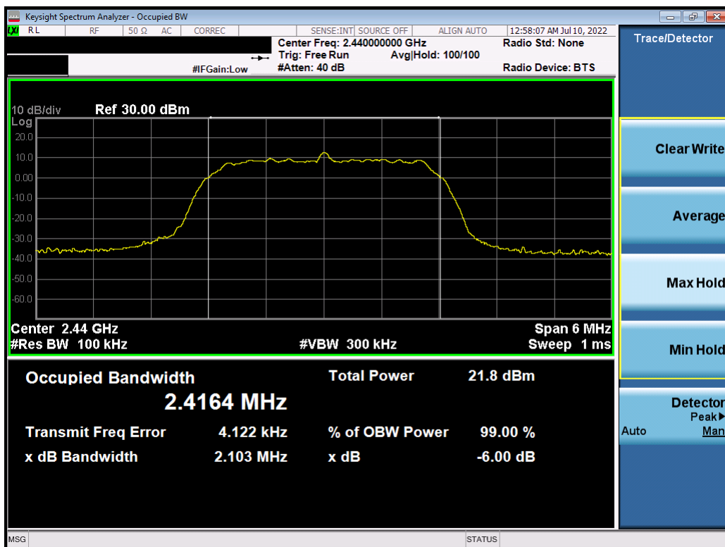
Plot 7-8. 6dB BW & 99% OBW Plot (Bluetooth (HDRp4), 4Mbps – Ch. 38)
