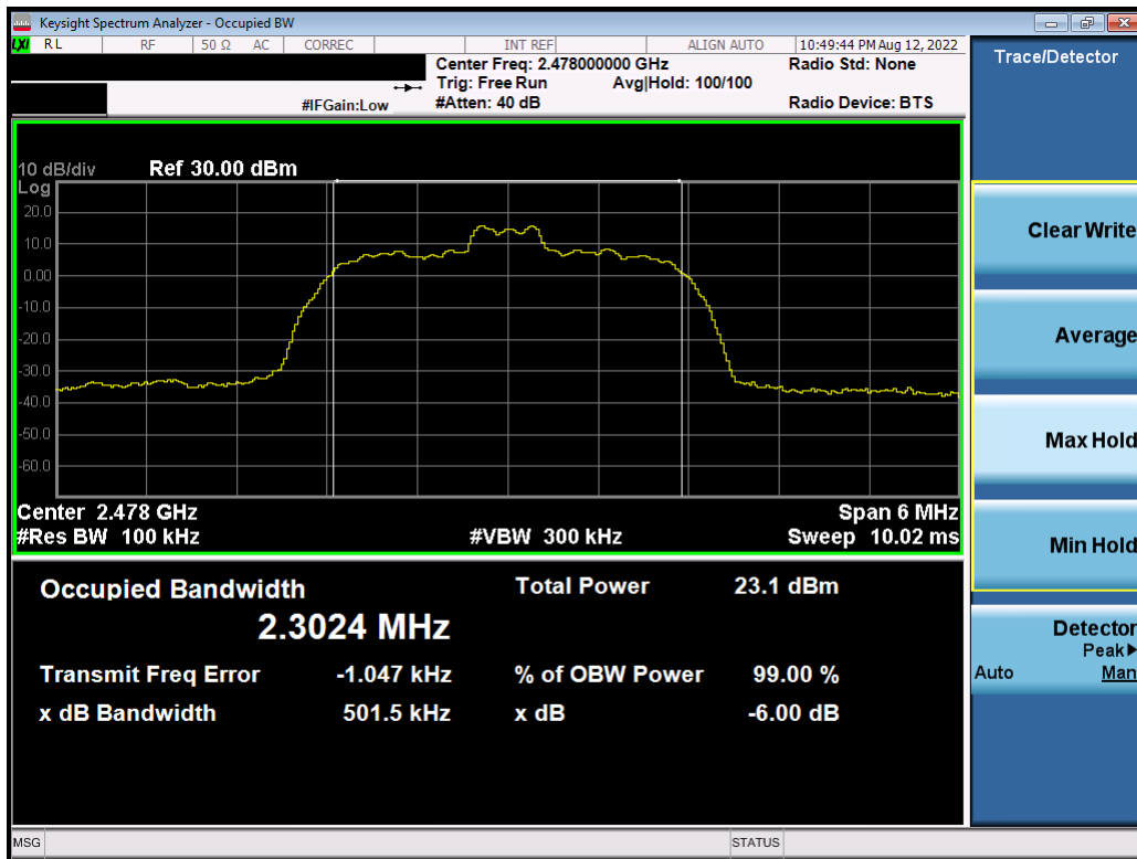
Plot 7-3. 6dB BW & 99% OBW Plot (Bluetooth (HDR4), 4Mbps – Ch. 75)
