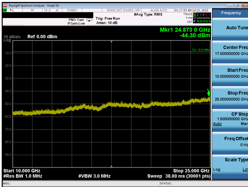
Plot 7-36. Conducted Spurious Plot (Bluetooth (HDRp8), 8 Mbps – Ch. 38)
