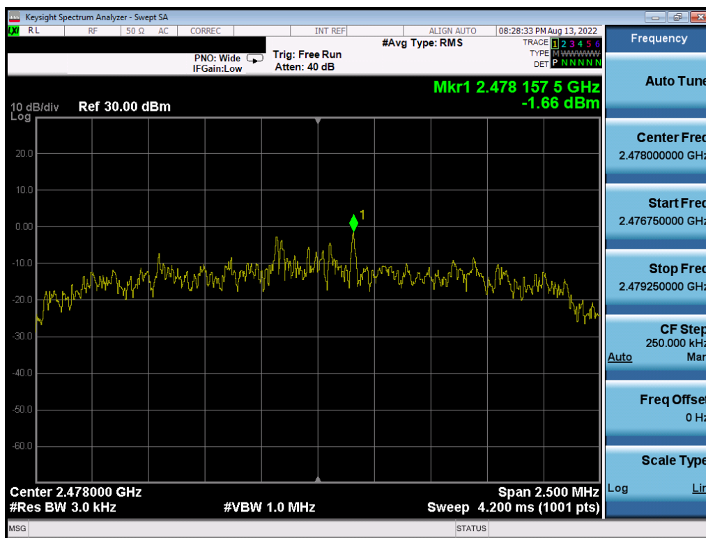
Plot 7-15. Power Spectral Density Plot (Bluetooth (HDR4), 4Mbps – Ch. 75)
