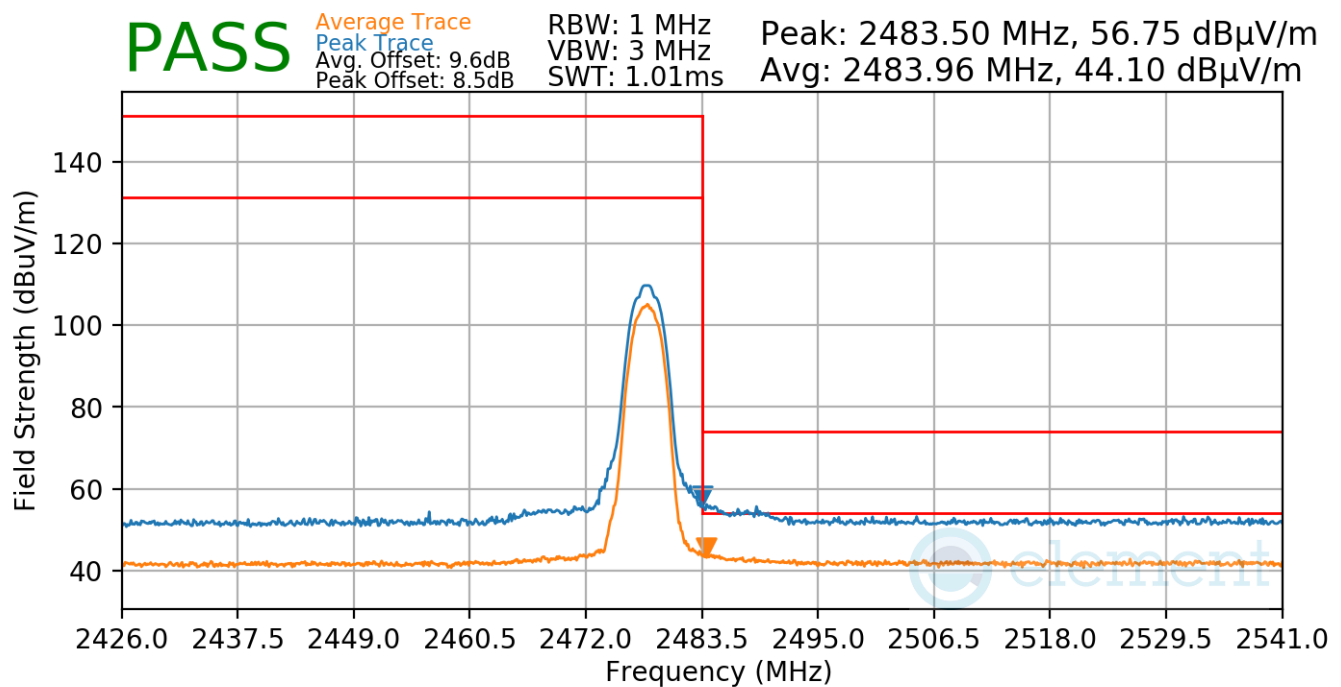
Plot 7-48. Radiated Restricted Upper Band Edge Measurement
