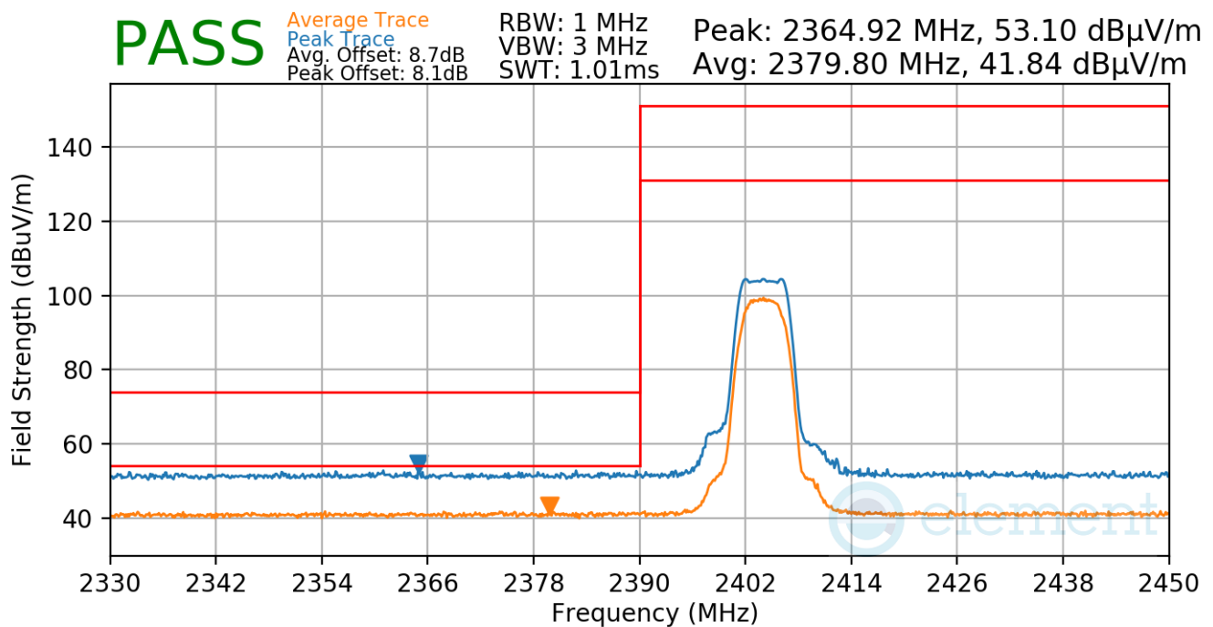
Plot 7-47. Radiated Restricted Lower Band Edge Measurement
