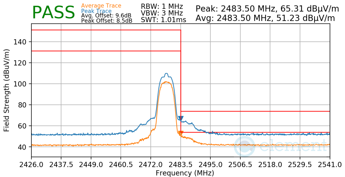
Plot 7-49. Radiated Restricted Upper Band Edge Measurement
