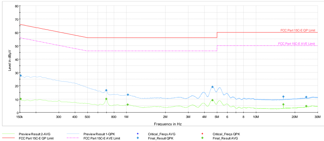
Plot 7-54. AC Line Conducted Plot with Bluetooth HDR (N, 4Mbps - Ch.38 with AC/DC Adapter)
