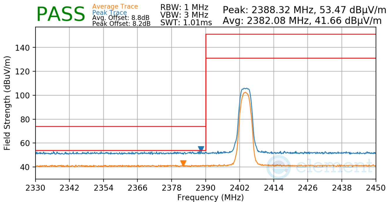
Plot 7-46. Radiated Restricted Lower Band Edge Measurement
