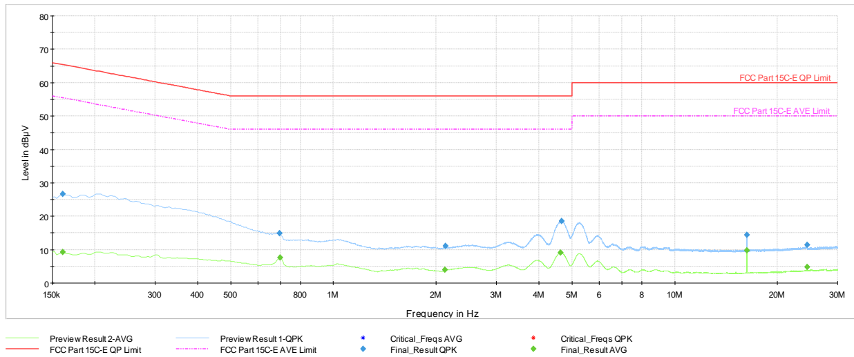
Plot 7-53. AC Line Conducted Plot with Bluetooth HDR (L1, 4Mbps - Ch.38 with AC/DC Adapter)
