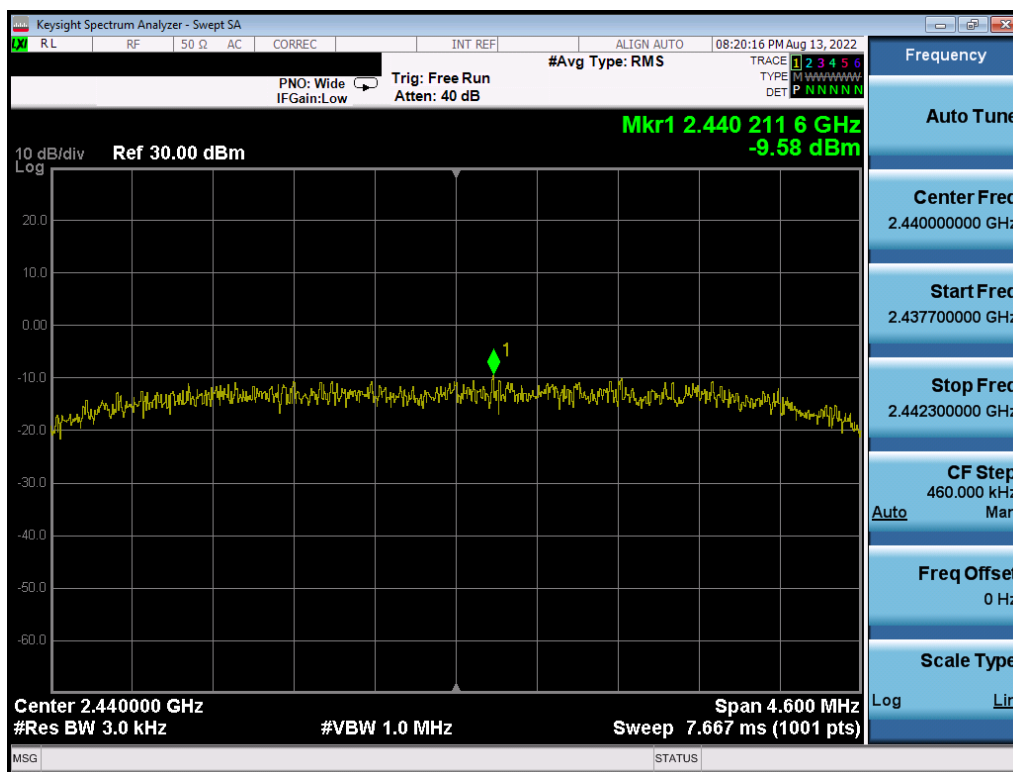
Plot 7-23. Power Spectral Density Plot (Bluetooth (HDRp8), 8Mbps – Ch. 38)
