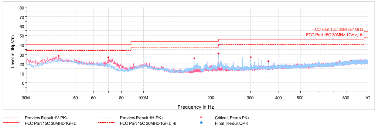
Plot 7-52. Radiated Spurious Emissions Below 1GHz (4Mbps – Ch.38 with AC/DC Adapter)
