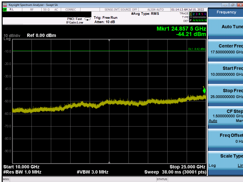
Plot 7-34. Conducted Spurious Plot (Bluetooth (HDP8), 8 Mbps – Ch. 1)
