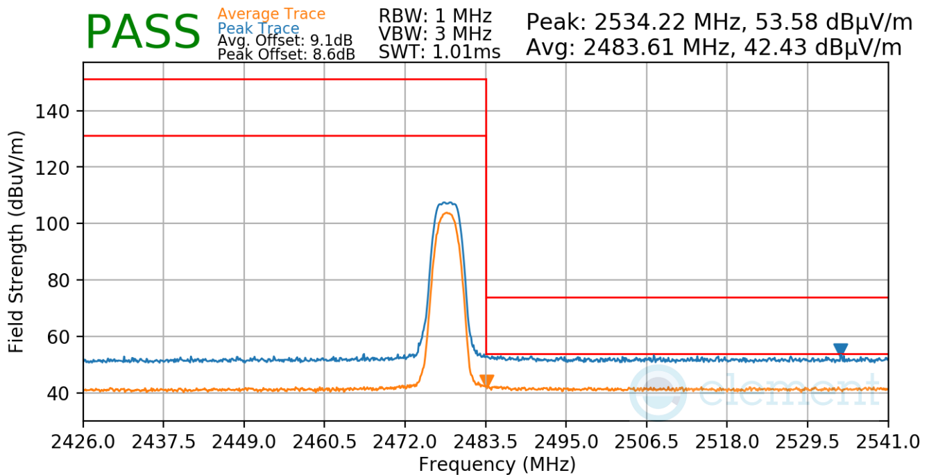
Plot 7-50. Radiated Restricted Upper Band Edge Measurement
