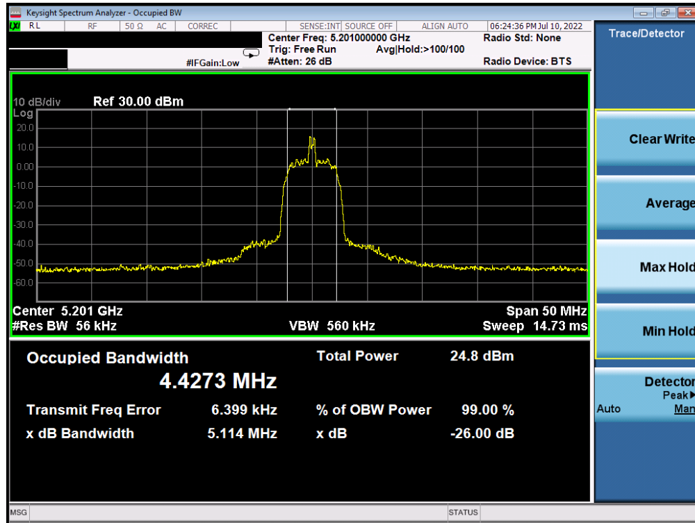
Plot 7-5. 26dB BW & 99% OBW (HDR8, 5201MHz)
