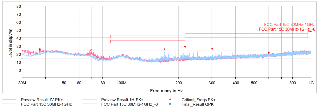
Plot 7-71. RSE 30MHz - 1GHz (HDR4 - 5201MHz), with AC/DC Adapter
