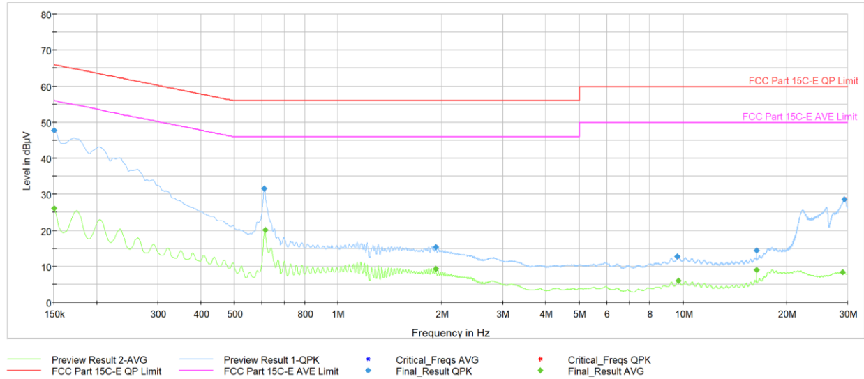
Plot 7-73. AC Line Conducted Plot (HDR4 – 5201MHz) (N) with host PC with Lightning Adapter
