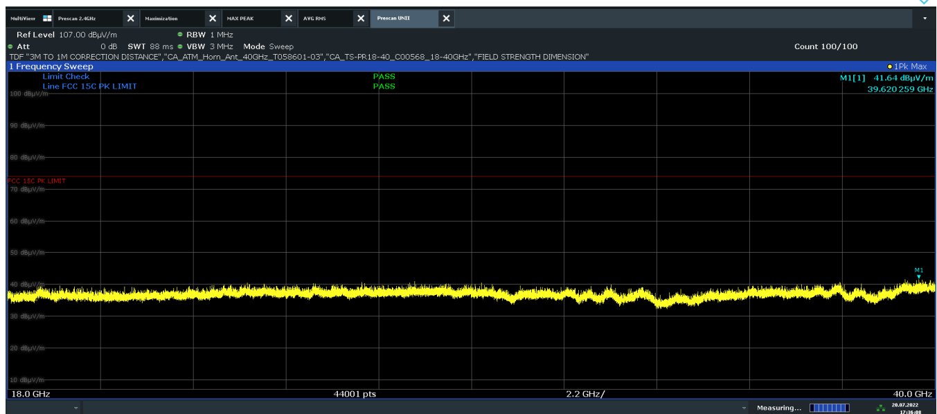
Plot 7-58. Radiated Spurious Emissions Above 18GHz (HDR4 – 5731MHz Pol. V)
