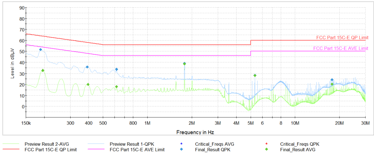
Plot 6-13. AC Line Conducted Plot (L1 - Mode 1, with Magnetic Charger & Laptop)
