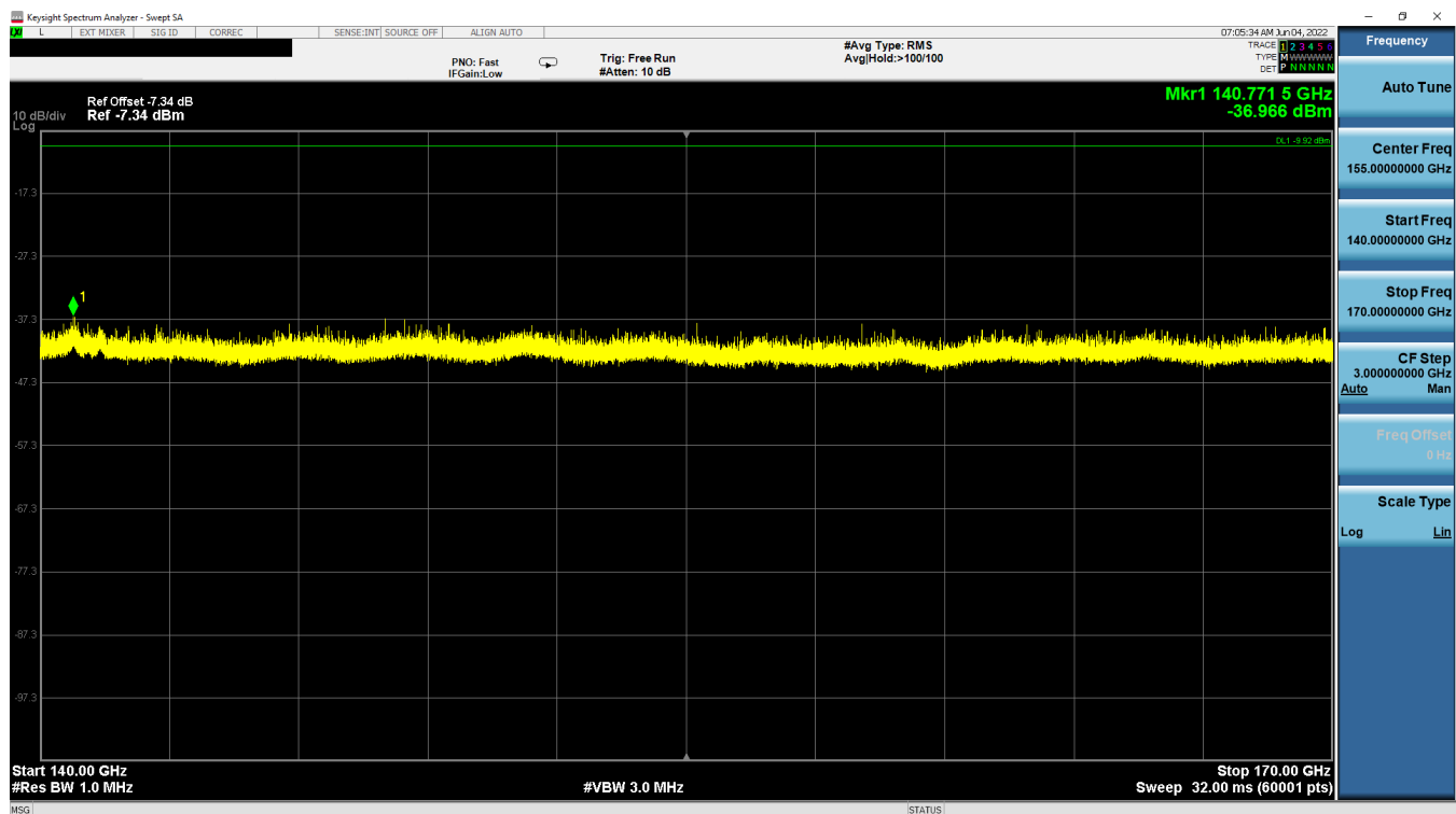
Plot 6-8. Radiated Spurious Emissions 140GHz – 170GHz (Mode1)
