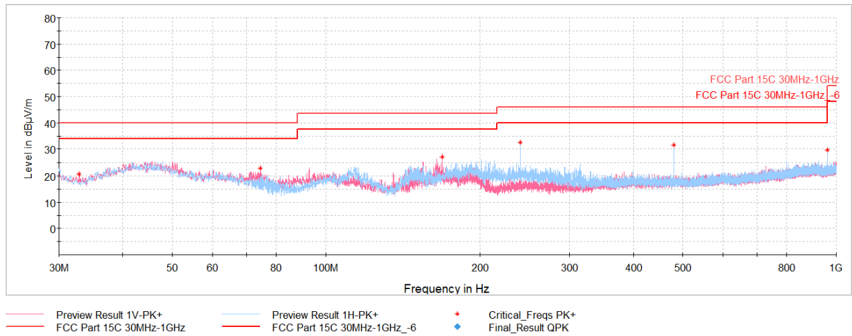
Plot 6-12. Radiated Spurious Emissions 30MHz – 1GHz (Mode 1, with Magnetic Charger & Laptop)
