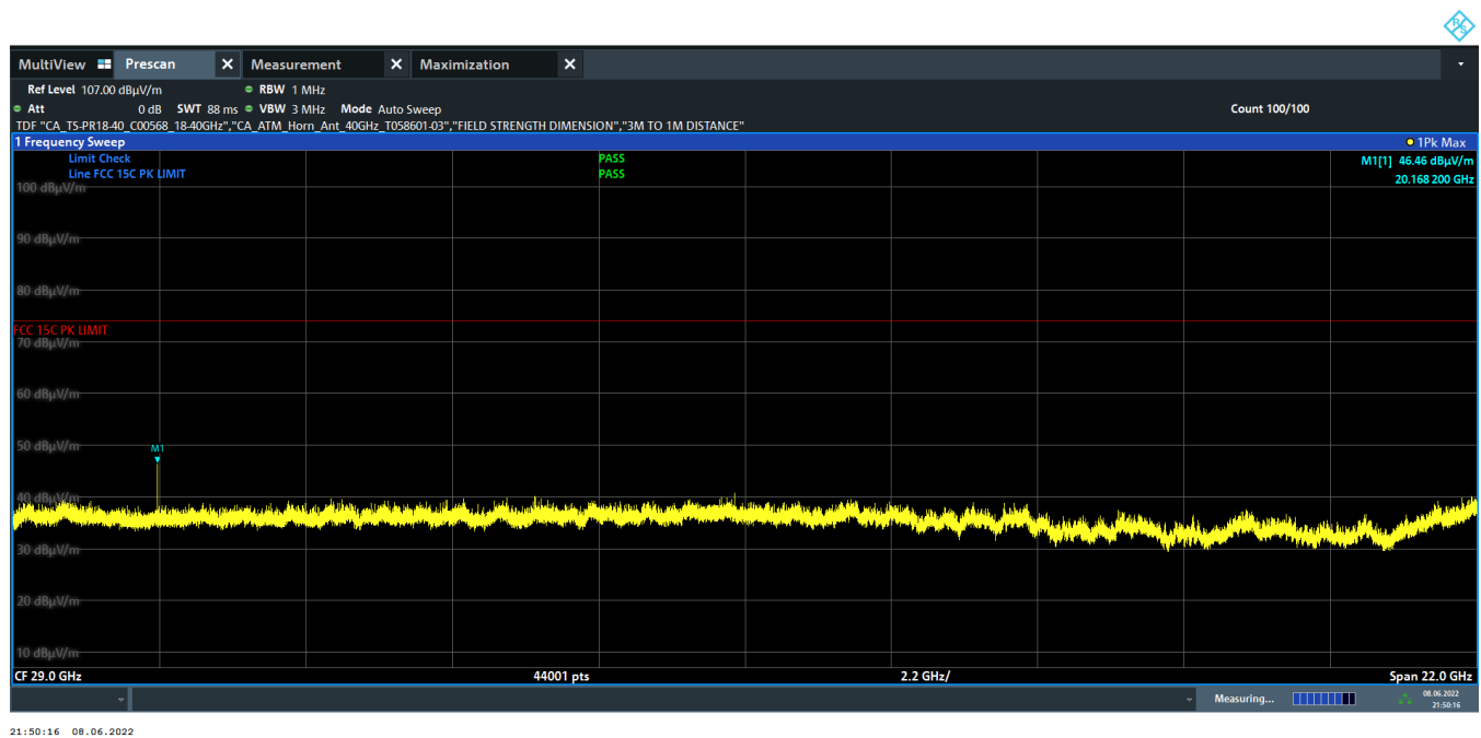
Plot 6-11. Radiated Spurious Emissions 18GHz – 40GHz (Mode 1)
