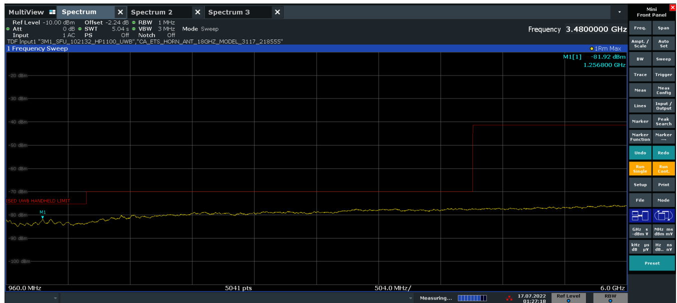
Plot 7-17. ISED Radiated Spurious Emission 960-6000MHz (Ch. 5, Config 0, Payload 125 Ant. Pol. H)
