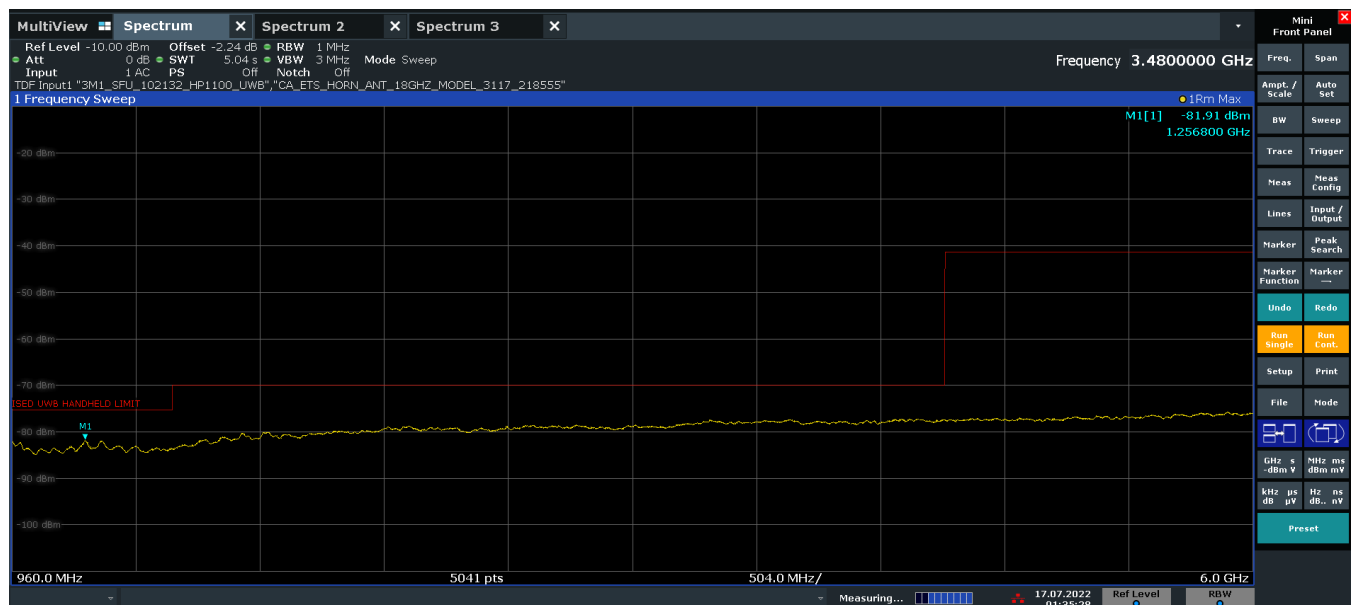
Plot 7-18. ISED Radiated Spurious Emission 960-6000MHz (Ch. 5, Config 0, Payload 125 Ant. Pol. V)
