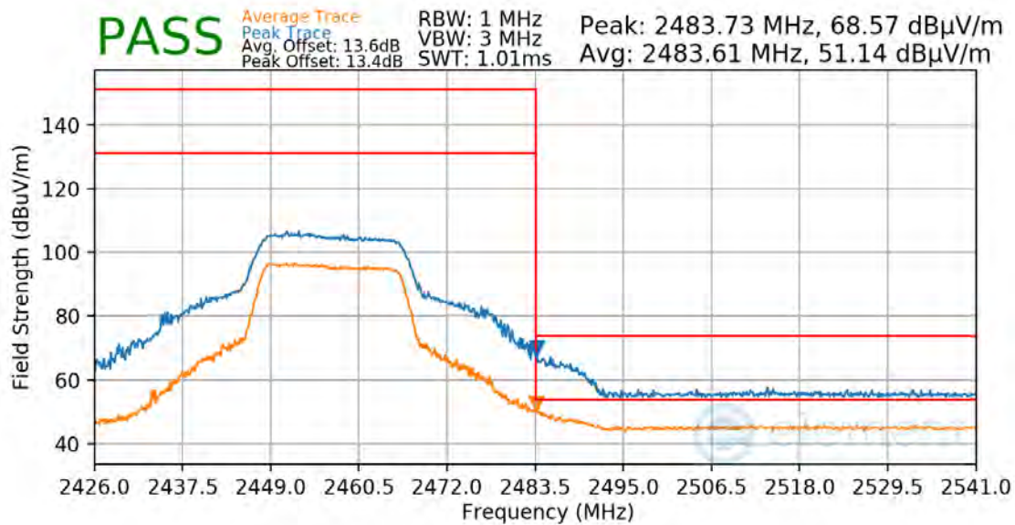
Plot 7-77. Radiated Restricted Upper Band Edge Measurement
