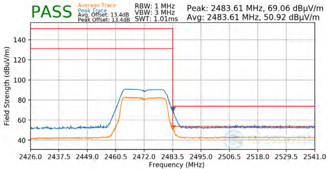
Plot 7-75. Radiated Restricted Upper Band Edge Measurement
