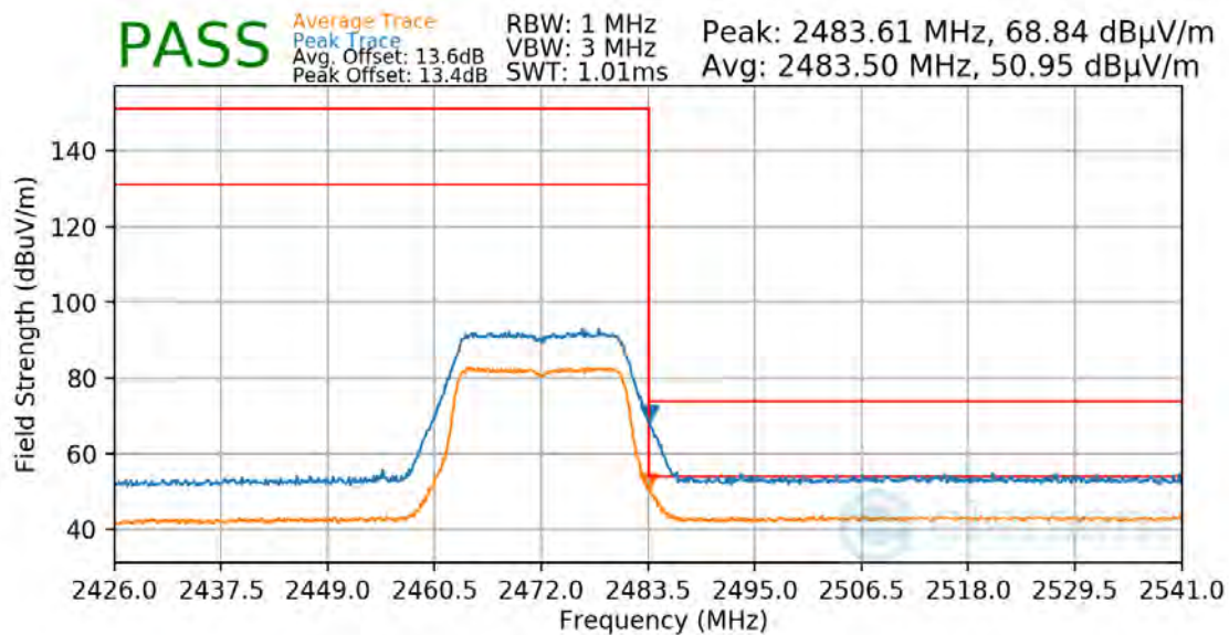
Plot 7-80. Radiated Restricted Upper Band Edge Measurement
