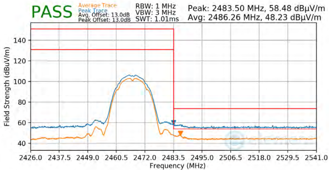
Plot 7-65. Radiated Restricted Upper Band Edge Measurement
