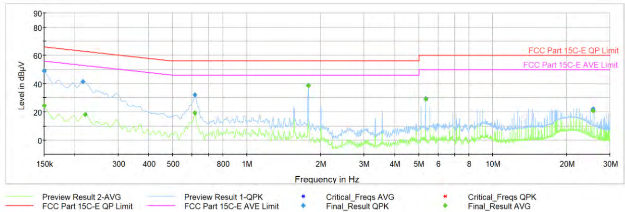
Plot 7-83. AC Line Conducted Plot 802.11b - Ch.6 (L1, with host PC and Magnetic charger)
