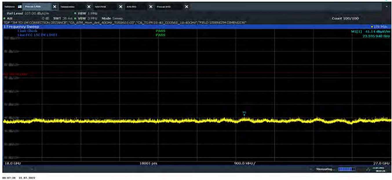
Plot 7-61. Radiated Spurious Plot Above 18GHz (802.11b – Ch. 6 Pol H)
