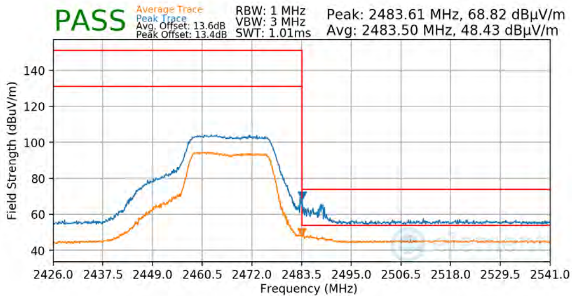
Plot 7-79. Radiated Restricted Upper Band Edge Measurement
