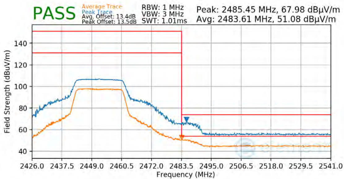
Plot 7-71. Radiated Restricted Upper Band Edge Measurement
