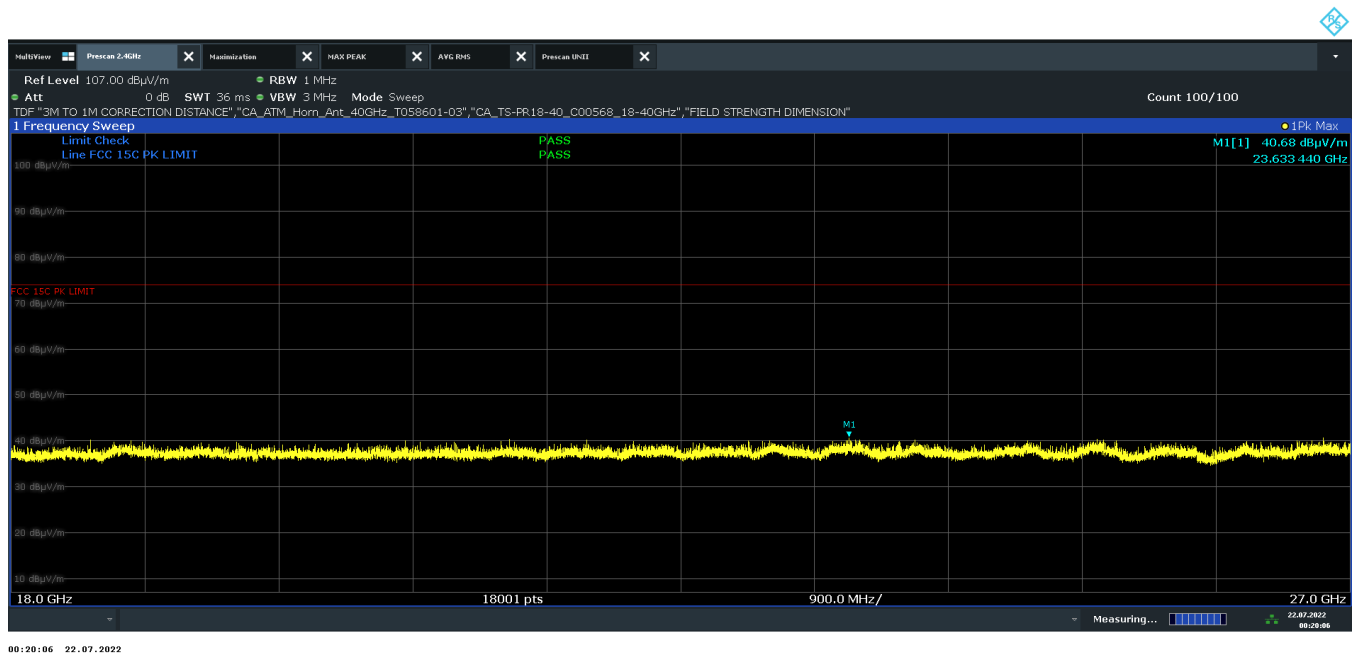
Plot 7-33. Radiated Spurious Emissions Above 18GHz (1Mbps ePA – Ch. 19, Pol. V)
