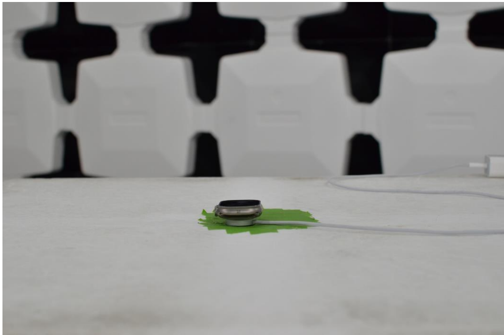
Figure 1: 1-18GHz Test Setup (Front View)
