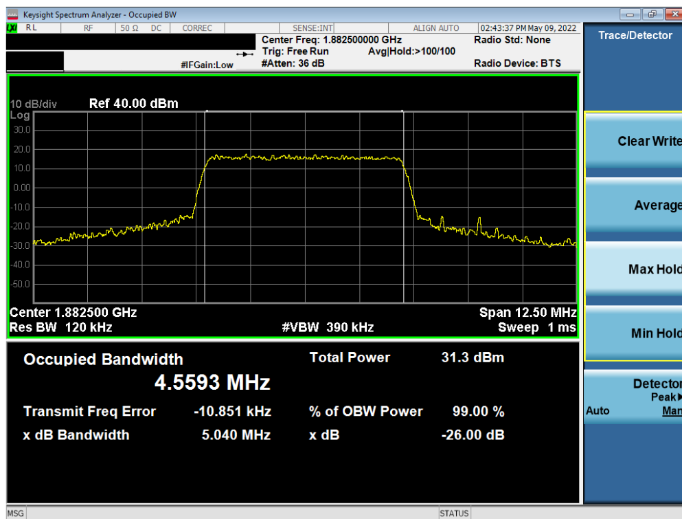
Plot 7-6. Occupied Bandwidth Plot (LTE Band 25/2 - 5MHz 16-QAM - Full RB Configuration)
