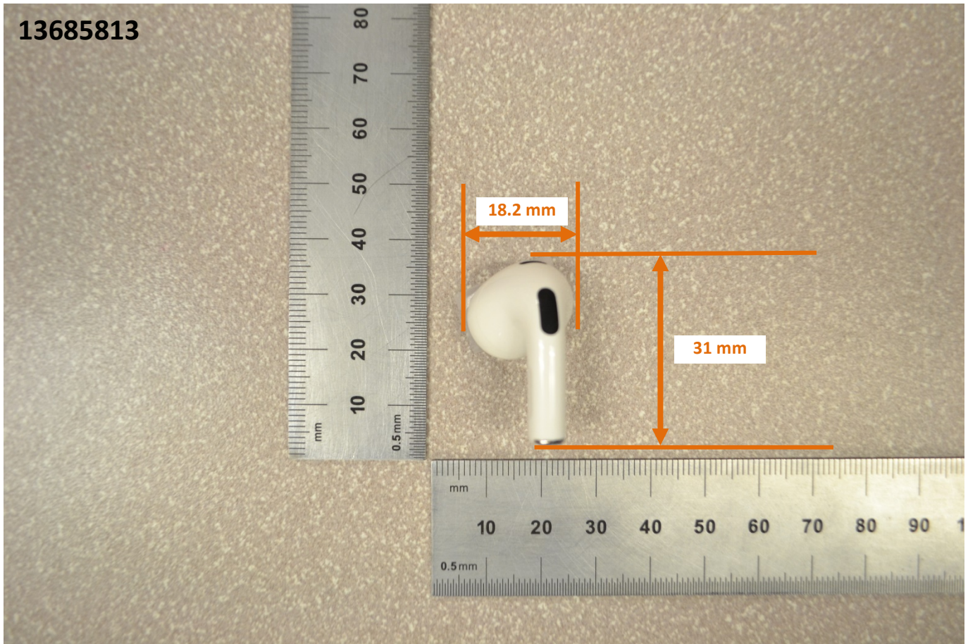
Photograph 1: Overall Dimensions
