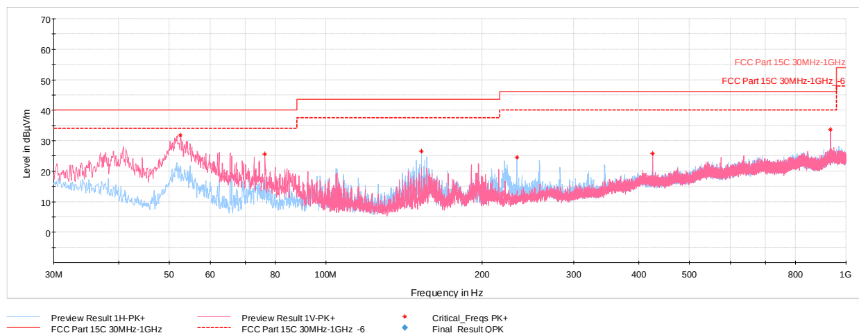
Plot 6-12. Radiated Spurious Emissions 30MHz – 1GHz (Mode 1, with AC/DC Adapter + Magnetic Charger)
