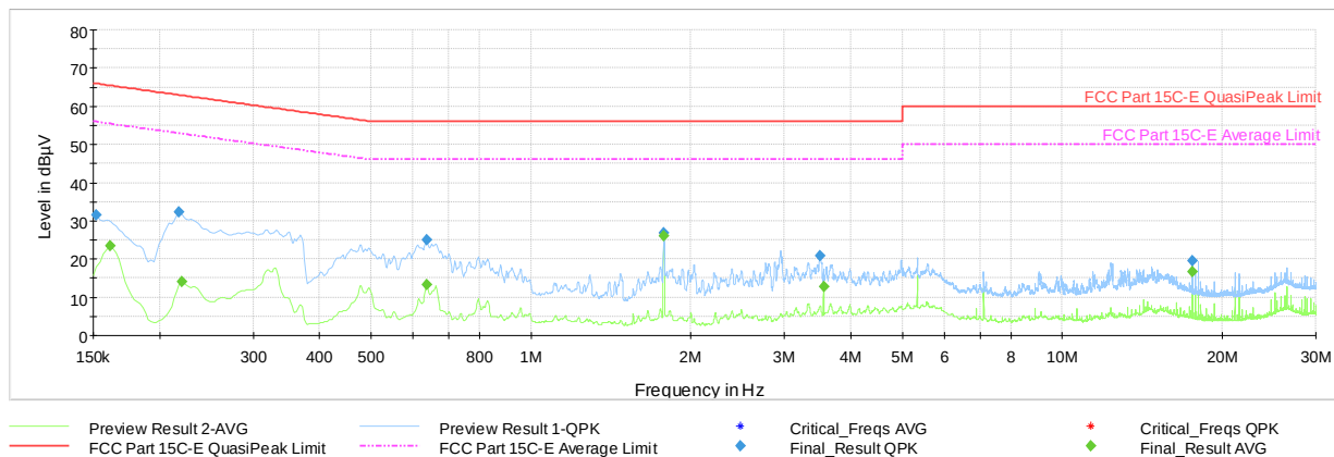
Plot 6-13. AC Line Conducted Plot (L1 - Mode 1, with AC/DC Adapter + Magnetic Charger)
