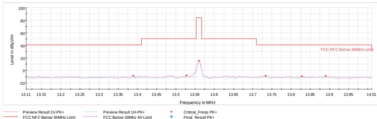
Plot 7-6. In Band Radiated Spurious Emissions (CE A 848kbps, with AC/DC Adapter and Magnetic Charger)
