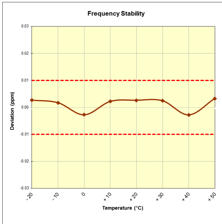
Figure 7-4. Frequency Stability Plot (Reader 10% ASK 1 out of 256)
