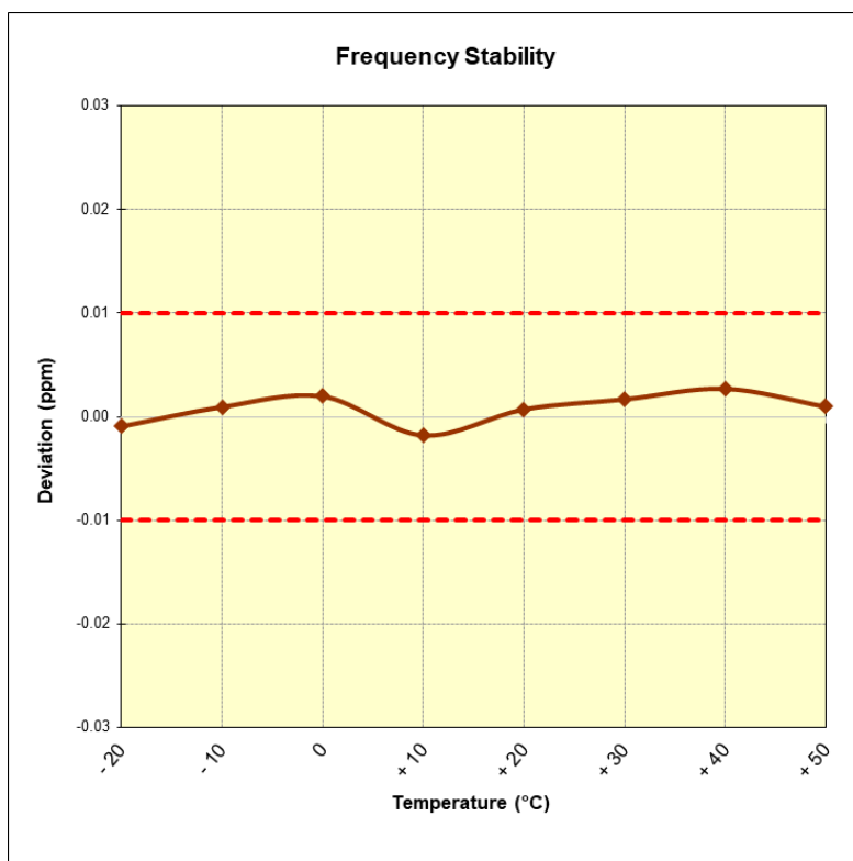
Figure 7-3. Frequency Stability Plot (CE A 848kbps)
