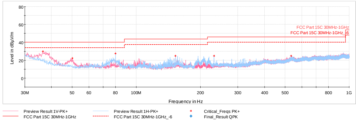
Plot 7-10. Radiated Spurious Emissions 30MHz – 1GHz (CE A 848kbps, with AC/DC Adapter and Magnetic Charger)
