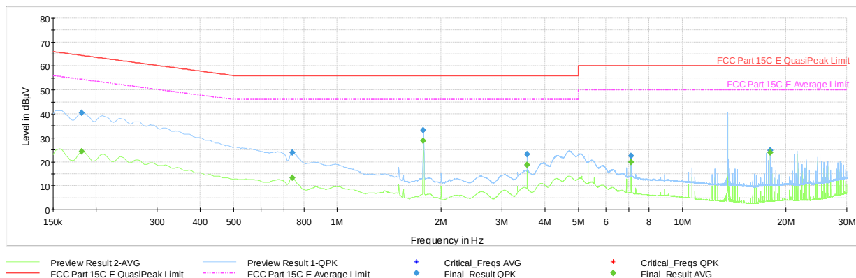
Plot 7-14. AC Line-Conducted Plot (L1, Reader 10% ASK 1 out of 256, with AC/DC Adapter and Magnetic Charger)
