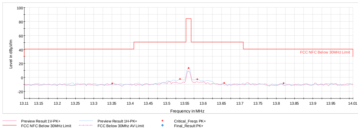
Plot 7-7. In Band Radiated Spurious Emissions (Reader 10% ASK 1 out of 256, AC/DC Adapter and Magnetic Charger)
