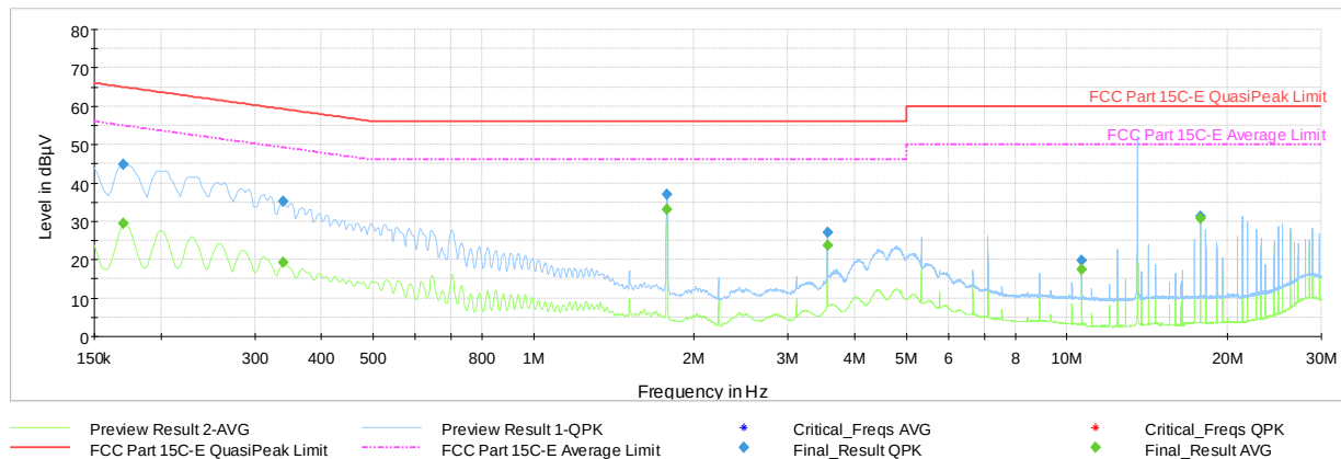
Plot 7-12. AC Line-Conducted Plot (L1, CE A 848kbps, with AC/DC Adapter and Magnetic Charger)
