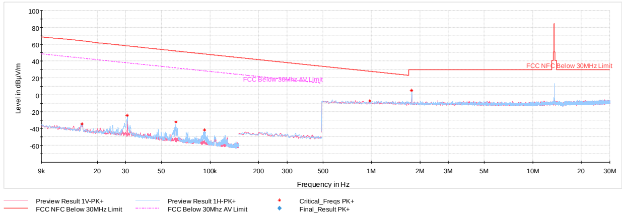
Plot 7-9. Radiated Spurious Emissions 9kHz – 30MHz (Reader 10% ASK 1 out of 256, with AC/DC Adapter and Magnetic Charger)
