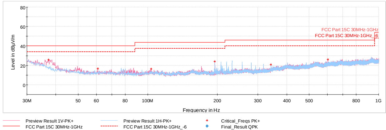
Plot 7-11. Radiated Spurious Emissions 30MHz – 1GHz (Reader 10% ASK 1 out of 256, with AC/DC Adapter and Magnetic Charger)
