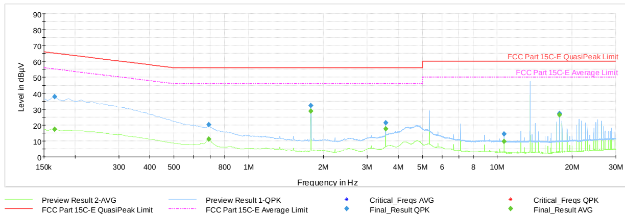
Plot 7-13. AC Line-Conducted Plot (N, CE A 848kbps, with AC/DC Adapter and Magnetic Charger)
