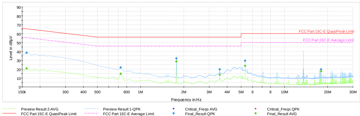
Plot 7-15. AC Line-Conducted Plot (N, Reader 10% ASK 1 out of 256, with AC/DC Adapter and Magnetic Charger)
