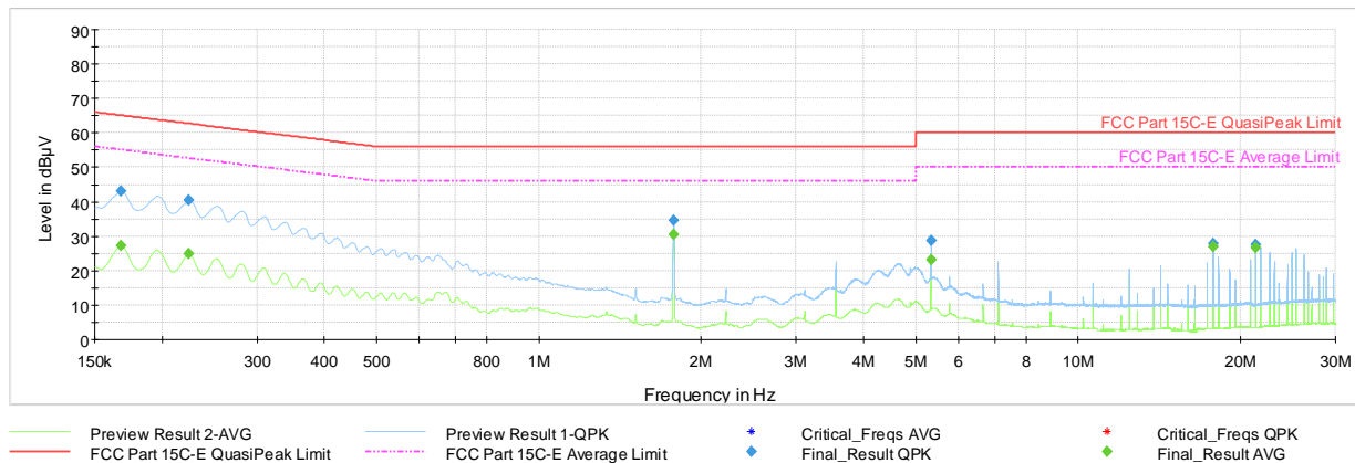
Plot 7-42. AC Line Conducted (Ch. 5, Config 3, Payload 125 N, with AC/DC Adapter + Magnetic Charger)
