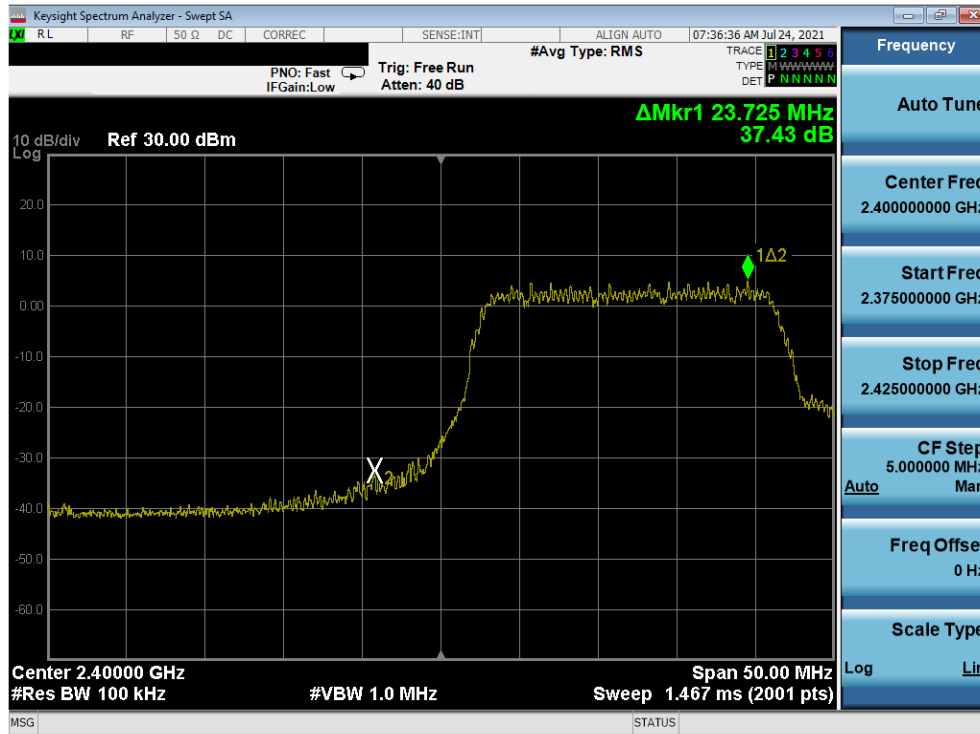
Plot 7-45. Band Edge Plot (802.11n MCS7 – Ch. 1)
