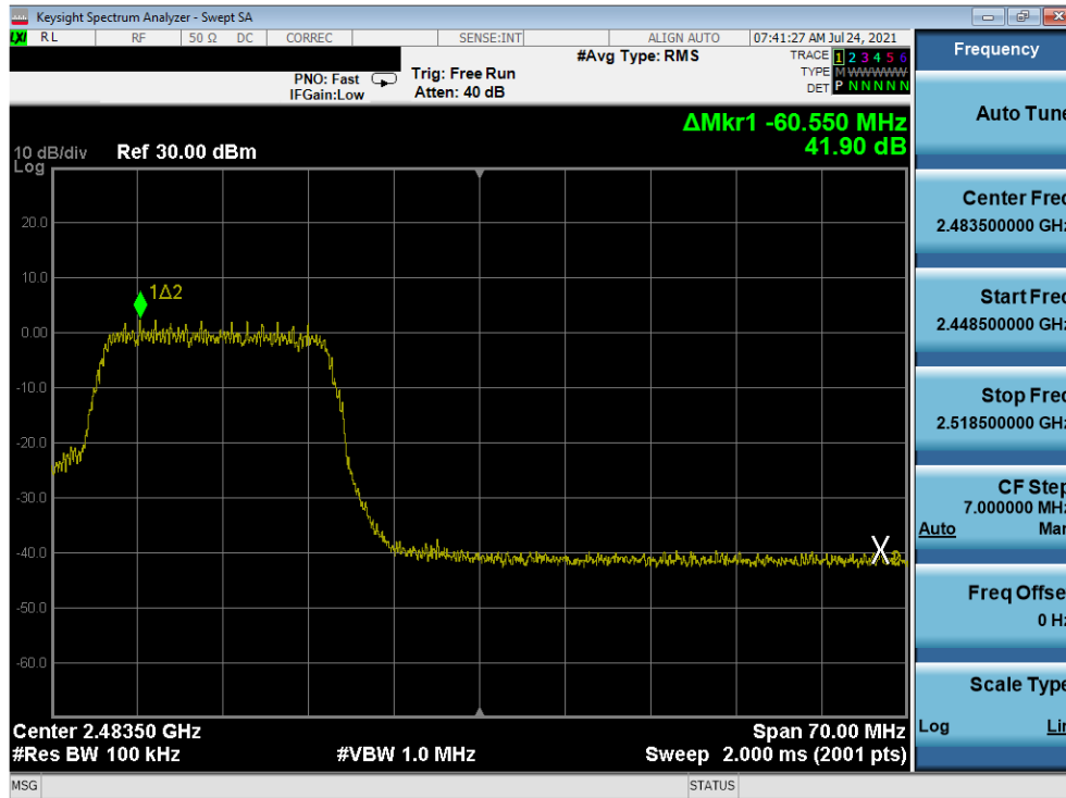
Plot 7-47. Band Edge Plot (802.11n MCS7 – Ch. 11)
