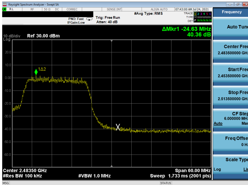
Plot 7-48. Band Edge Plot (802.11n MCS7 – Ch. 12)
