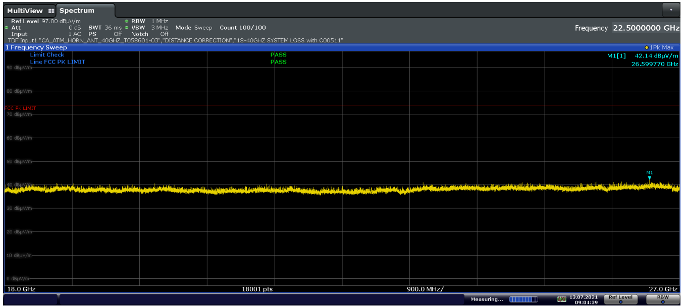
Plot 7-59. Radiated Spurious Plot above 18GHz (802.11b – Ch. 11 Pol H)
