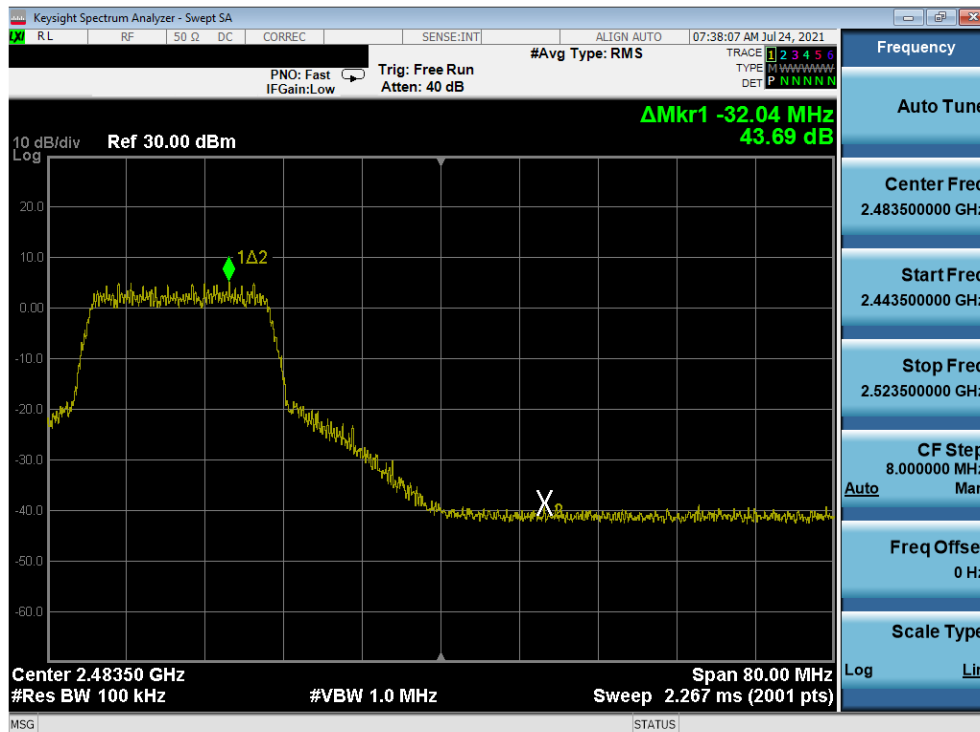
Plot 7-46. Band Edge Plot (802.11n MCS7 – Ch. 10)
