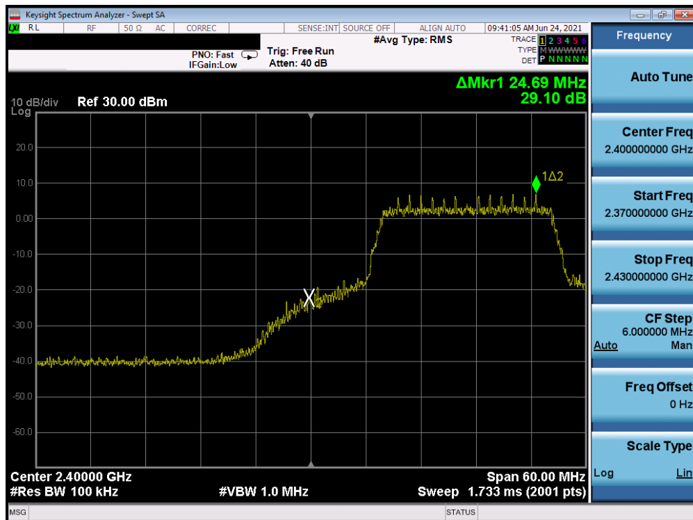
Plot 7-38. Band Edge Plot (802.11n MCS0 – Ch. 2)
