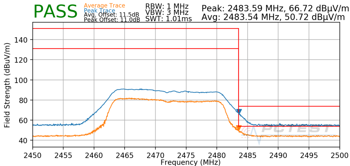
Plot 7-77. Radiated Restricted Upper Band Edge Measurement
