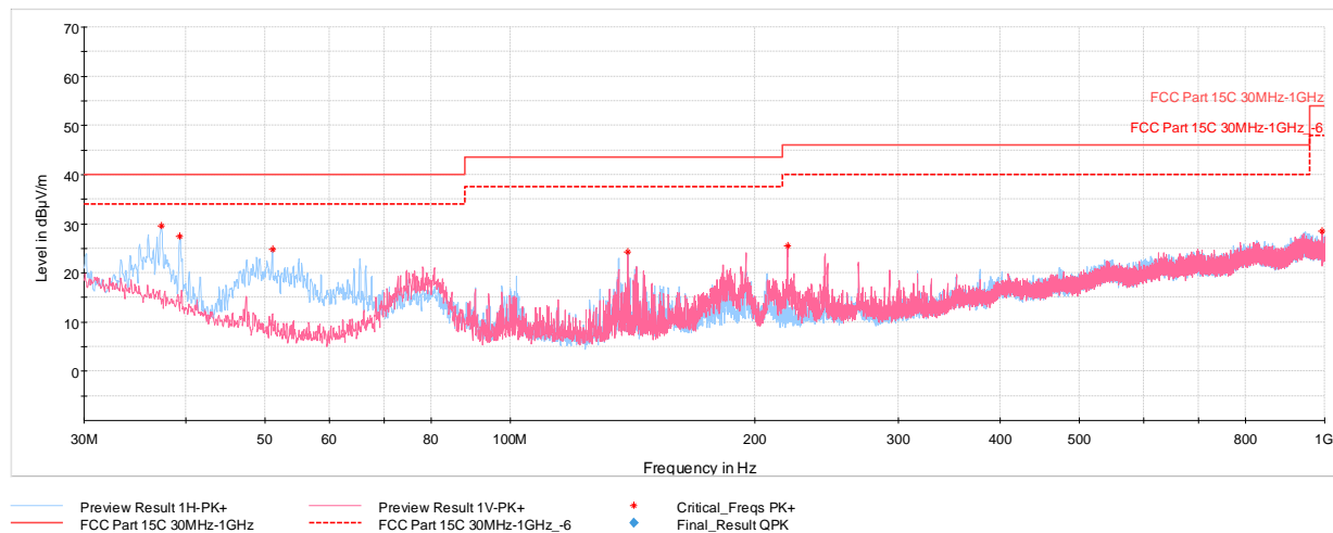
Plot 7-78. Radiated Spurious Emissions 30MHz-1GHz 802.11b – Ch.11, with AC/DC Adapter and Magnetic Charger
