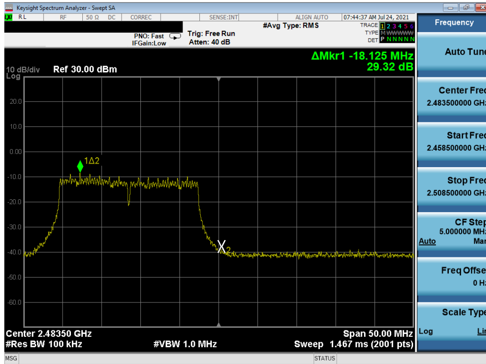
Plot 7-49. Band Edge Plot (802.11n MCS7 – Ch. 13)
