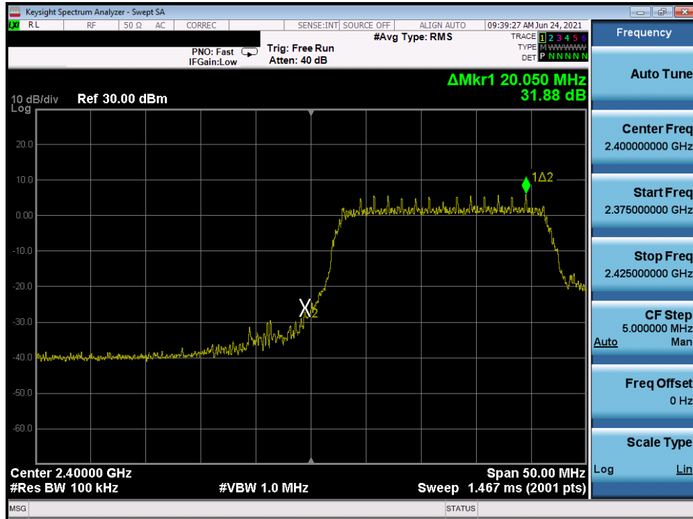
Plot 7-37. Band Edge Plot (802.11n MCS0 – Ch. 1)
