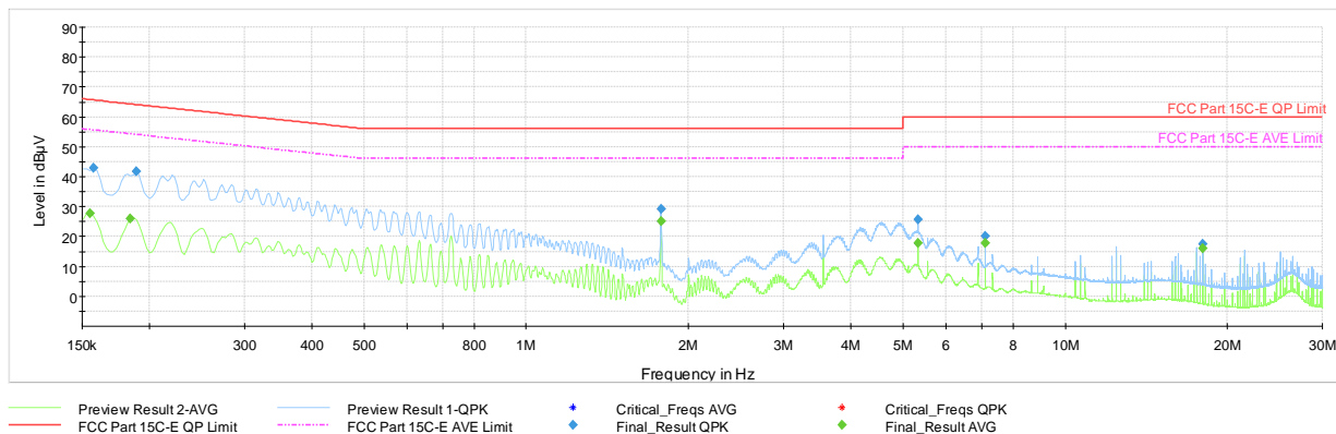
Plot 7-80. AC Line Conducted Plot 802.11b – Ch.11 (N), with AC/DC Adapter and Magnetic Charger
