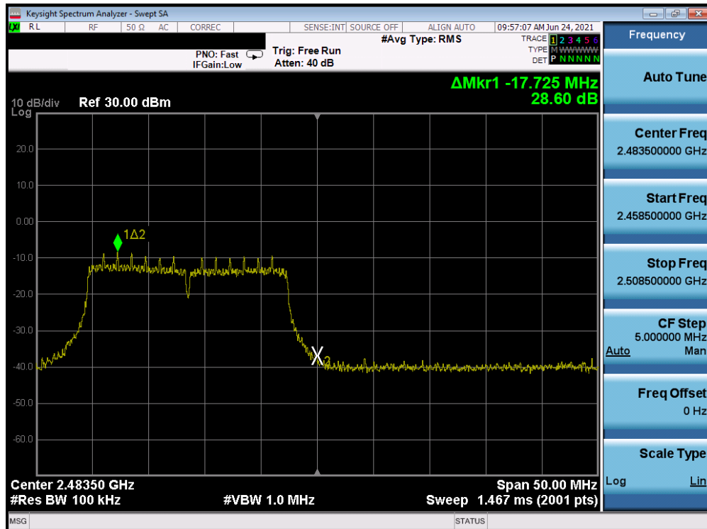
Plot 7-44. Band Edge Plot (802.11n MCS0 – Ch. 13)
