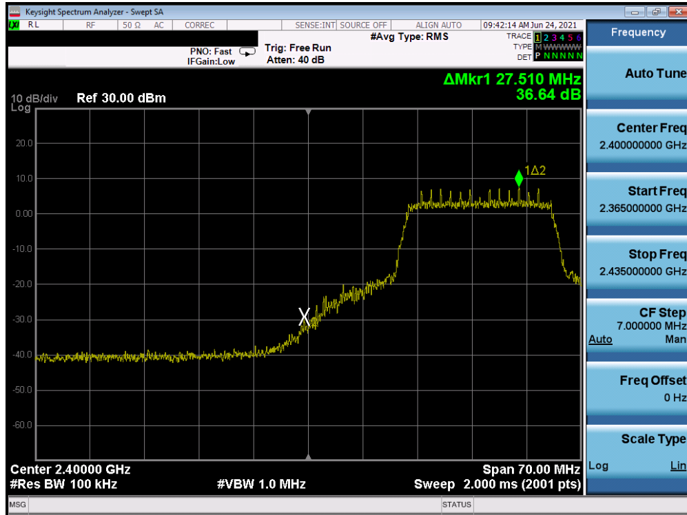
Plot 7-39. Band Edge Plot (802.11n MCS0 – Ch. 3)
