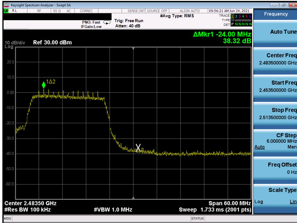
Plot 7-43. Band Edge Plot (802.11n MCS0 – Ch. 12)
