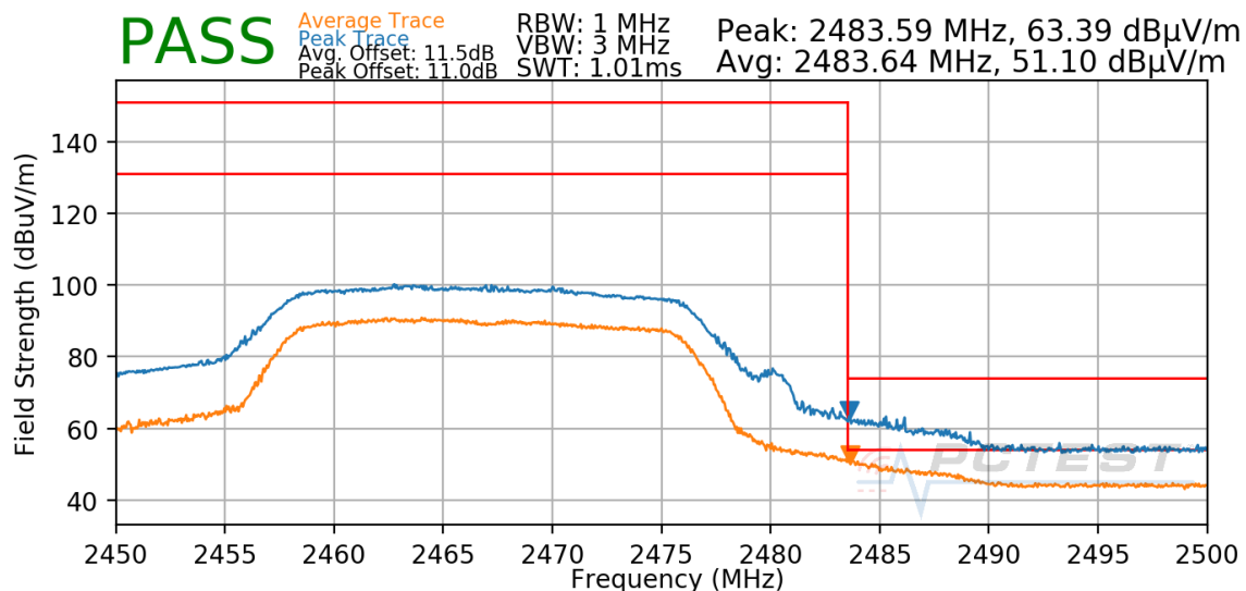
Plot 7-76. Radiated Restricted Upper Band Edge Measurement
