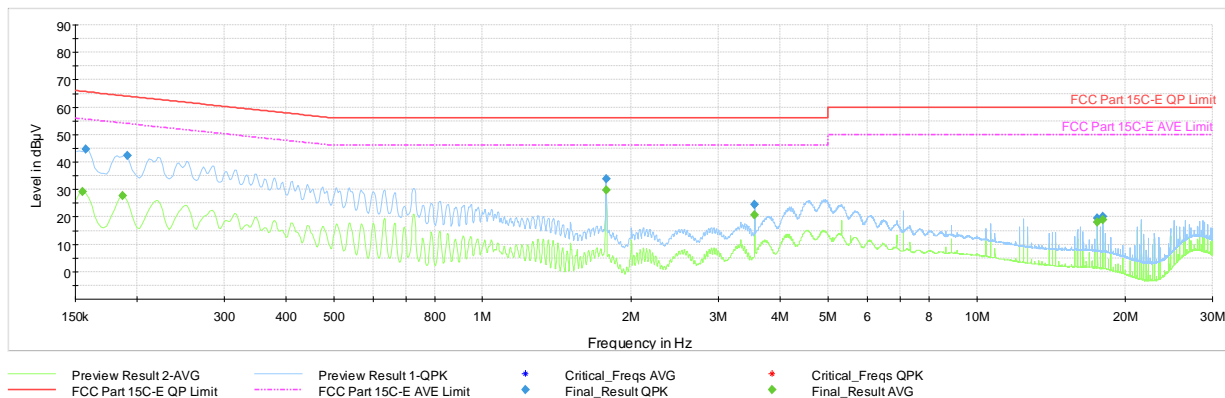
Plot 7-79. AC Line Conducted Plot 802.11b – Ch.11 (L1), with AC/DC Adapter and Magnetic Charger
