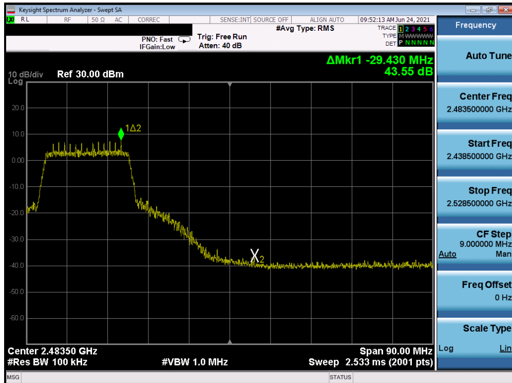
Plot 7-40. Band Edge Plot (802.11n MCS0 – Ch. 9)
