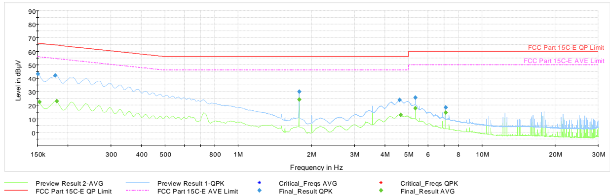
Plot 7-40. AC Line Conducted Emissions with Bluetooth LE (1Mbps, ePA – Ch.19, N, with AC/DC Adapter + Magnetic Charger)
