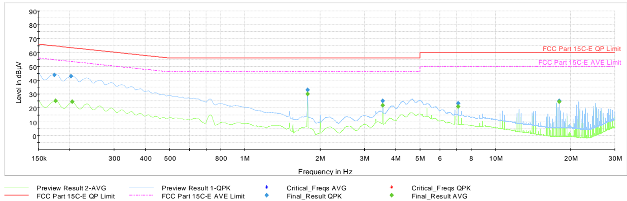
Plot 7-39. AC Line Conducted Emissions with Bluetooth LE (1Mbps, ePA – Ch.19, L1, with AC/DC Adapter + Magnetic Charger)
