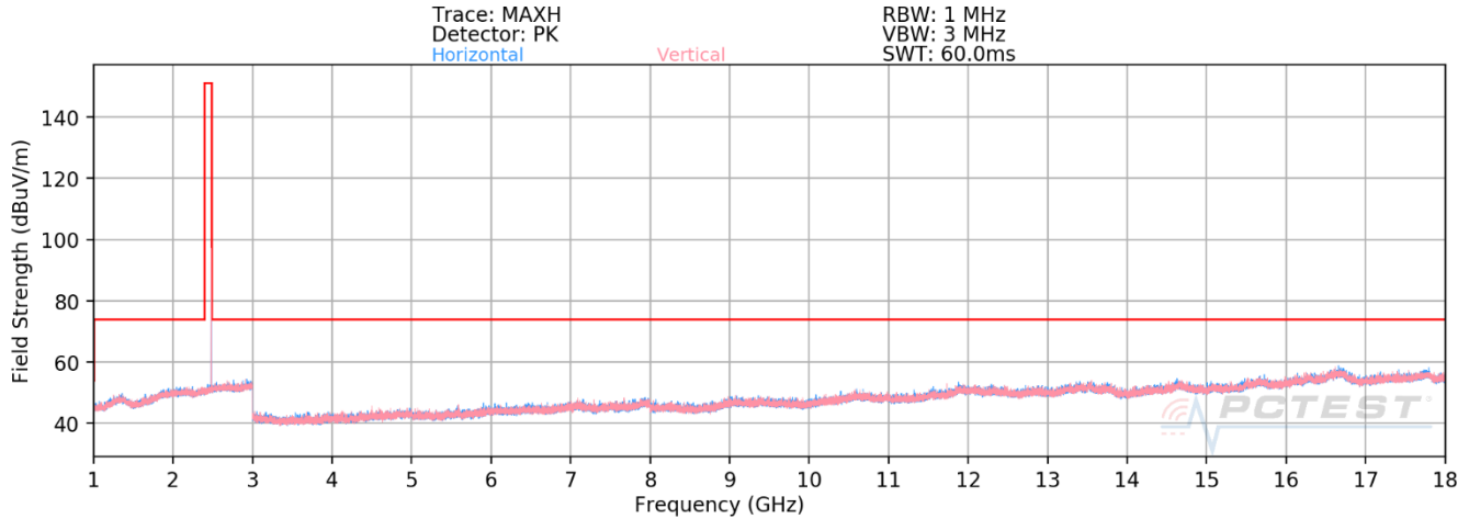
Plot 7-31. Radiated Spurious Emissions Above 1GHz (1Mbps ePA – Ch. 39, Ant. Pol. H & V)
