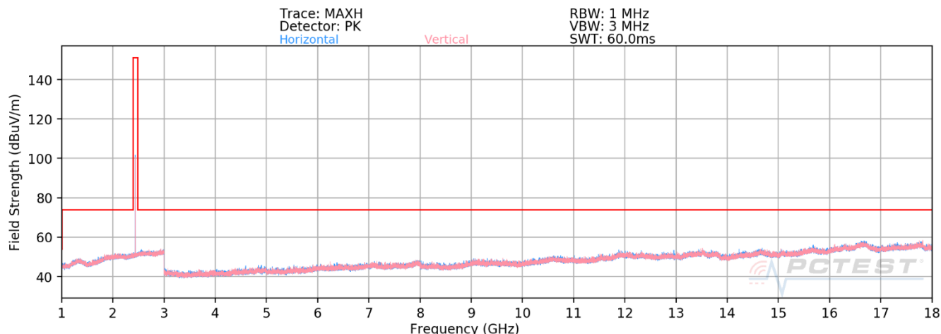
Plot 7-30. Radiated Spurious Emissions Above 1GHz (1Mbps, ePA – Ch. 19, Ant. Pol. H & V)
