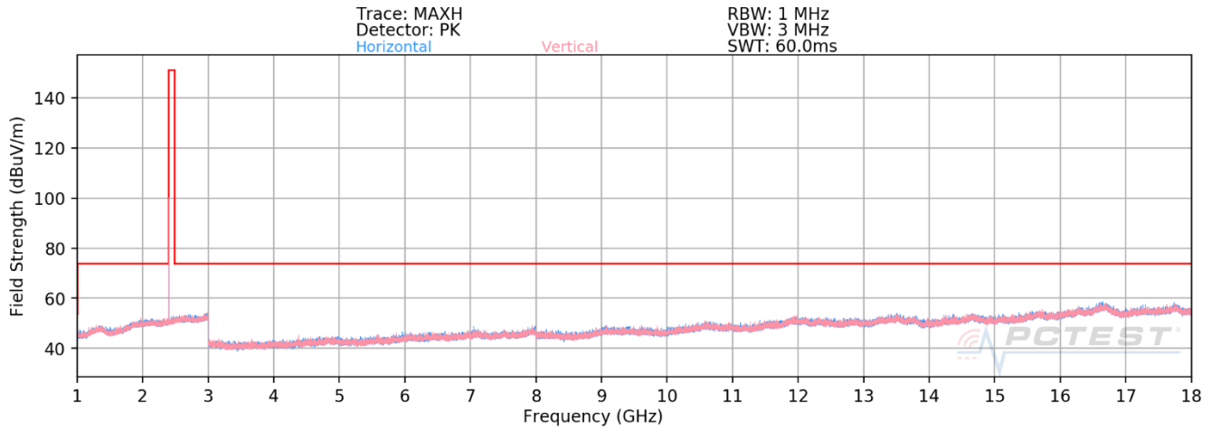
Plot 7-29. Radiated Spurious Emissions Above 1GHz (1Mbps, ePA – Ch. 0, Ant. Pol. H & V)
