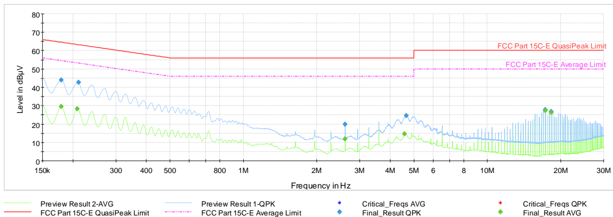
Plot 7-39. AC Line Conducted Emissions with Bluetooth HDR (L1, 4Mbps ePA – Ch.38 with AC/DC Adapter + Magnetic Charger)
