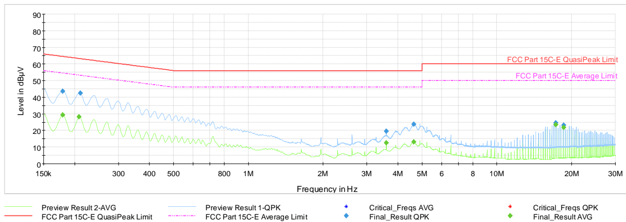
Plot 7-40. AC Line Conducted Emissions with Bluetooth HDR (N, 4Mbps ePA – Ch.38 with AC/DC Adapter + Magnetic Charger)
