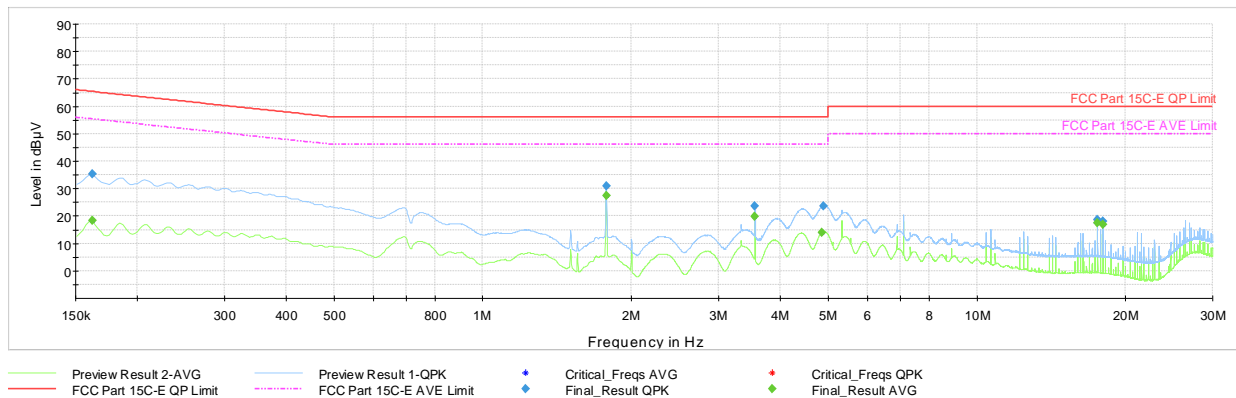
Plot 7-60. AC Line Conducted Plot with 802.11n UNII Band 2C – Ch.144 (L1) with AC/DC Adaptor & Magnetic Charger
