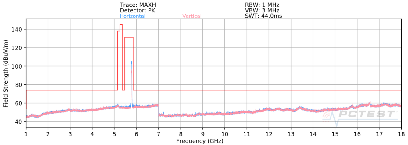
Plot 7-37. Radiated Spurious Emissions above 1GHz (802.11n – UNII 3 Ch. 157)
