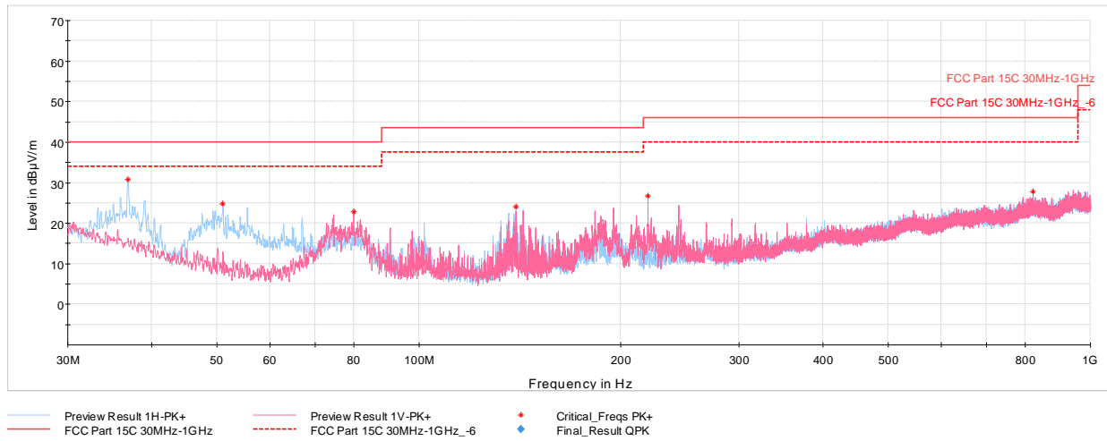
Plot 7-58. Radiated Spurious Emissions below 1GHz (802.11n – UNII 2C Ch. 144) with AC/DC Adaptor & Magnetic Charger
