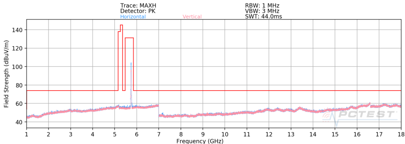
Plot 7-36. Radiated Spurious Emissions above 1GHz (802.11n – UNII 3 Ch. 149)
