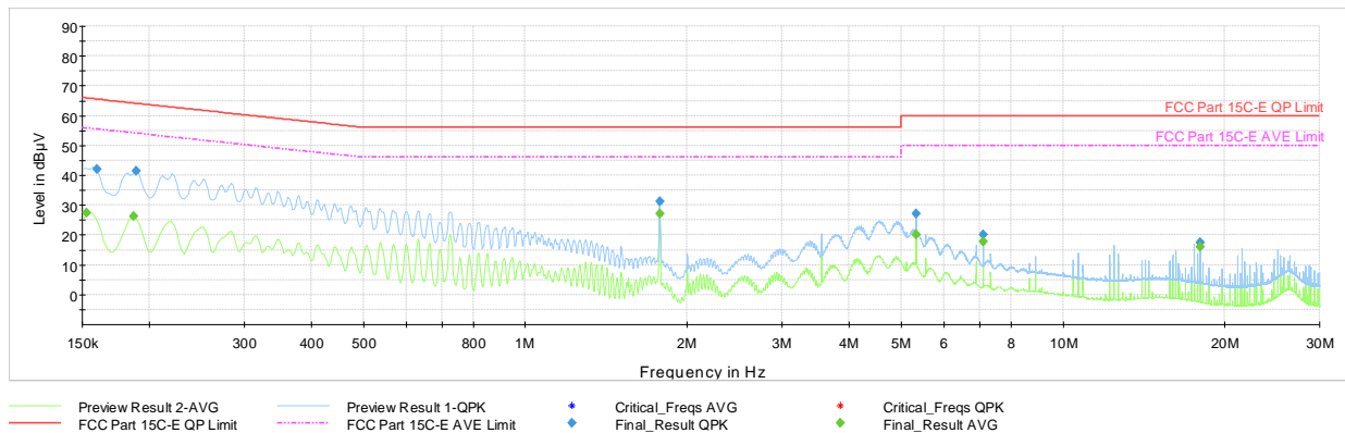
Plot 7-61. AC Line Conducted Plot with 802.11n UNII Band 2C – Ch.144 (N) with AC/DC Adaptor & Magnetic Charger
