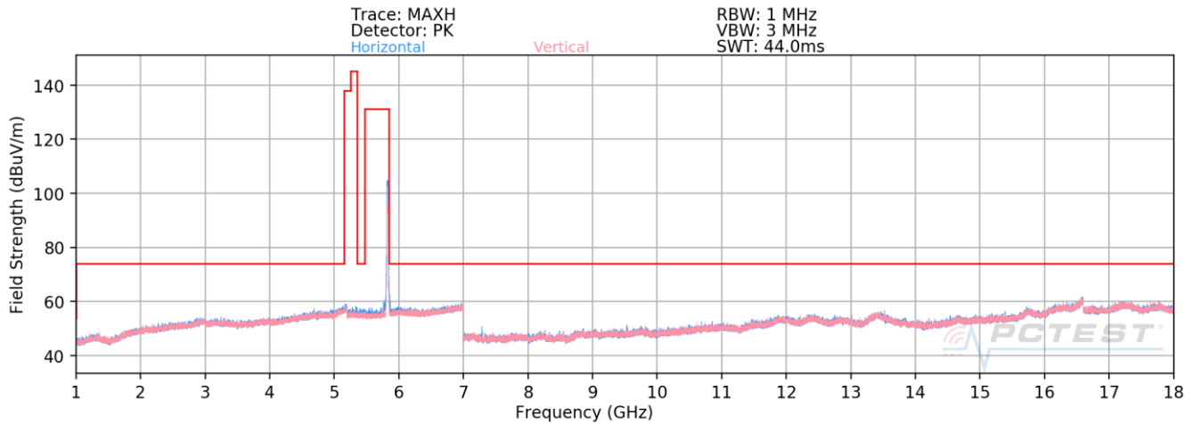
Plot 7-38. Radiated Spurious Emissions above 1GHz (802.11n – UNII 3 Ch. 165)
