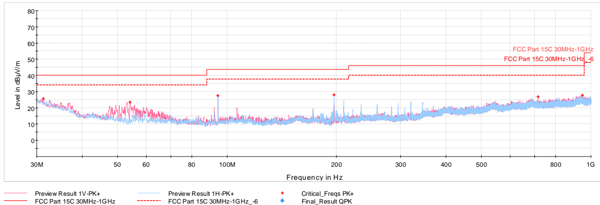
Plot 7-59. Radiated Spurious Emissions – Simultaneous Transmission below 1GHz with AC/DC Adaptor & Magnetic Charger
