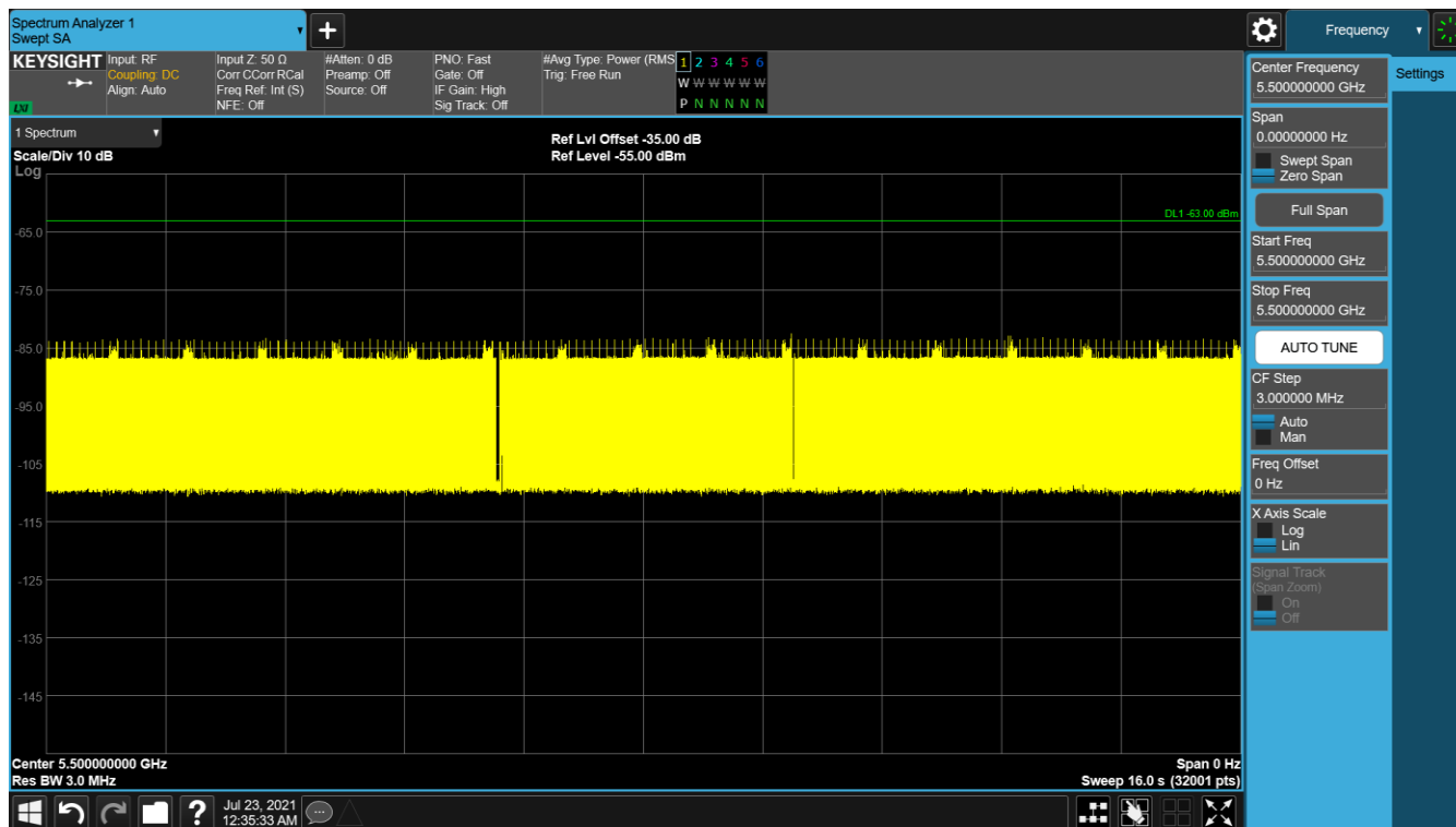
Figure 9-1. 5500MHz - Channel Loading - (20MHz)
