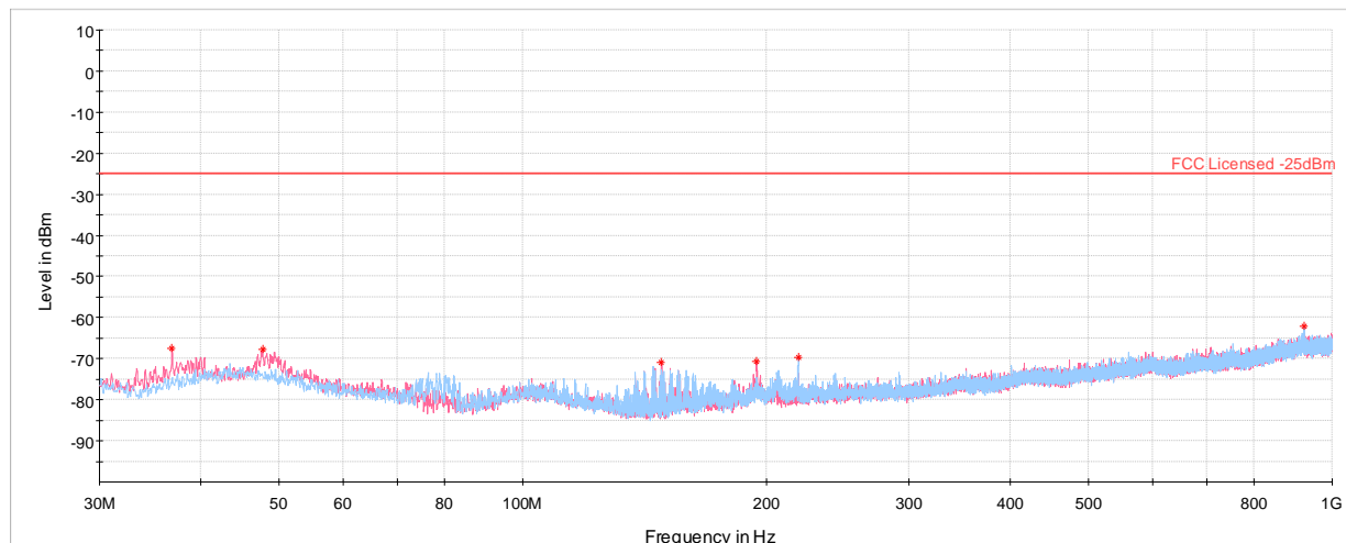
Plot 7-57. Radiated Spurious Emissions – Simultaneous Transmission 30MHz – 1GHz
