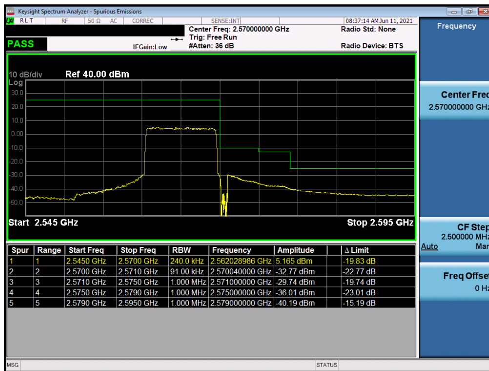
Plot 7-38. Upper ACP Plot (LTE Band 7 - 10MHz QPSK – Full RB)
