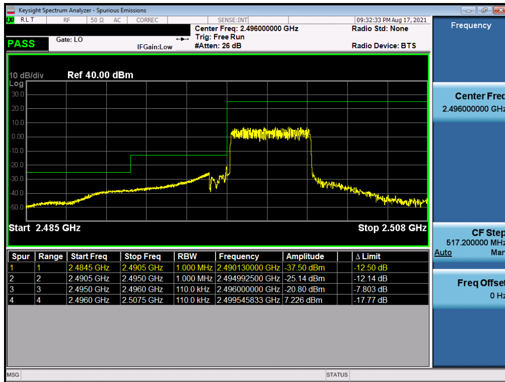
Plot 7-43. Lower ACP Plot (LTE Band 41 - 5MHz QPSK – Full RB)
