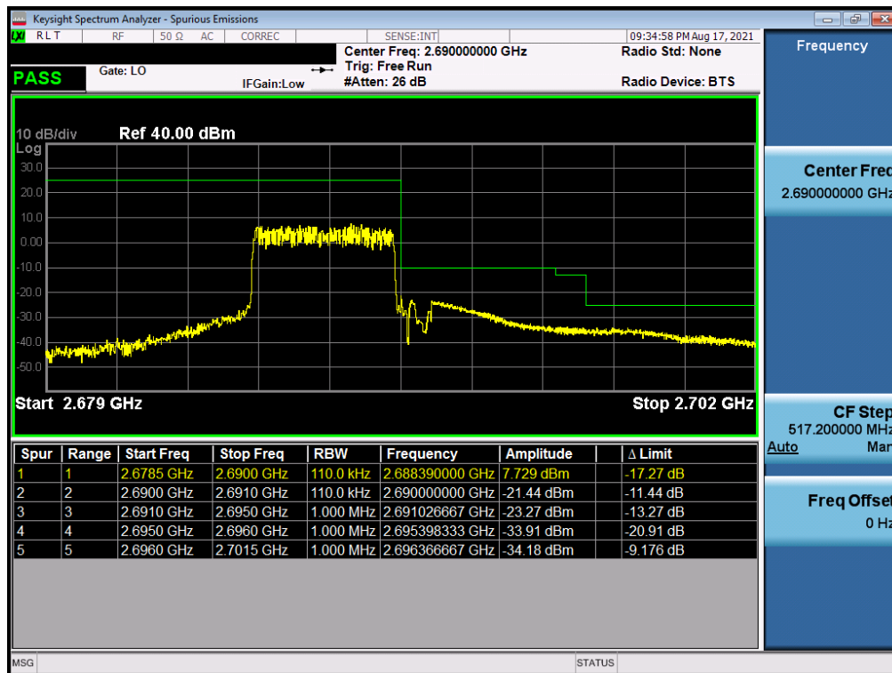
Plot 7-44. Upper ACP Plot (LTE Band 41 - 5MHz QPSK – Full RB)
