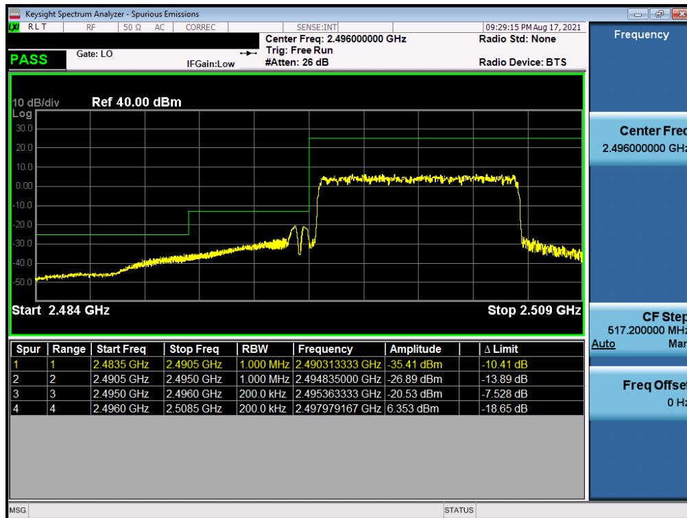
Plot 7-45. Lower ACP Plot (LTE Band 41 - 10MHz QPSK – Full RB)
