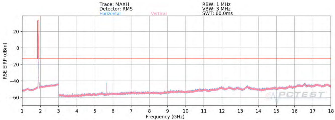
Plot 7-109. Radiated Spurious Plot (LTE Band 25/2)
