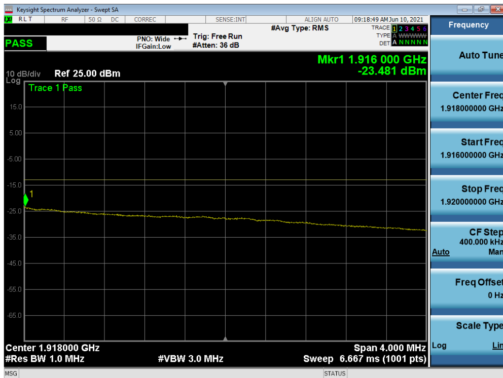
Plot 7-51. Extended Upper Band Edge Plot (LTE Band 25 – 15MHz QPSK – Full RB Configuration)
