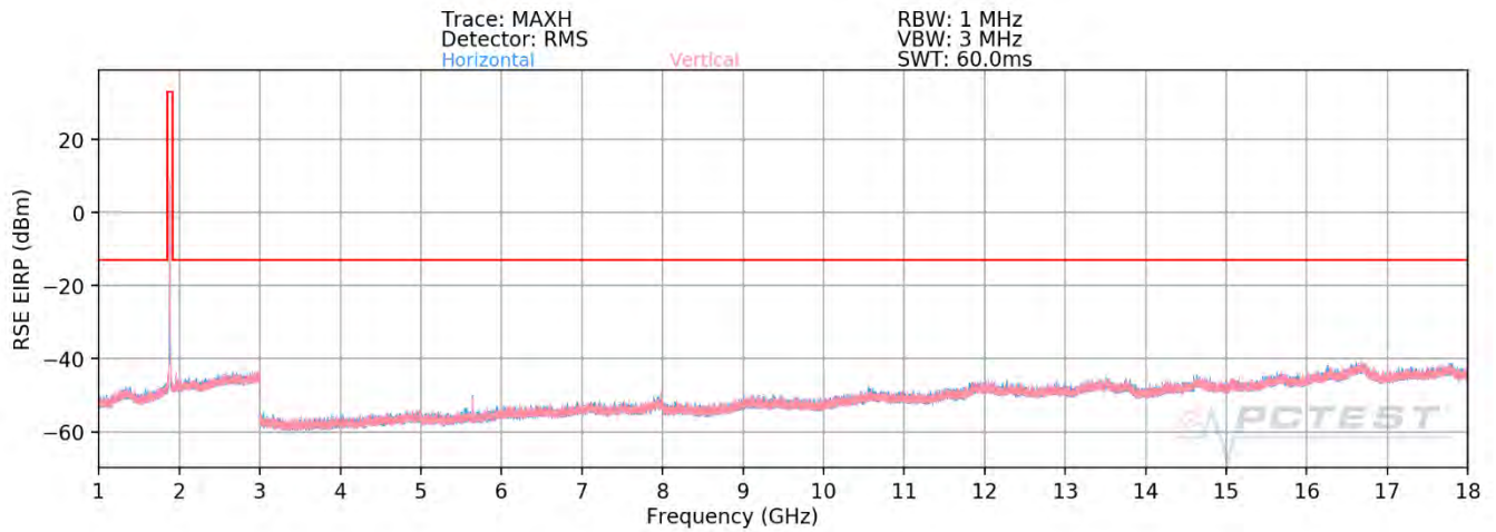
Plot 7-110. Radiated Spurious Plot (WCDMA PCS)
