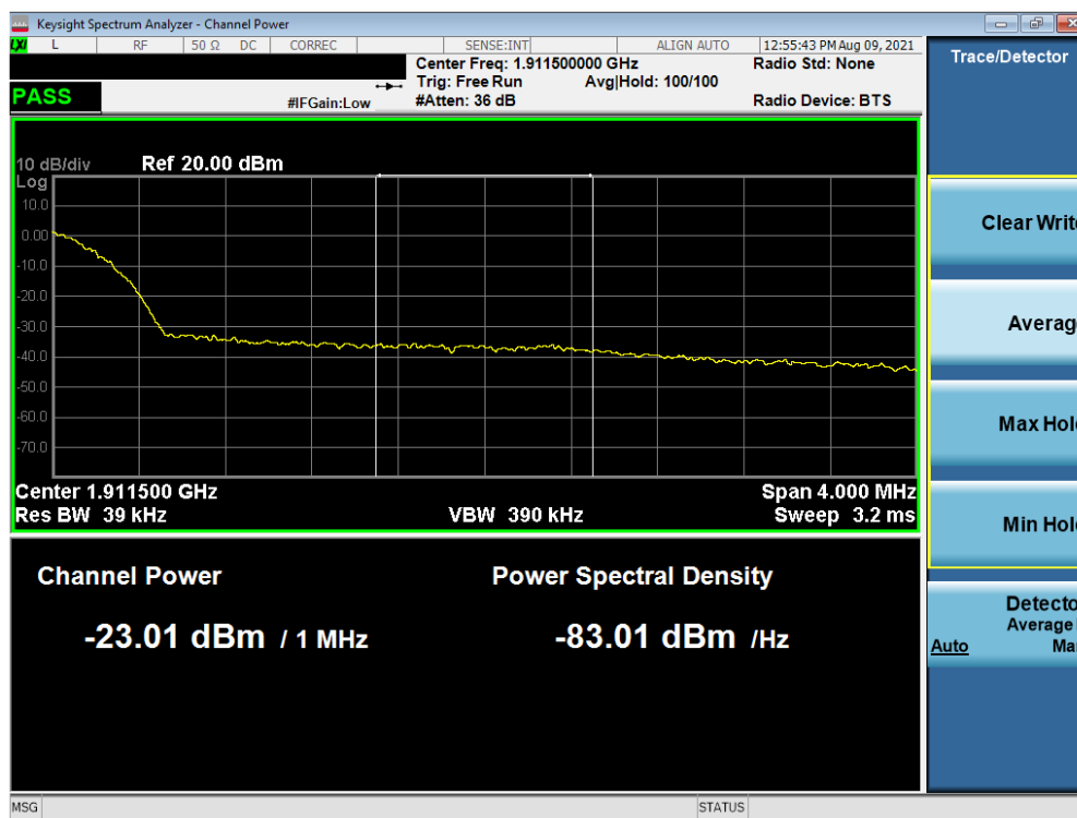
Plot 7-83. Extended Upper Band Edge Plot (WCDMA PCS – Ch. 9538)
