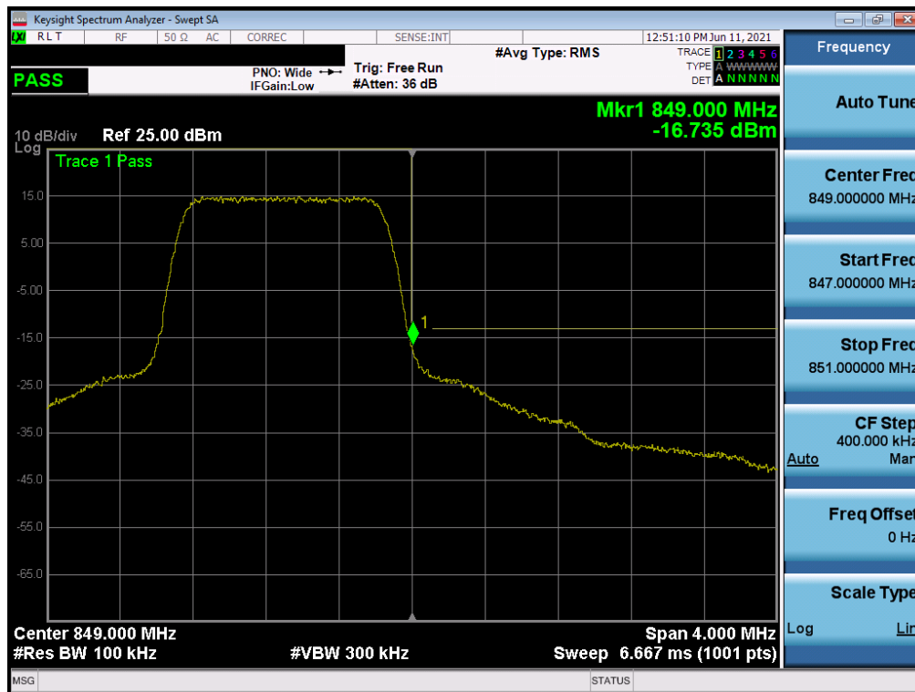
Plot 7-37. Upper BE Plot (LTE Band 5 – 1.4MHz QPSK – Full RB Configuration)
