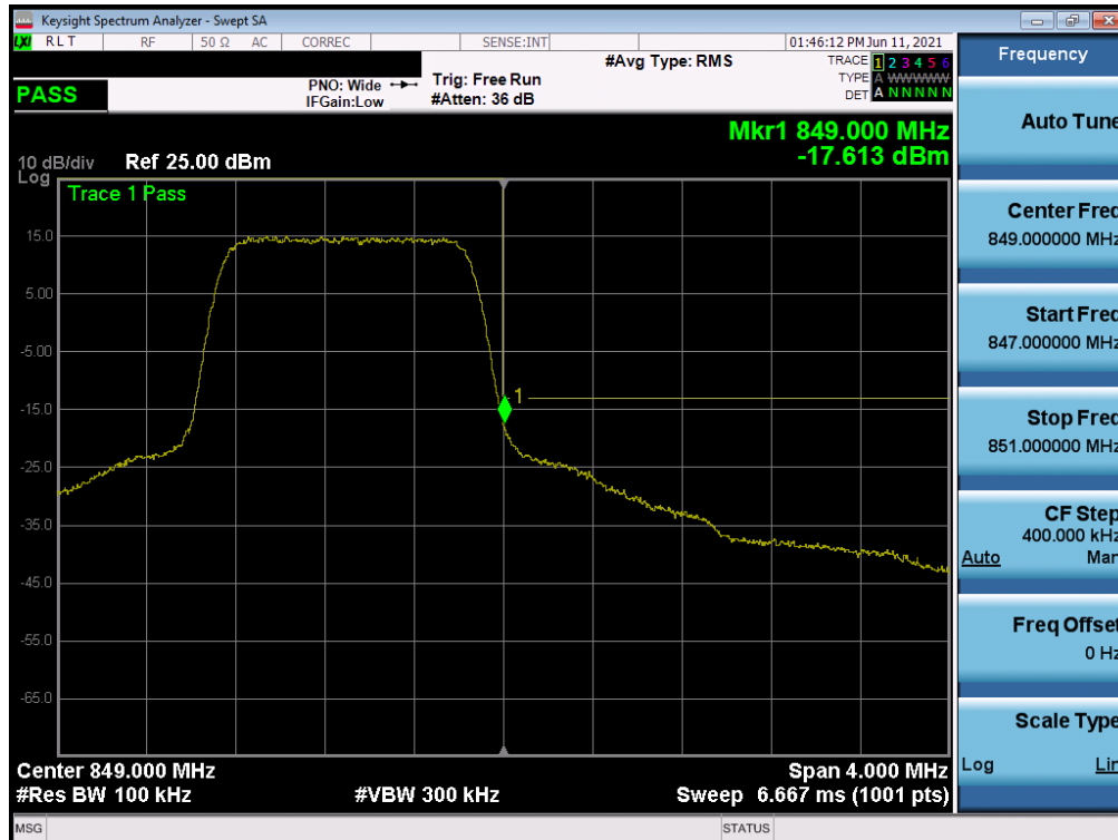
Plot 7-29. Upper BE Plot (LTE Band 26 – 1.4MHz QPSK – Full RB Configuration)
