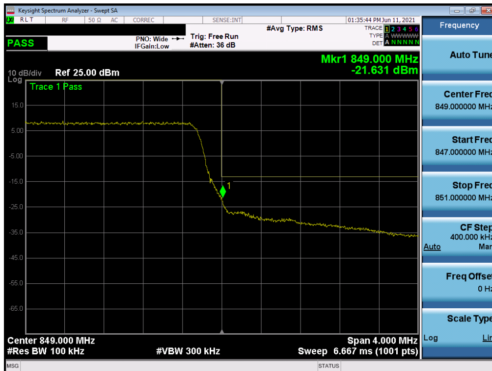
Plot 7-33. Upper BE Plot (LTE Band 26 - 5MHz QPSK – Full RB Configuration)
