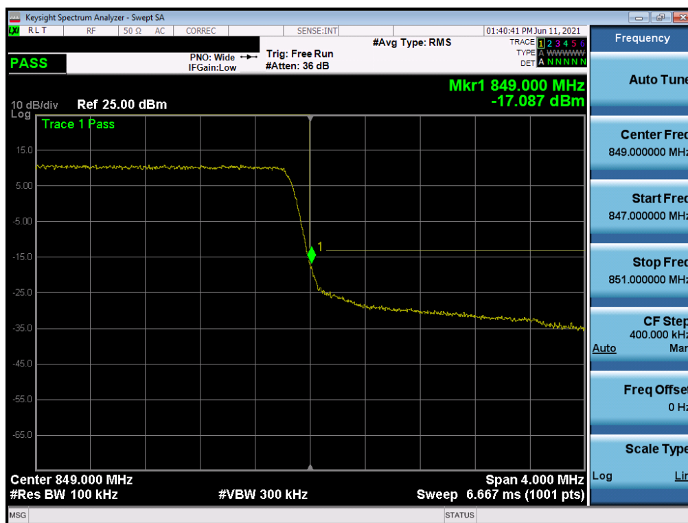
Plot 7-31. Upper BE Plot (LTE Band 26 - 3MHz QPSK – Full RB Configuration)
