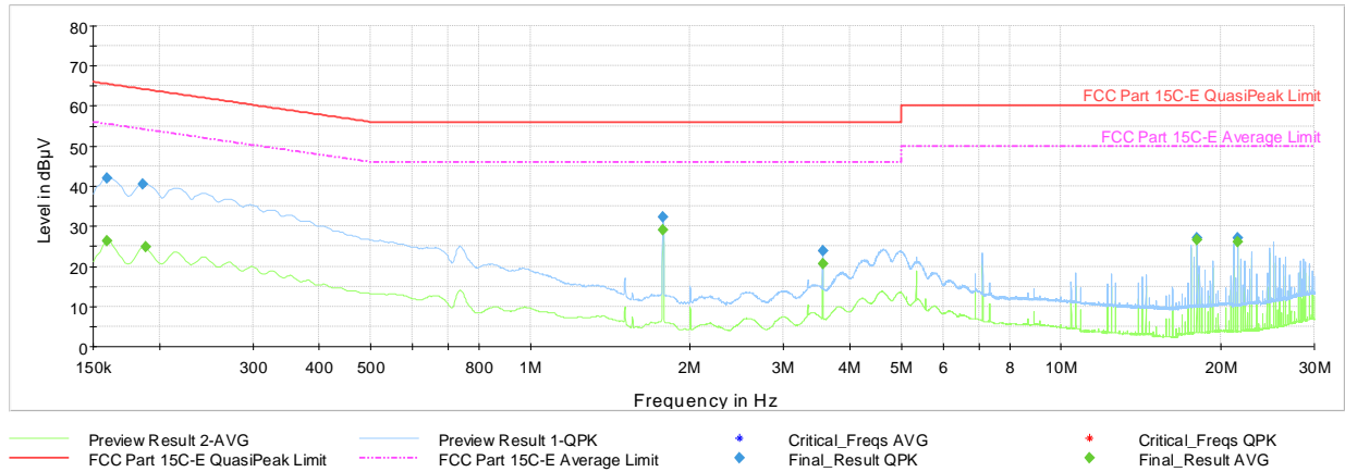
Plot 7-39. AC Line Conducted Emissions with Bluetooth LE (1Mbps, ePA – Ch.39, L1, with AC/DC Adapter + Magnetic Charger)
