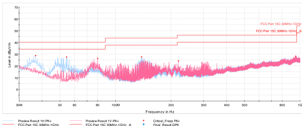
Plot 7-38. Radiated Spurious Emissions Below 1GHz (1Mbps, ePA – Ch.39, Pol. H & V, with AC/DC Adapter + Magnetic Charger)
