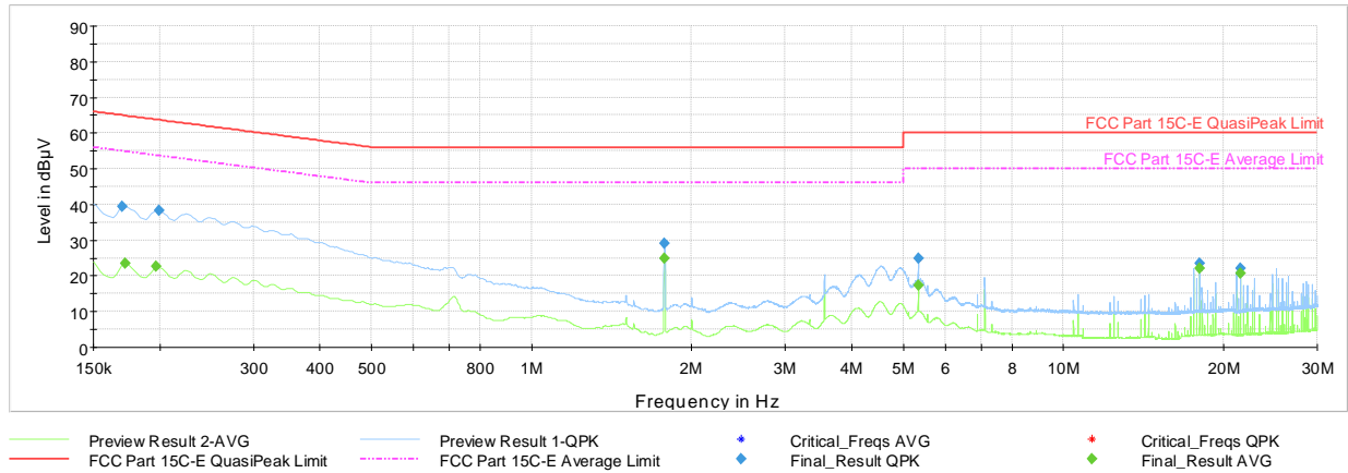
Plot 7-40. AC Line Conducted Emissions with Bluetooth LE (1Mbps, ePA – Ch.39, N, with AC/DC Adapter + Magnetic Charger)
