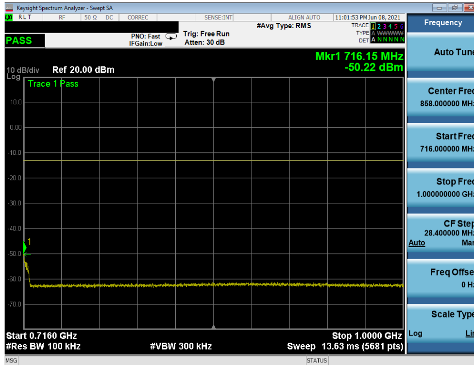
Plot 7-39. CSE Plot (LTE Band 12/17 - 10MHz QPSK - RB Size 1, RB Offset 0 - Mid Channel)
