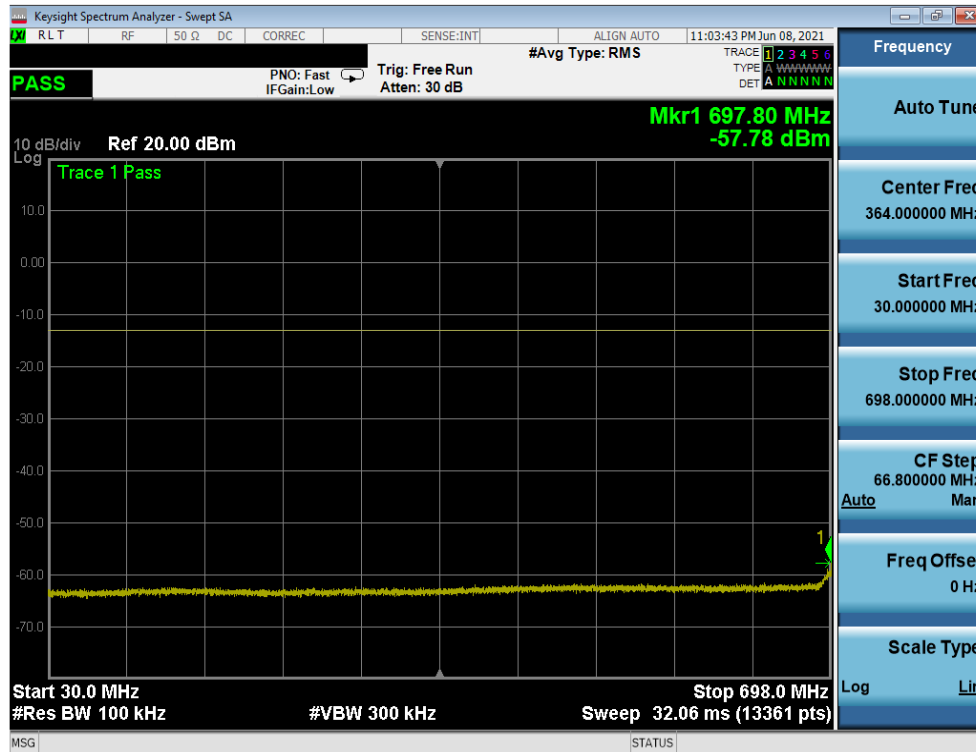
Plot 7-41. CSE (LTE Band 12/17 - 10MHz QPSK - RB Size 1, RB Offset 0 - High Channel)
