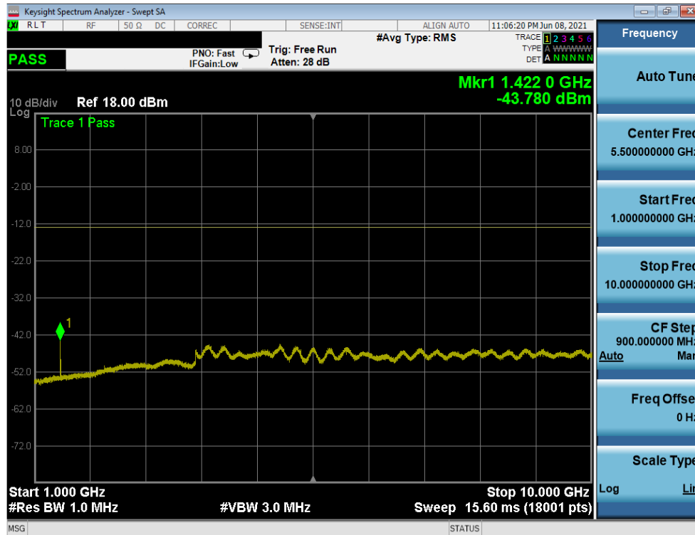
Plot 7-43. CSE (LTE Band 12/17 - 10MHz QPSK - RB Size 1, RB Offset 0 - High Channel)
