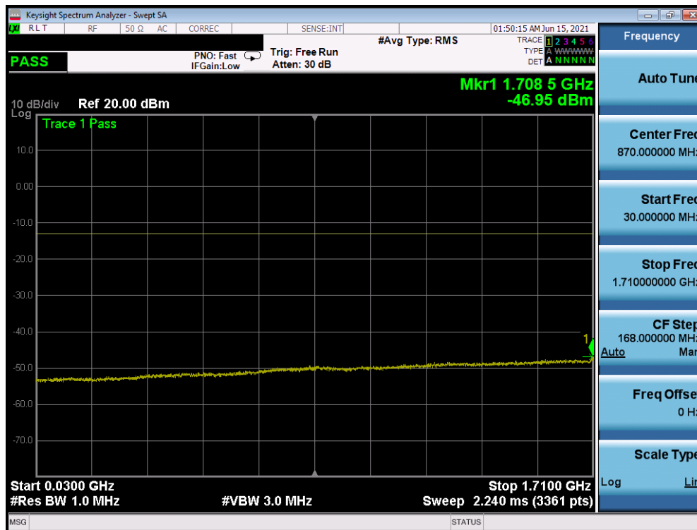
Plot 7-50. CSE (WCDMA Ch. 1413- Mid Channel)
