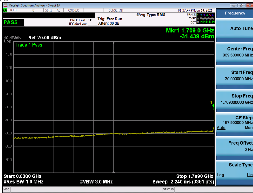
Plot 7-26. CSE (LTE Band 66/4 - 20MHz QPSK - RB Size 1, RB Offset 0 - Low Channel)
