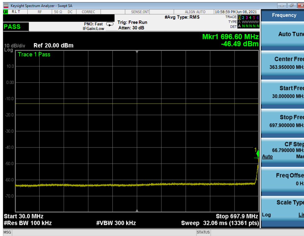
Plot 7-35. CSE (LTE Band 12/17 - 10MHz QPSK - RB Size 1, RB Offset 0 - Low Channel)
