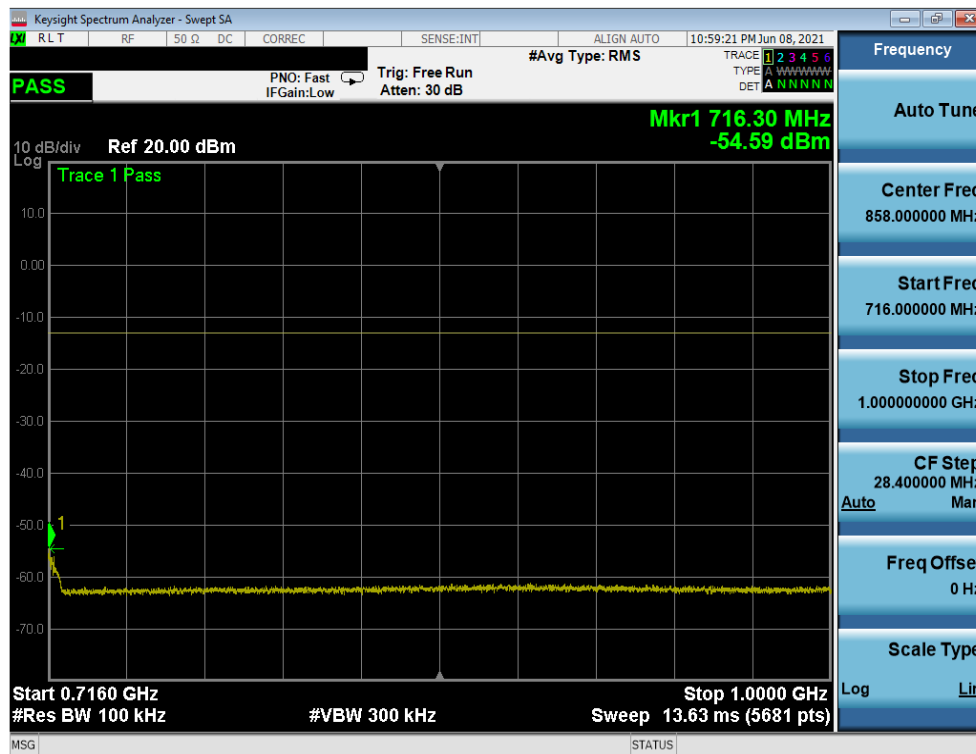
Plot 7-36. CSE (LTE Band 12/17 - 10MHz QPSK - RB Size 1, RB Offset 0 - Low Channel)
