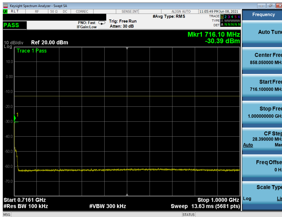
Plot 7-42. CSE (LTE Band 12/17 - 10MHz QPSK - RB Size 1, RB Offset 0 - High Channel)
