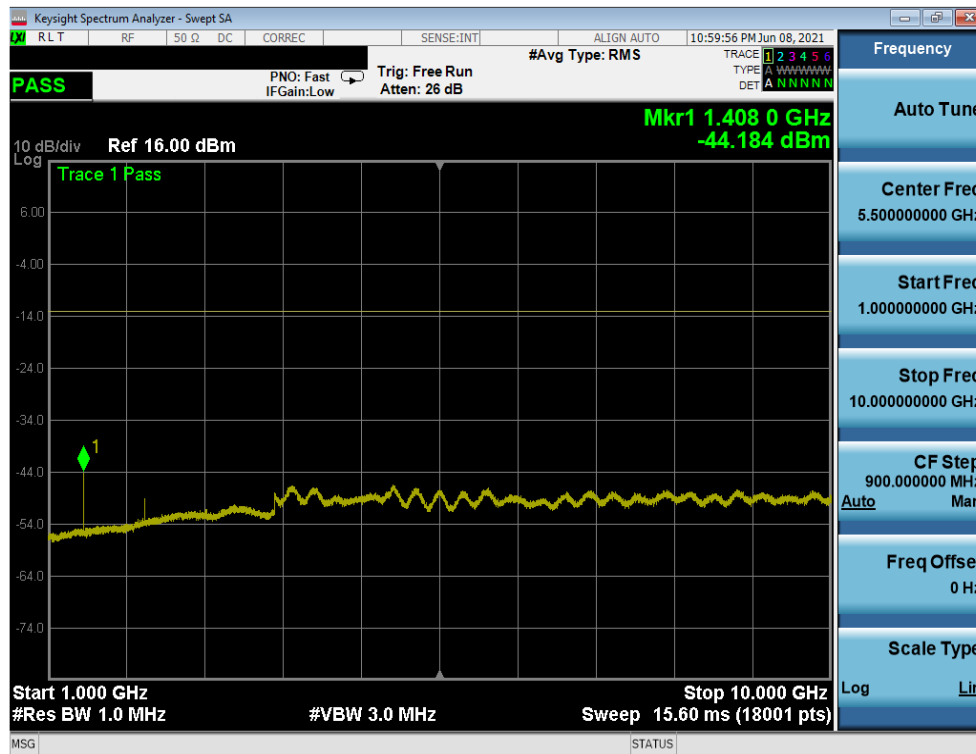
Plot 7-37. CSE (LTE Band 12/17 - 10MHz QPSK - RB Size 1, RB Offset 0 - Low Channel)
