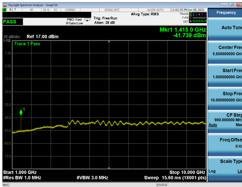
Plot 7-40. CSE (LTE Band 12/17 - 10MHz QPSK - RB Size 1, RB Offset 0 - Mid Channel)
