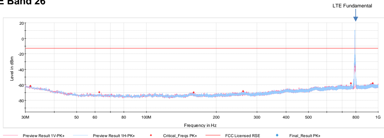
Plot 7-46. Antenna BCM Radiated Spurious Plot below 1GHz (LTE Band 26)
