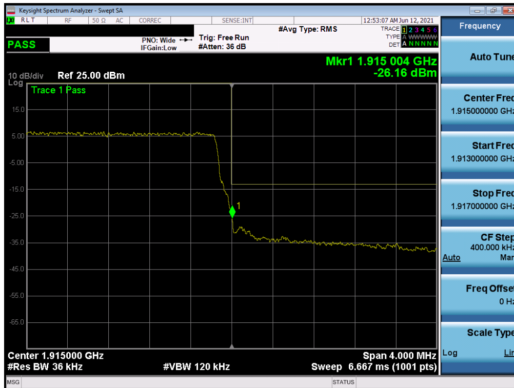
Plot 7-62. Upper Band Edge Plot (LTE Band 25 – 3MHz QPSK – Full RB Configuration)
