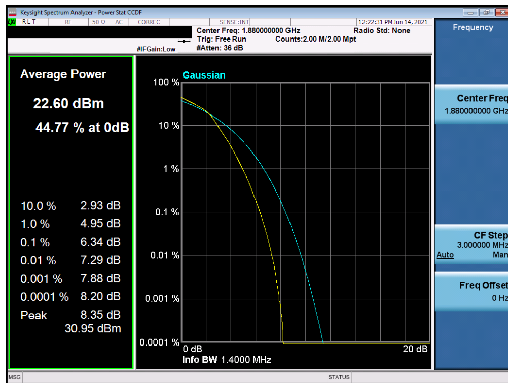
Plot 7-85. PAR Plot (LTE Band 2 - 1.4MHz 16-QAM - Full RB Configuration)
