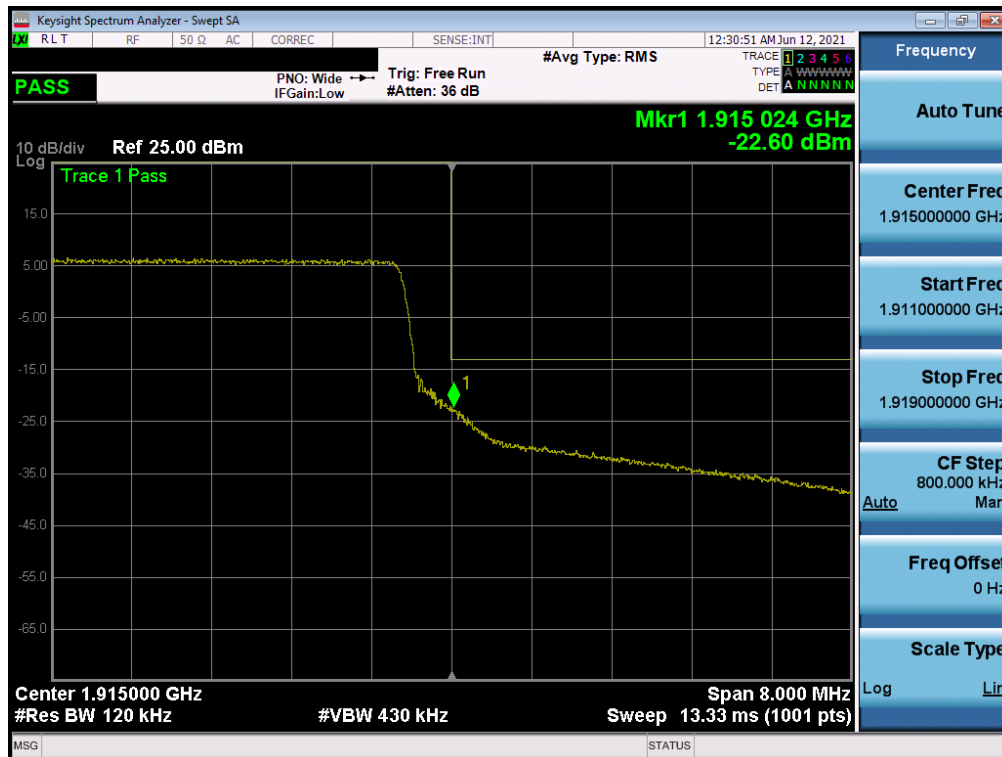
Plot 7-70. Upper Band Edge Plot (LTE Band 25 – 10MHz QPSK – Full RB Configuration)
