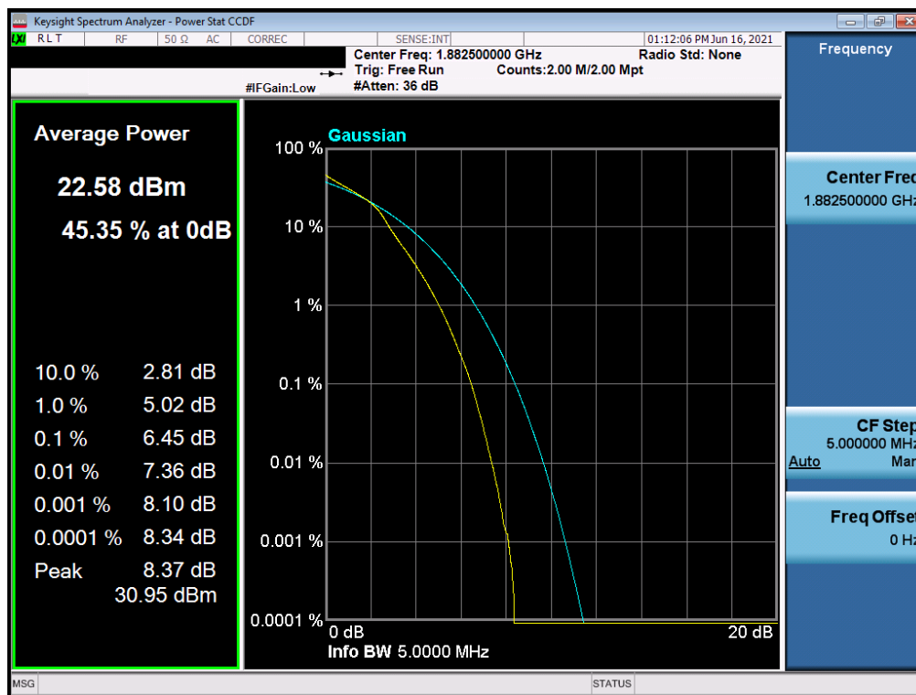
Plot 7-101. PAR Plot (LTE Band 25 - 5MHz 16-QAM - Full RB Configuration)
