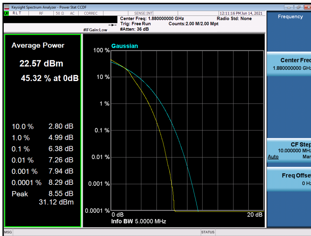
Plot 7-89. PAR Plot (LTE Band 2 - 5MHz 16-QAM - Full RB Configuration)
