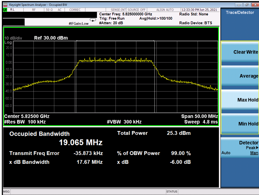
Plot 7-12. 99% OBW and 6dB Bandwidth (20MHz BW 802.11n (UNII Band 3) – Ch. 165)
