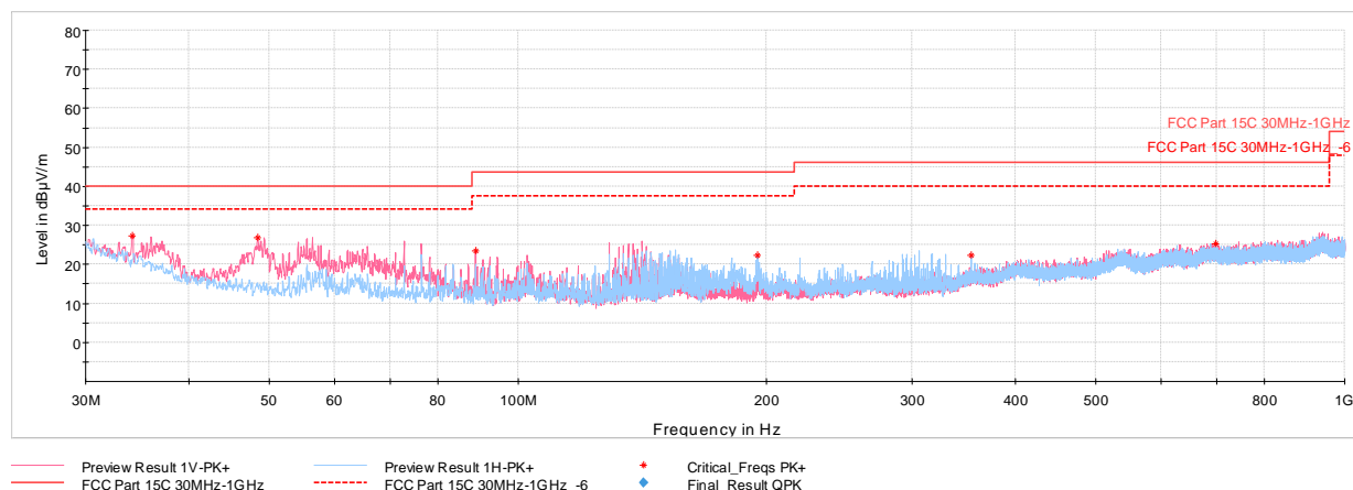
Plot 7-58. Radiated Spurious Emissions below 1GHz (802.11n – UNII 3 Ch. 157) with AC/DC Adaptor & Magnetic Charger
