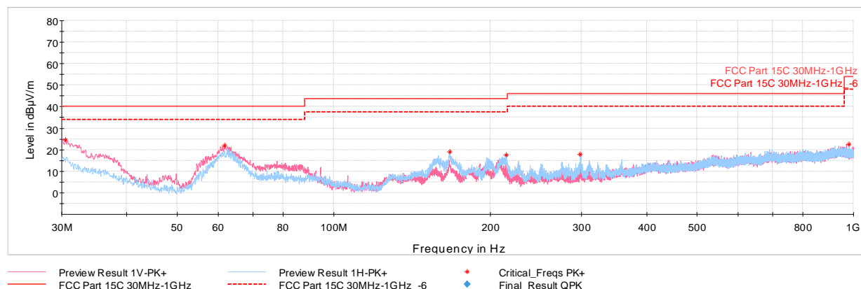
Plot 7-59. Radiated Spurious Emissions – Simultaneous Transmission below 1GHz with AC/DC Adaptor & Magnetic Charger
