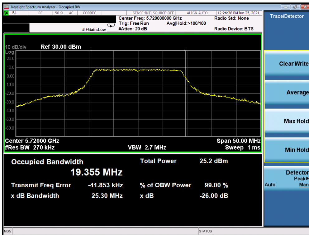
Plot 7-9. 99% OBW and 26dB Bandwidth (20MHz BW 802.11n (UNII Band 2C) – Ch. 144)
