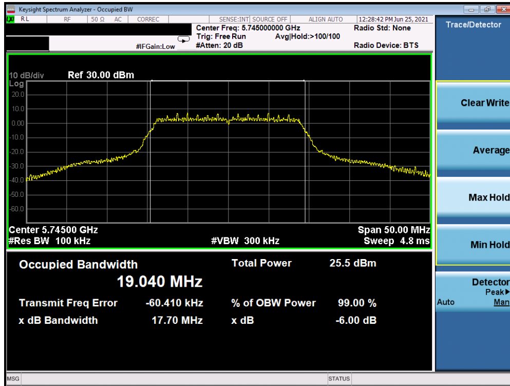
Plot 7-10. 99% OBW and 6dB Bandwidth (20MHz BW 802.11n (UNII Band 3) – Ch. 149)
