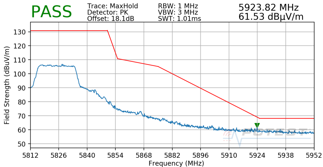
Plot 7-57. Radiated Upper Band Edge Plot (Peak - UNII Band 3)
