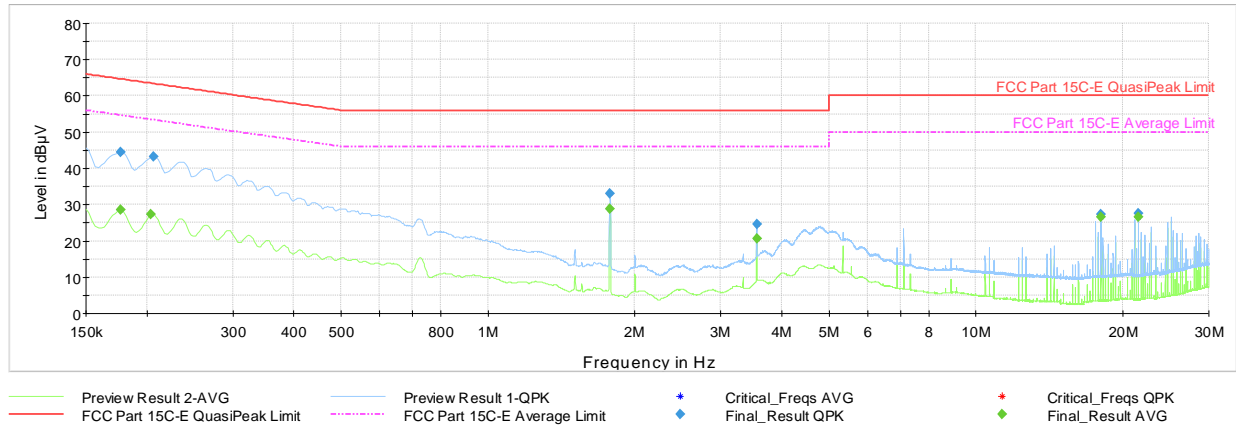
Plot 7-60. AC Line Conducted Plot with 802.11n UNII Band 3 – Ch.157 (L1) with AC/DC Adaptor & Magnetic Charger
