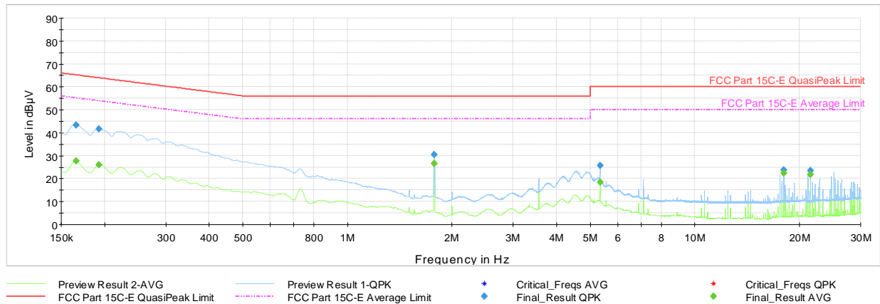
Plot 7-61. AC Line Conducted Plot with 802.11n UNII Band 3 – Ch.157 (N) with AC/DC Adaptor & Magnetic Charger
