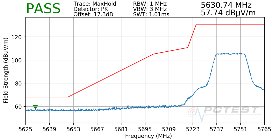
Plot 7-54. Radiated Lower Band Edge Plot (Peak – UNII Band 3)
