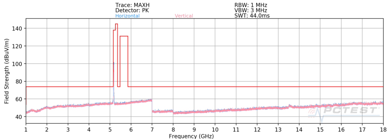
Plot 7-25. Radiated Spurious Emissions above 1GHz (802.11n – UNII 1 Ch. 36)
