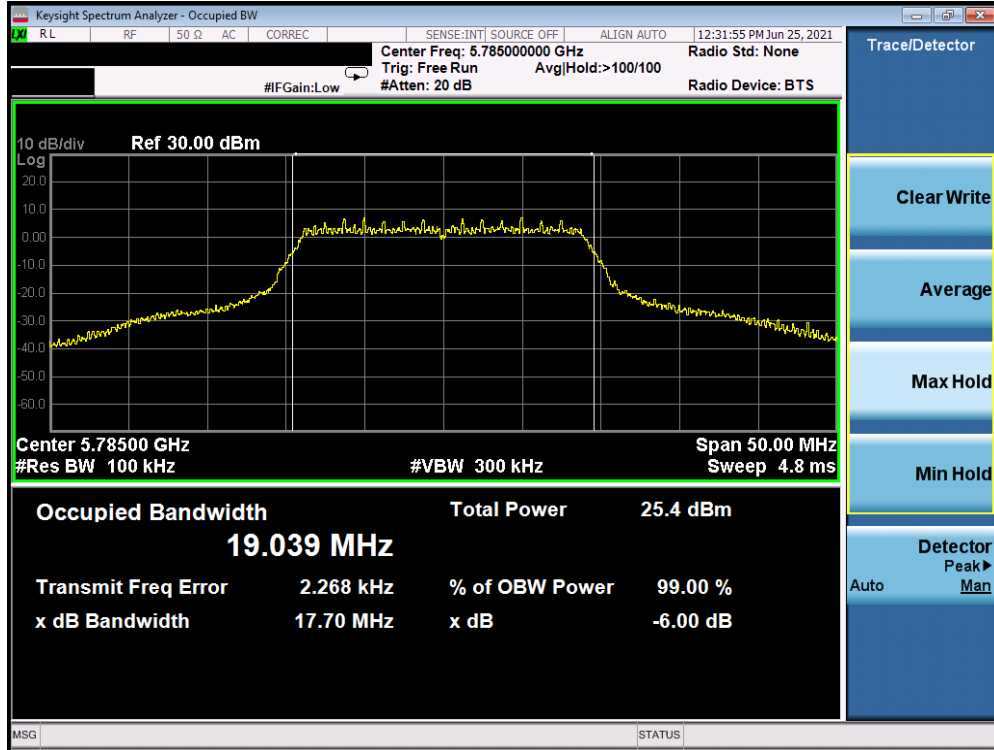
Plot 7-11. 99% OBW and 6dB Bandwidth (20MHz BW 802.11n (UNII Band 3) – Ch. 157)
