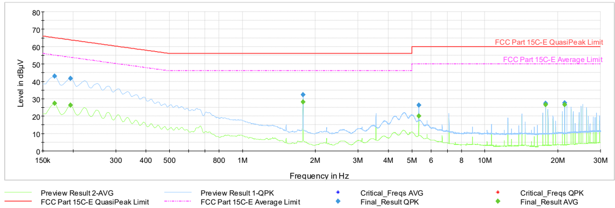
Plot 7-79.AC Line Conducted Plot 802.11b – Ch.6 (L1), with AC/DC Adapter and Magnetic Charger
