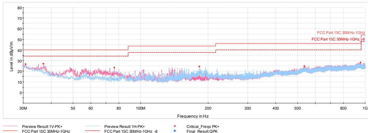
Plot 7-78. Radiated Spurious Emissions 30MHz-1GHz 802.11b – Ch.6, with AC/DC Adapter and Magnetic Charger
