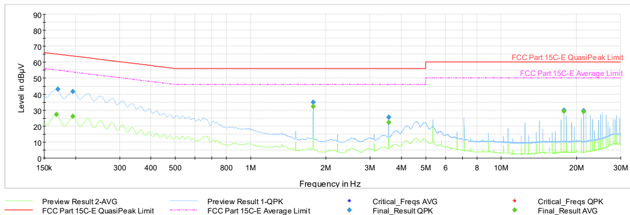
Plot 7-80.AC Line Conducted Plot 802.11b – Ch.6 (N), with AC/DC Adapter and Magnetic Charger
