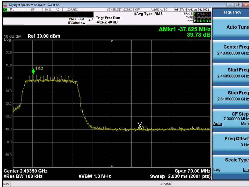
Plot 7-42. Band Edge Plot (802.11n MCS0 – Ch. 11)
