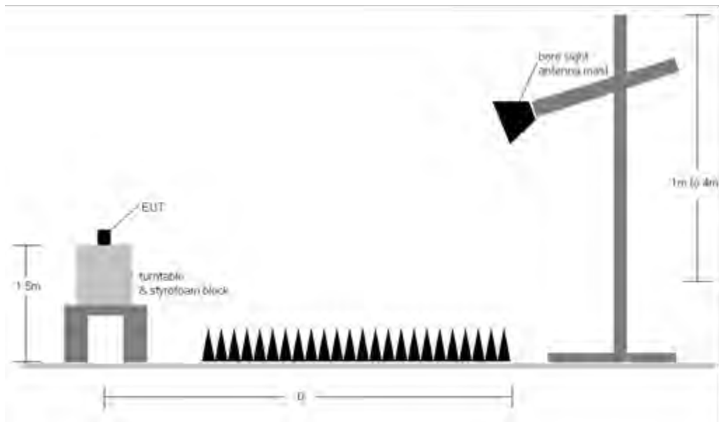
Figure 7-6. Radiated Measurement Setup
