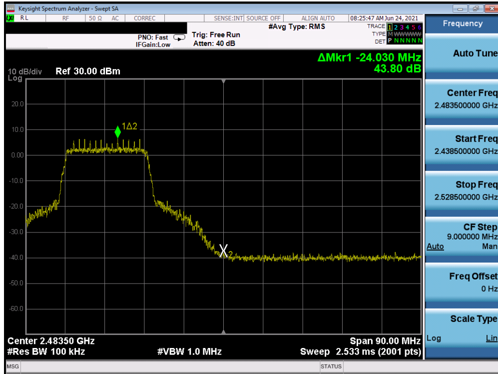
Plot 7-41. Band Edge Plot (802.11n MCS0 – Ch. 10)
