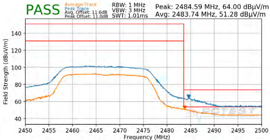
Plot 7-76. Radiated Restricted Upper Band Edge Measurement
